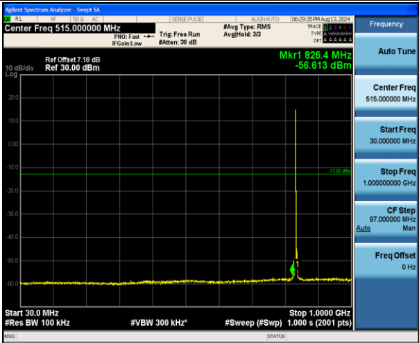
Band5_3MHz_16QAM_20525_1RB#0_30~1000_30~1000
