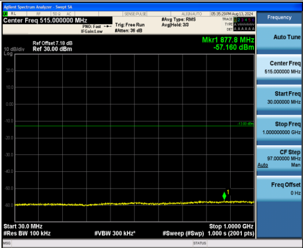
Band4_15MHz_QPSK_20025_1RB#0_30~1000_30~1000
