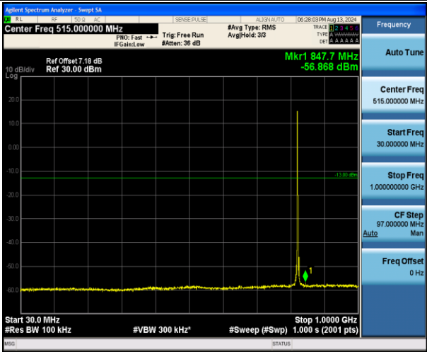
Band5_3MHz_QPSK_20415_1RB#0_30~1000_30~1000
