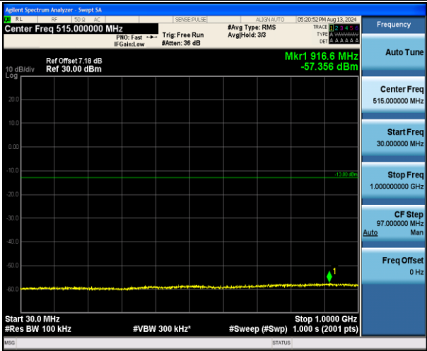
Band4_10MHz_16QAM_20175_1RB#0_30~1000_30~1000
