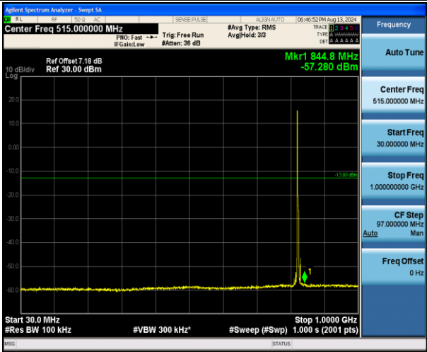
Band5_5MHz_QPSK_20425_1RB#0_30~1000_30~1000
