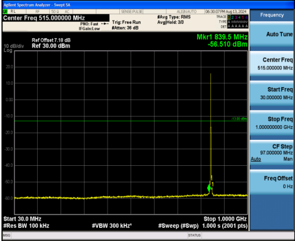
Band5_3MHz_QPSK_20635_1RB#0_30~1000_30~1000
