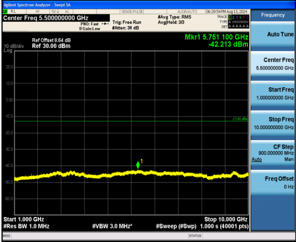
Band5_3MHz_16QAM_20525_1RB#0_1000~10000_1000~10000
