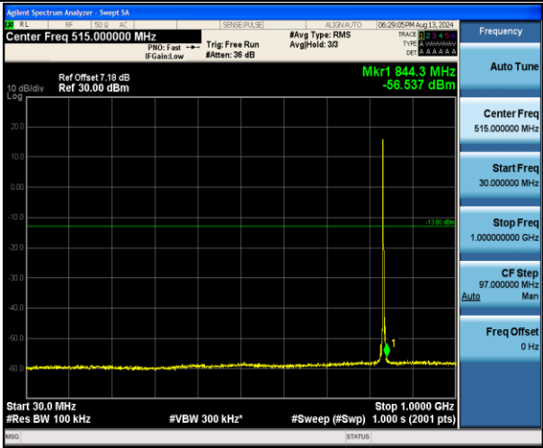
Band5_3MHz_QPSK_20525_1RB#0_30~1000_30~1000
