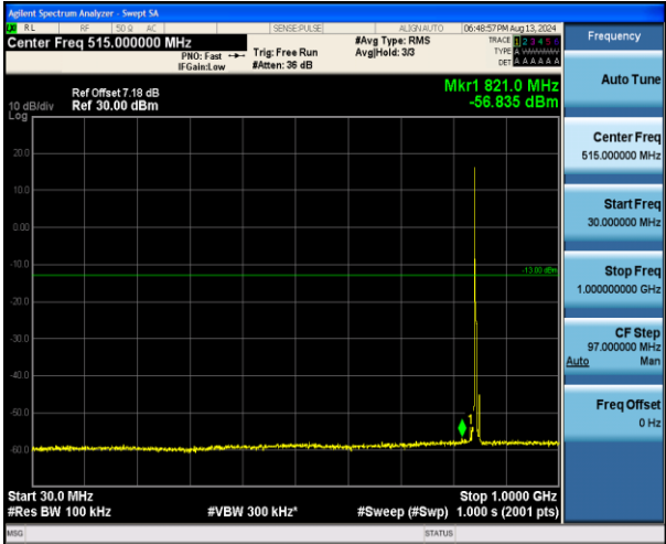
Band5_5MHz_QPSK_20625_1RB#0_30~1000_30~1000
