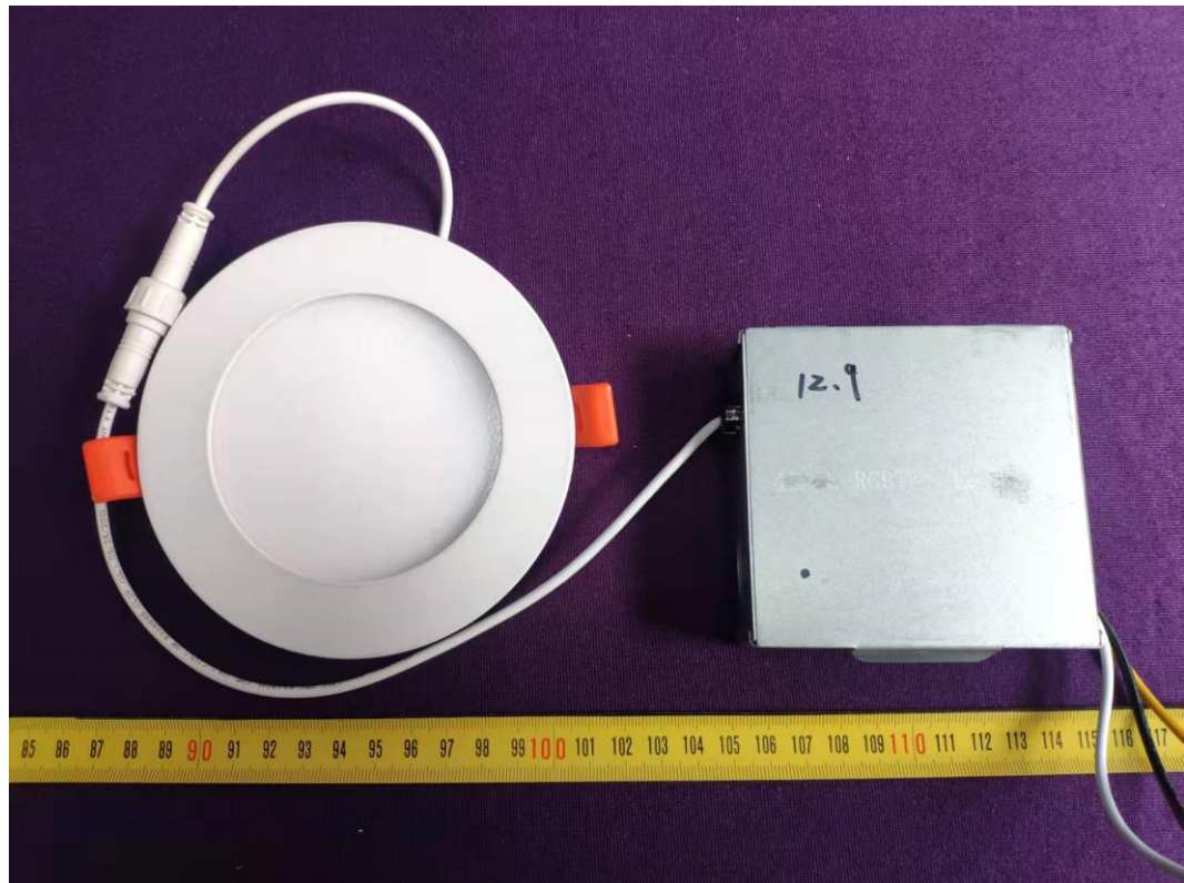
FIGURE 2 CYNCR FIXTURE CANLESS (M/N: CFXCNLR4S1) LAMP FRONT
