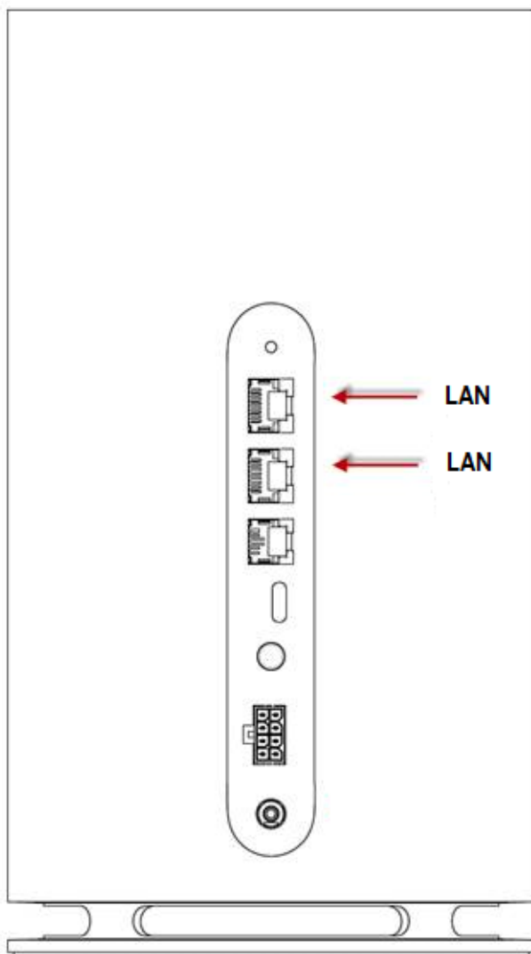
Figure 17 Location of the Gigabit Ethernet LAN ports
