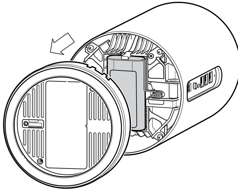
Figure 22 Remove battery
