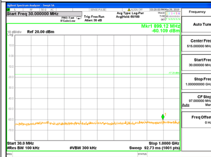
8DPSK on Channel 79
