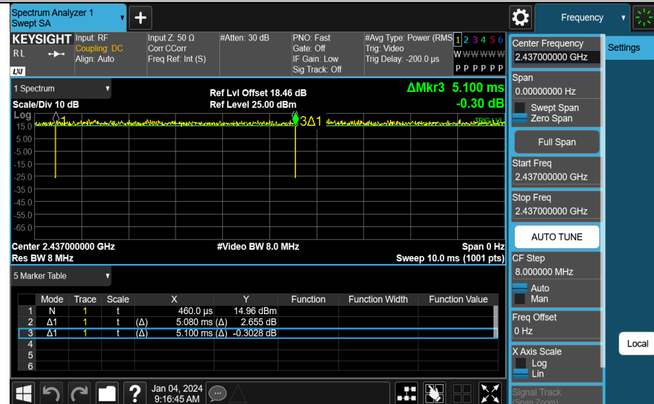
NTNV-11N20SISO-Ant1-2437
