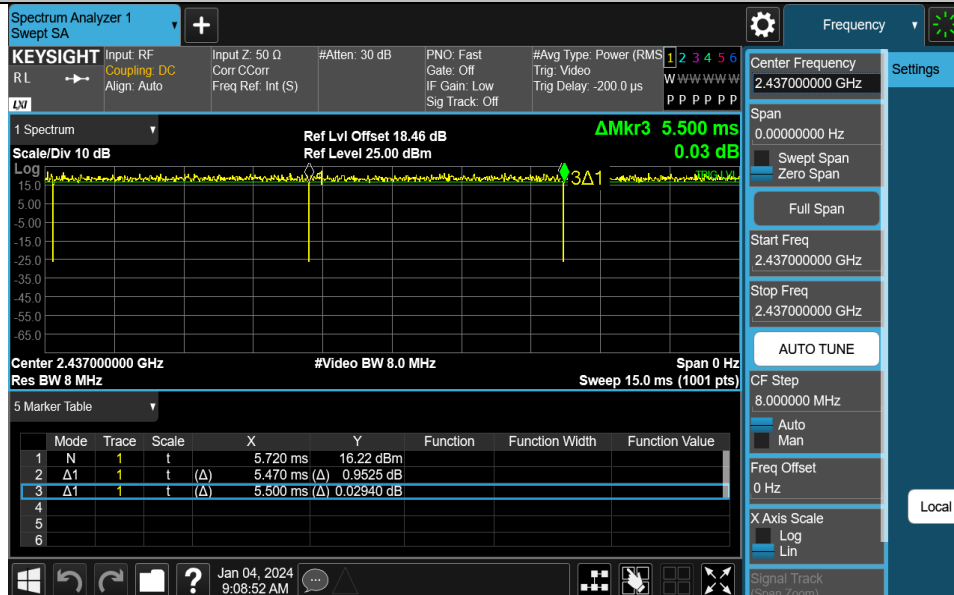
NTNV-11N20SISO-Ant1-2437
