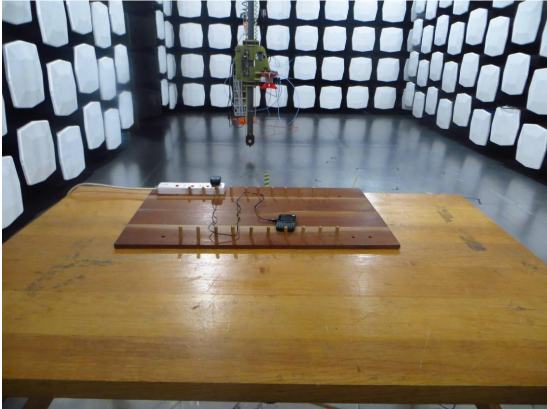
8. Part 15B Radiated emission (USB) below 1GHz
