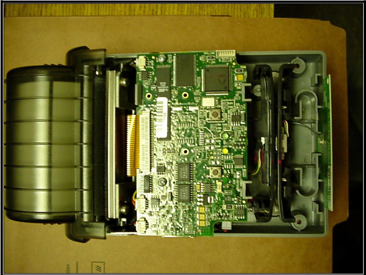
Photograph 6: PCB in Cameo 3 Printer with scanner
