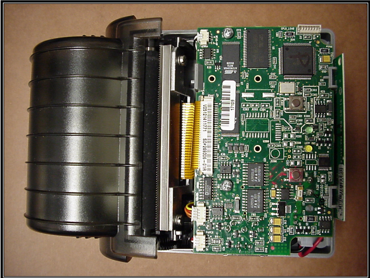
Photograph 5: PCB in Cameo 3 Printer
