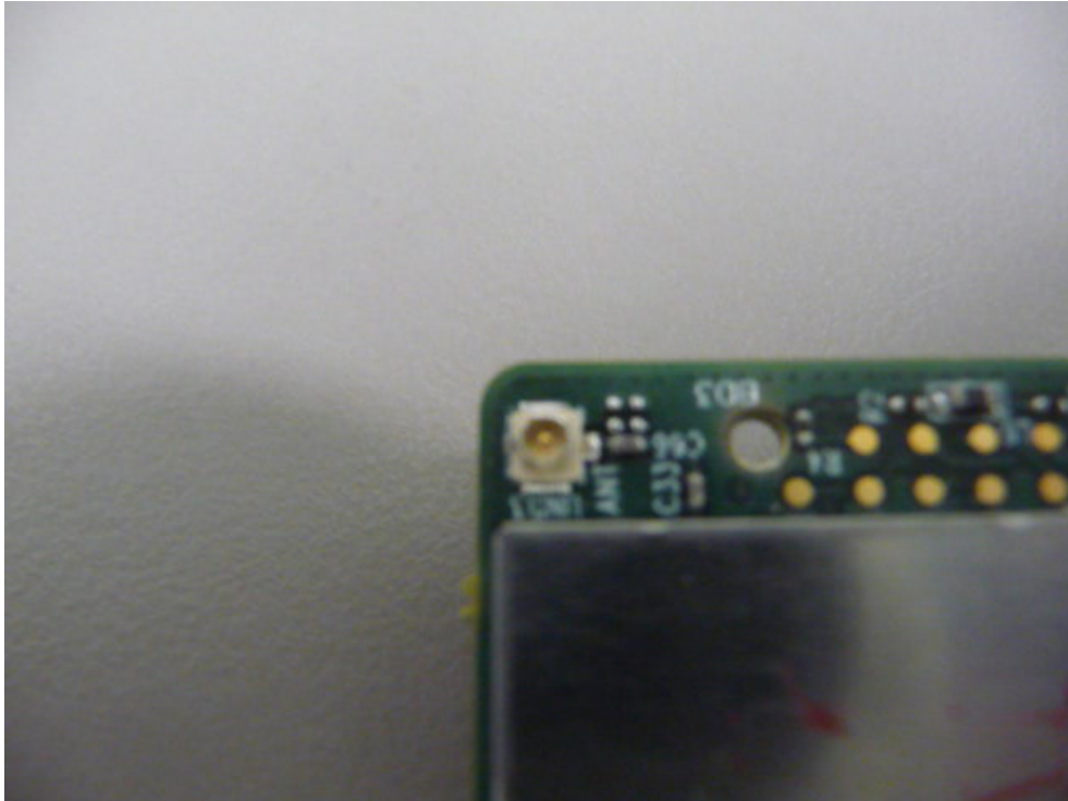
Photograph No.3 Power-G Modem LP Module Antenna connector
