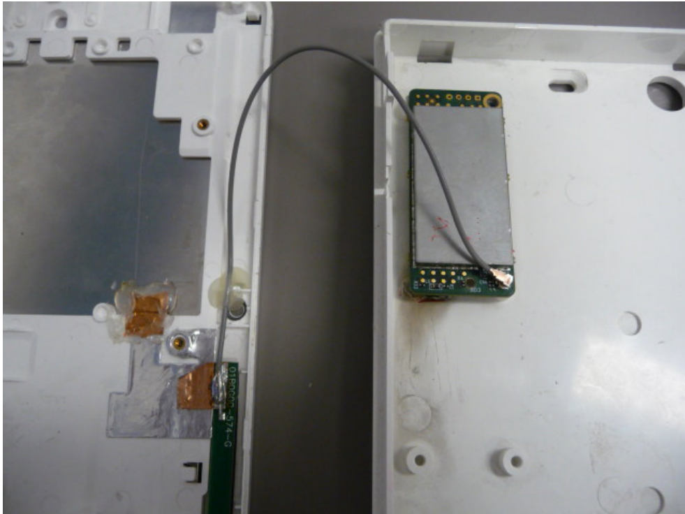
Photograph No.4 Power-G Modem LP Module Antenna assembly
