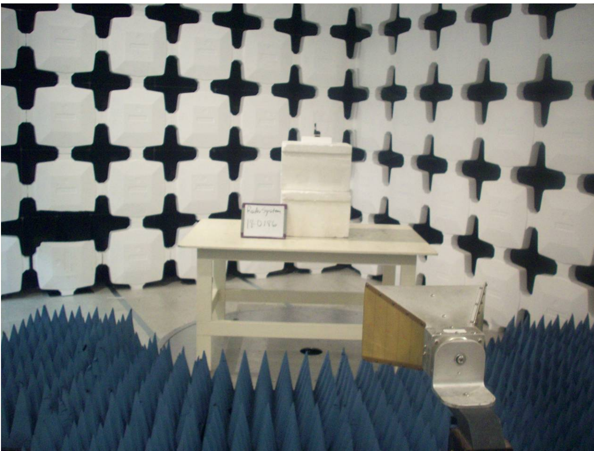
Figure 6. Intentional Radiated Emissions Test Setup, above 1 GHz
