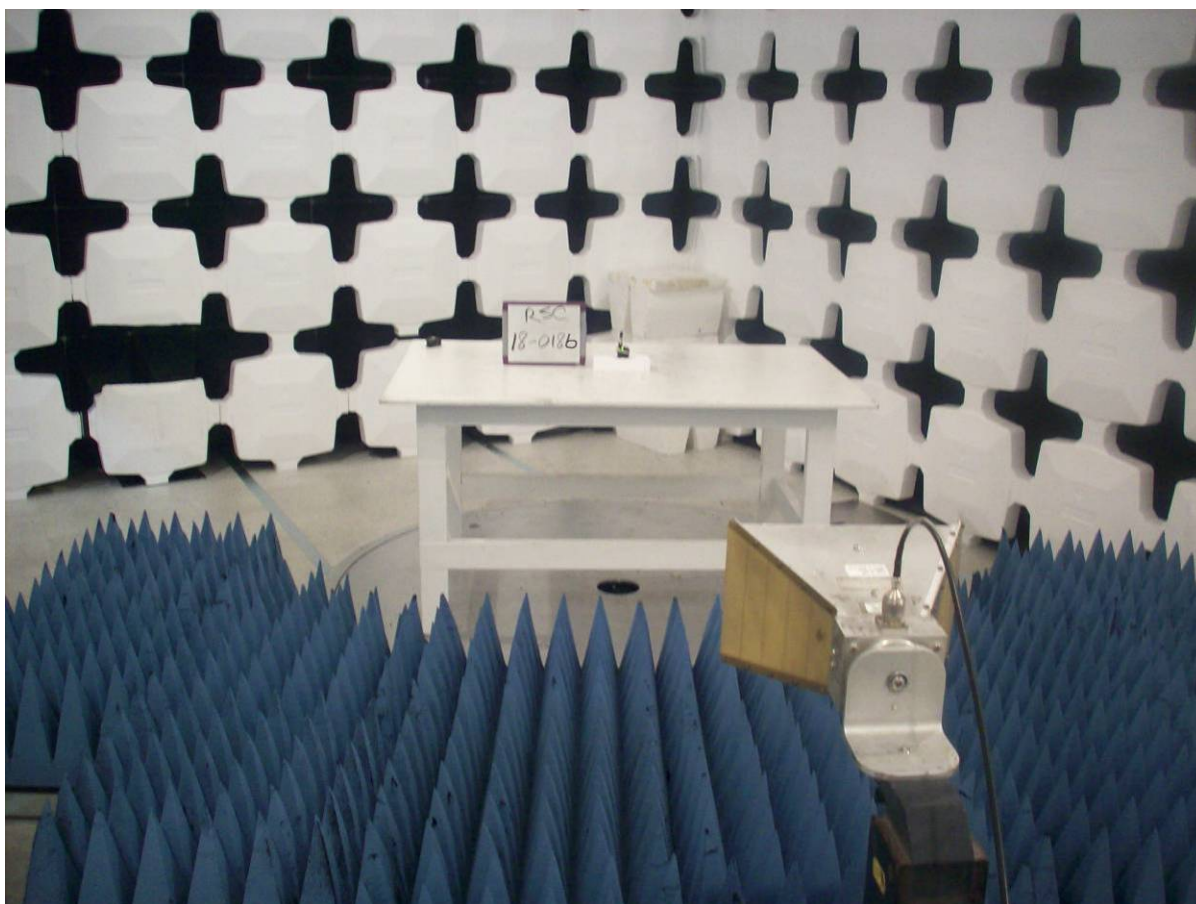
Figure 5. Unintentional Radiated Emissions Test Setup, above 1 GHz
