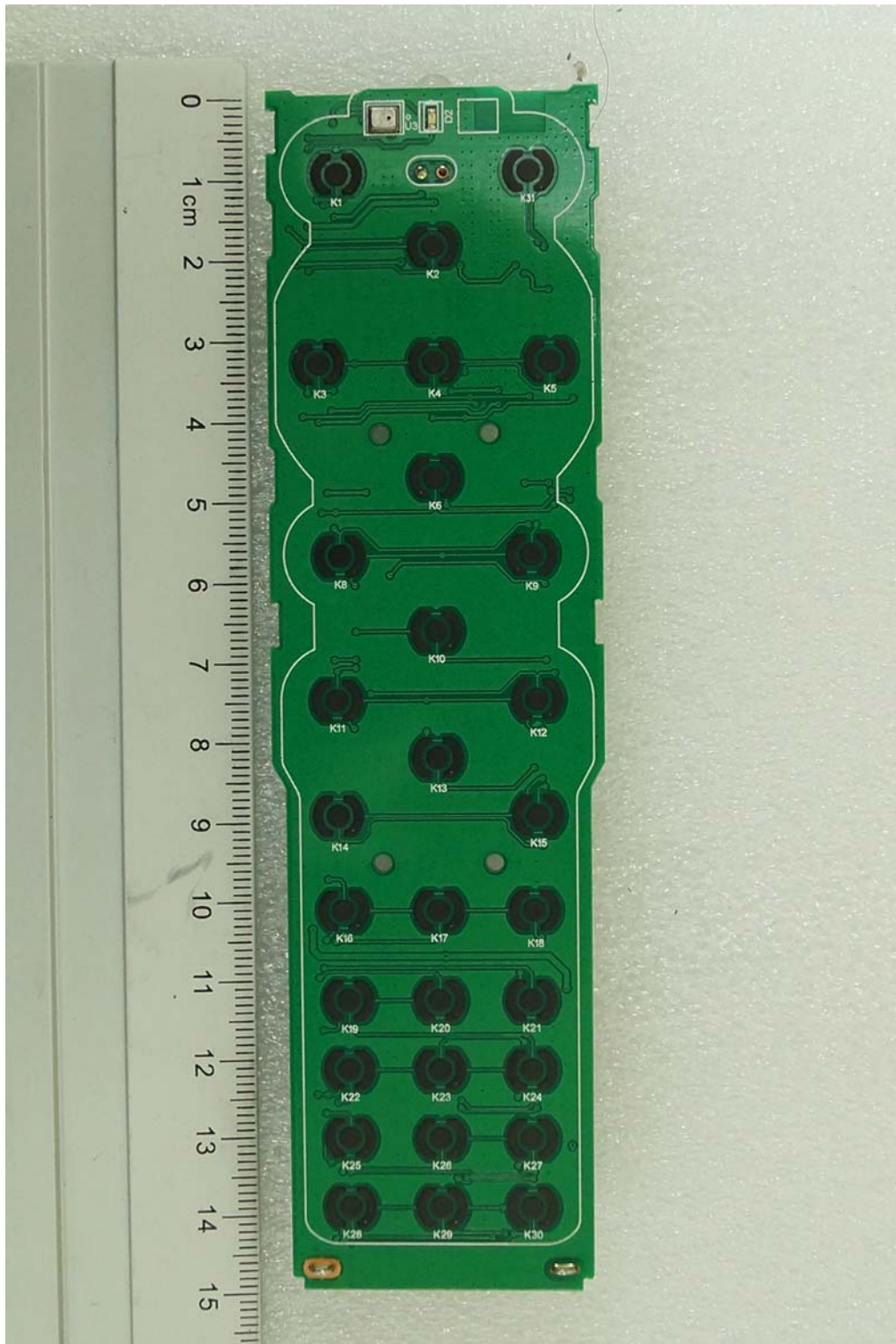
< Main board Top view #2 >
