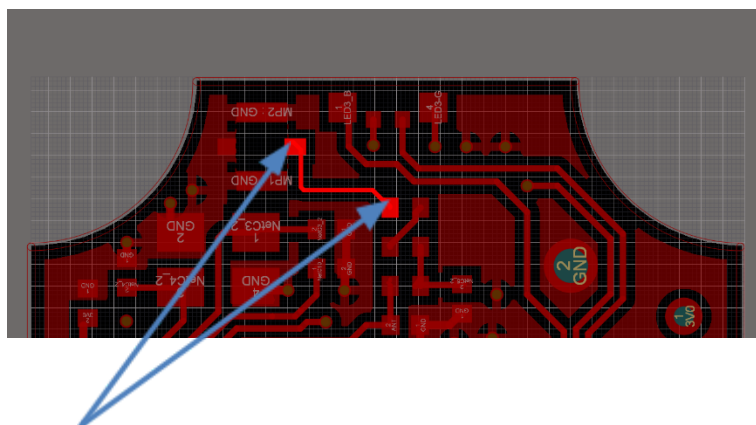
PCB Trace Antenna
