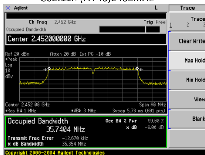
802.11n (HT40)2452MHz
