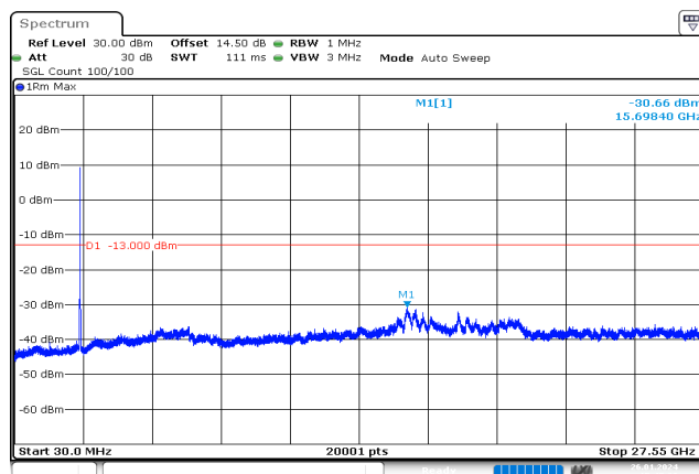
20MHz_High_QPSK_100@0 -30.66 dBm
