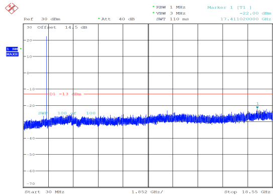
5MHz_Middle_QPSK_1@0 -22.00 dBm
