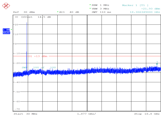
15MHz_Middle_QPSK_1@74 -21.93 dBm
