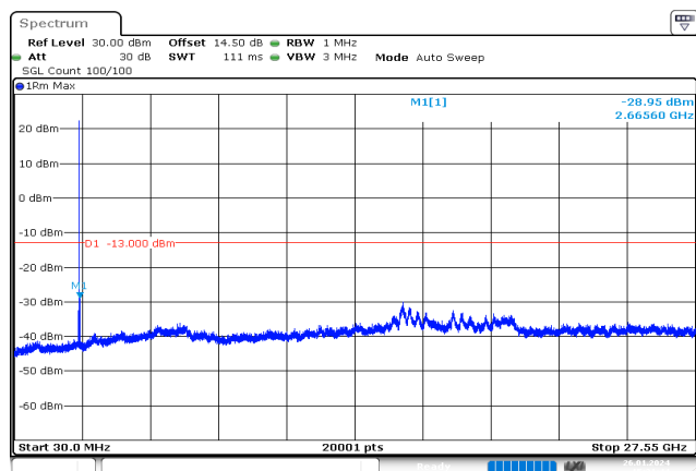
5MHz_High_QPSK_1@0 -28.95 dBm
