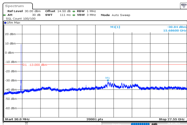
20MHz_Middle_QPSK_100@0 -30.84 dBm
