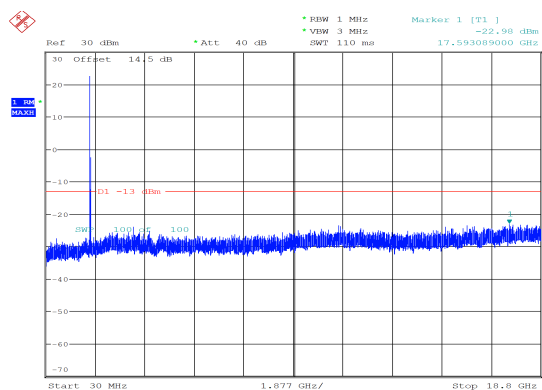
3MHz_Low_QPSK_1@0 -22.98 dBm
