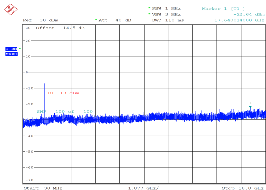
3MHz_Middle_QPSK_1@14 -22.64 dBm
