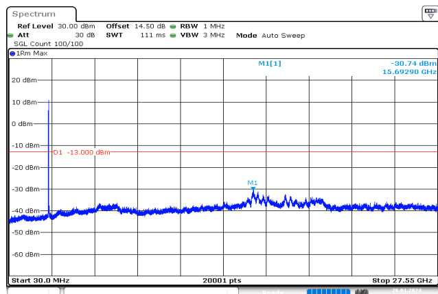
15MHz_Low_QPSK_75@0 -30.74 dBm
