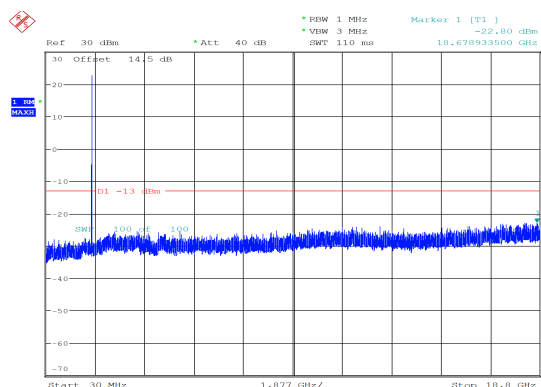
10MHz_High_QPSK_1@49 -22.80 dBm
