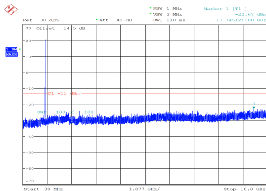
1.4MHz_Middle_QPSK_6@0 -22.67 dBm
