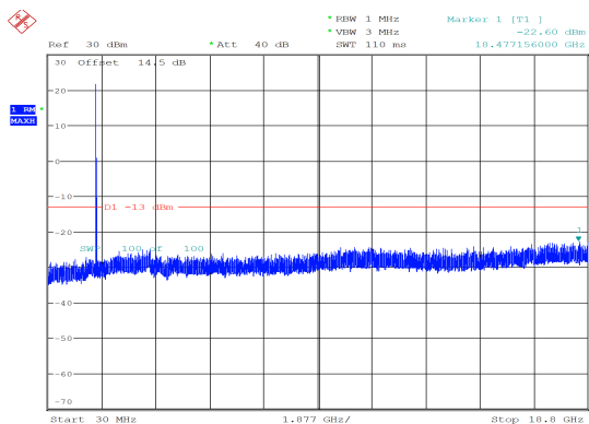
5MHz_Low_QPSK_1@0 -22.60 dBm
