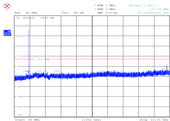
15MHz_Middle_QPSK_75@0 -21.73 dBm
