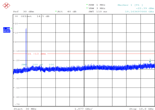
15MHz_Middle_QPSK_75@0 -22.39 dBm
