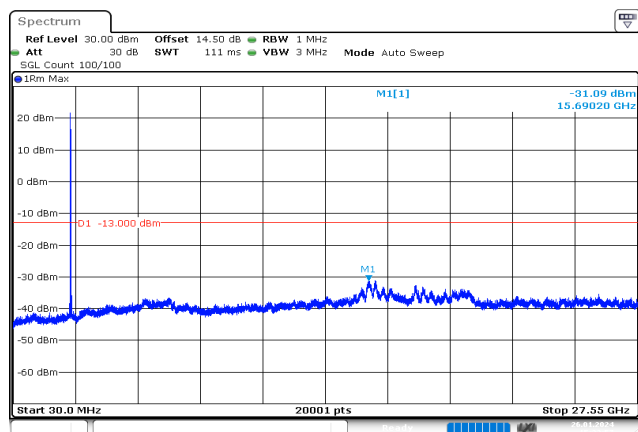
15MHz_Low_QPSK_1@0 -31.09 dBm
