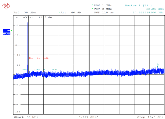
5MHz_High_QPSK_1@0 -22.25 dBm
