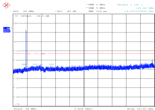
15MHz_Low_QPSK_75@0 -22.42 dBm
