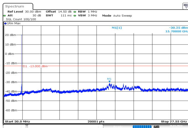
15MHz_High_QPSK_1@74 -30.25 dBm
