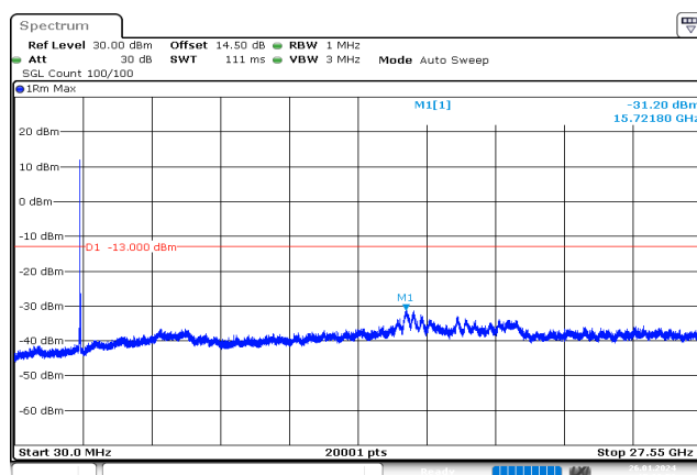
10MHz_High_QPSK_50@0 -31.20 dBm
