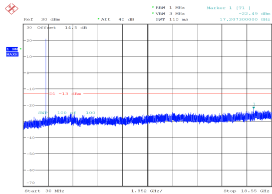
5MHz_Low_QPSK_1@24 -22.49 dBm
