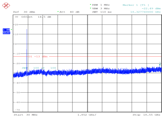
20MHz_Middle_QPSK_100@0 -22.49 dBm
