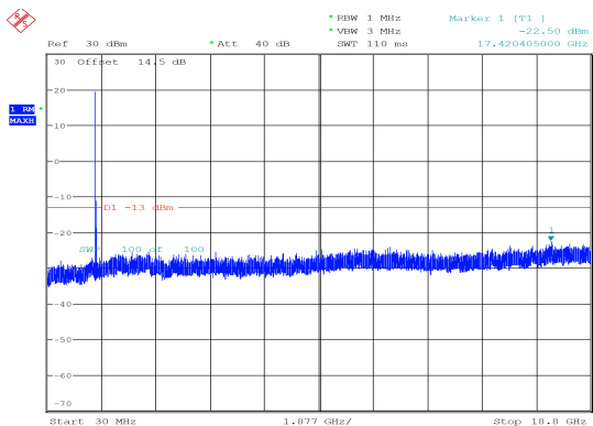
1.4MHz_Low_QPSK_6@0 -22.50 dBm
