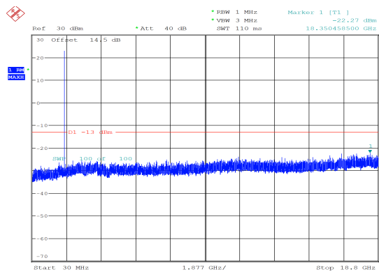
1.4MHz_High_QPSK_1@5 -22.27 dBm
