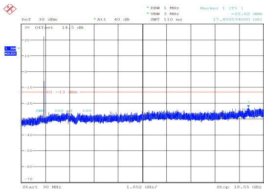
20MHz_High_QPSK_1@0 -22.62 dBm
