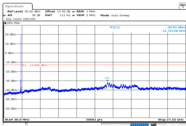
10MHz_Middle_QPSK_1@0 -30.82 dBm
