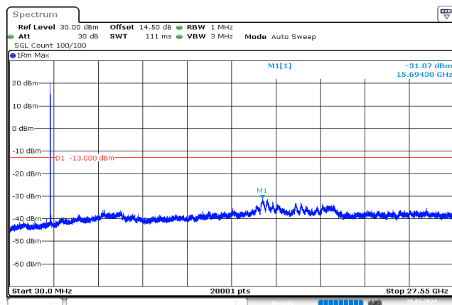
10MHz_Low_QPSK_1@0 -31.07 dBm
