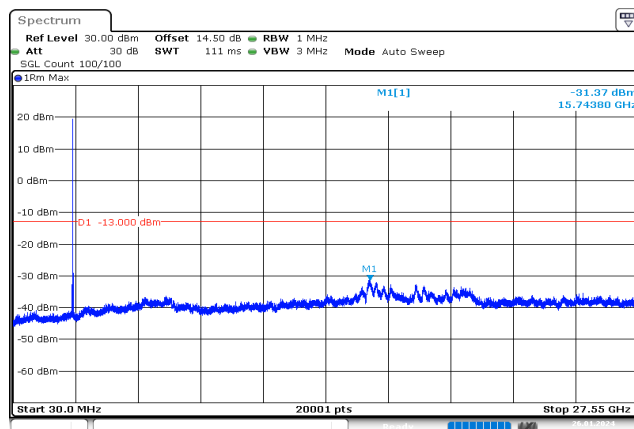
20MHz_High_QPSK_1@0 -31.37 dBm
