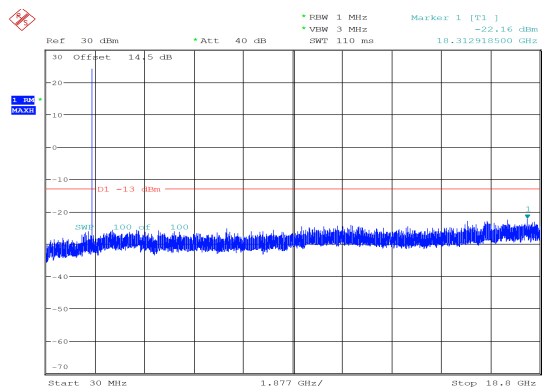
3MHz_High_QPSK_1@14 -22.16 dBm
