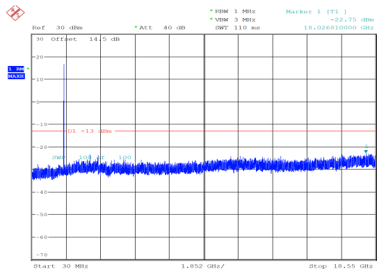
5MHz_High_QPSK_25@0 -22.75 dBm
