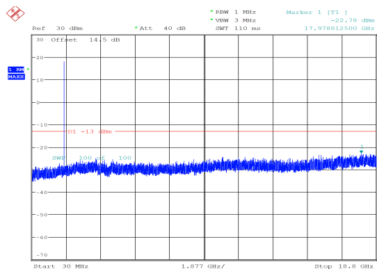
3MHz_High_QPSK_15@0 -22.78 dBm
