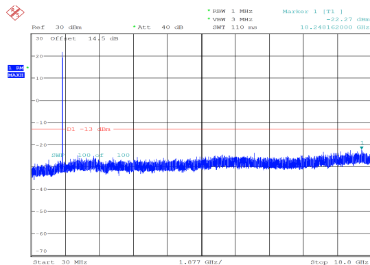
5MHz_Middle_QPSK_1@0 -22.27 dBm
