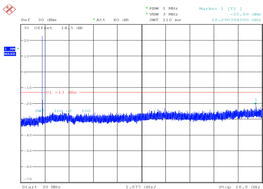
1.4MHz_Low_QPSK_1@0 -20.89 dBm
