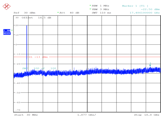
3MHz_Low_QPSK_1@14 -22.50 dBm
