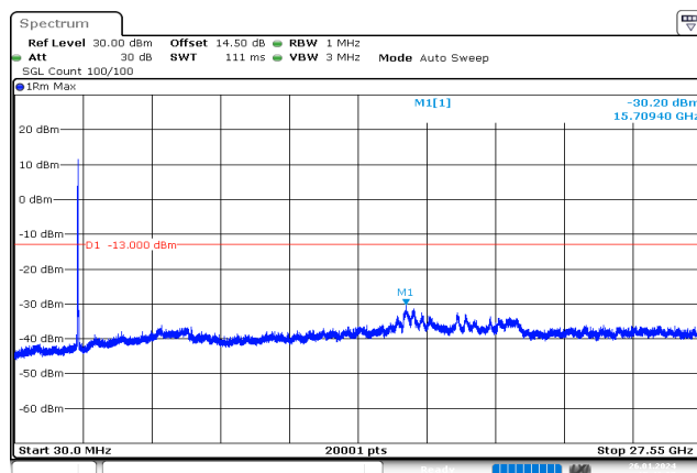
20MHz_Low_QPSK_100@0 -30.20 dBm
