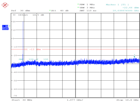
1.4MHz_Middle_QPSK_1@5 -22.66 dBm
