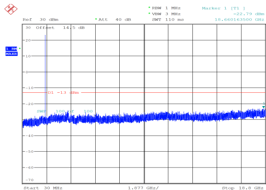
3MHz_High_QPSK_1@0 -22.79 dBm
