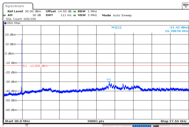
5MHz_High_QPSK_25@0 -31.42 dBm
