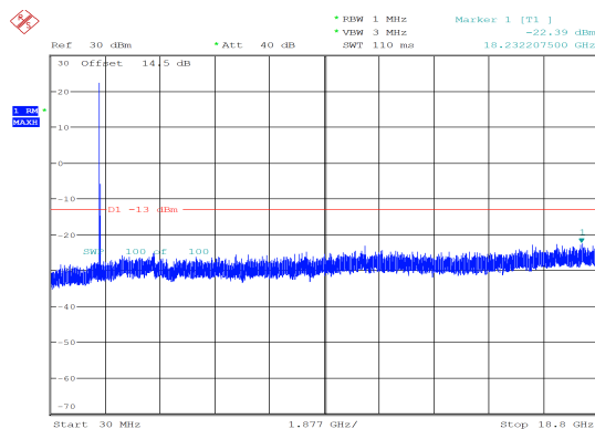
1.4MHz_Low_QPSK_1@5 -22.39 dBm
