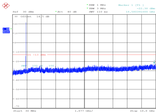
5MHz_Middle_QPSK_1@24 -22.38 dBm
