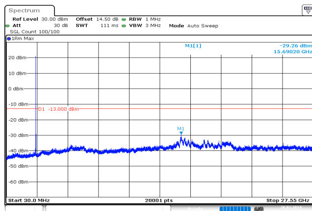
5MHz_High_QPSK_1@24 -29.26 dBm
