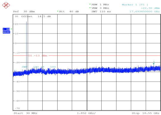
5MHz_Low_QPSK_1@0 -22.38 dBm
