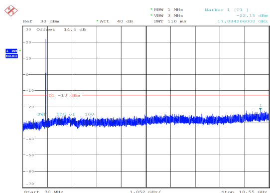
10MHz_High_QPSK_1@49 -22.15 dBm
