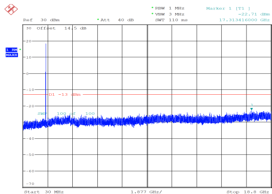
3MHz_Middle_QPSK_15@0 -22.71 dBm
