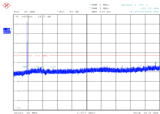
10MHz_High_QPSK_1@0 -22.32 dBm
