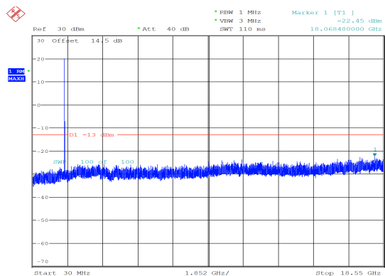
15MHz_Low_QPSK_1@0 -22.45 dBm
