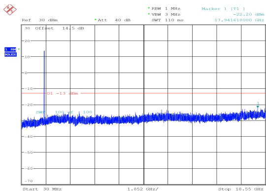
20MHz_High_QPSK_100@0 -22.20 dBm
