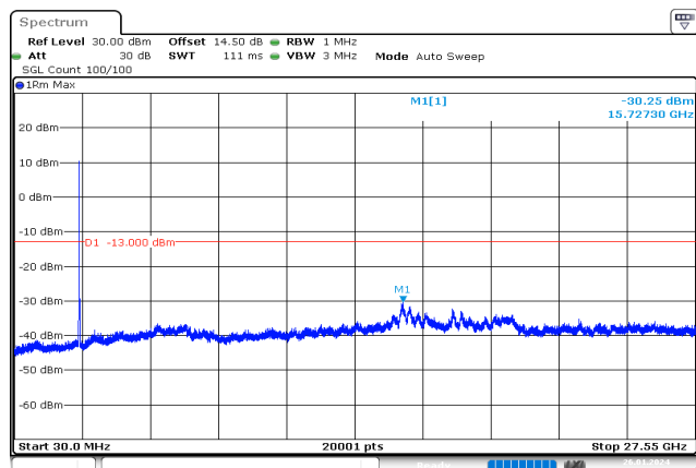
15MHz_High_QPSK_75@0 -30.25 dBm
