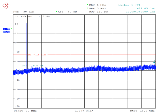
10MHz_Middle_QPSK_1@49 -22.45 dBm
