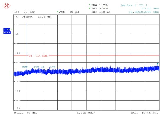
15MHz_Middle_QPSK_1@74 -22.29 dBm
