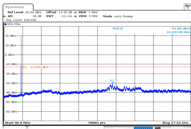
10MHz_Low_QPSK_1@49 -31.06 dBm
