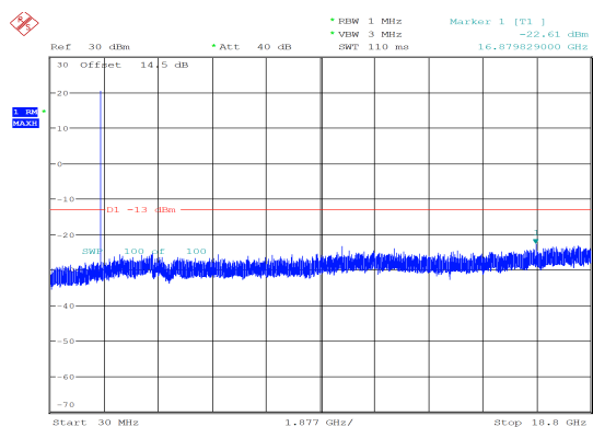
1.4MHz_High_QPSK_6@0 -22.61 dBm
