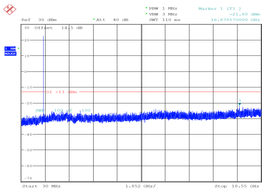
5MHz_Middle_QPSK_1@24 -21.60 dBm
