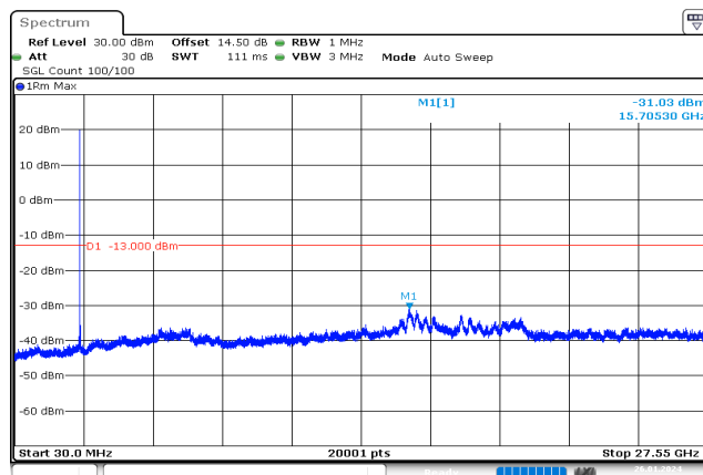
15MHz_Middle_QPSK_1@0 -31.03 dBm
