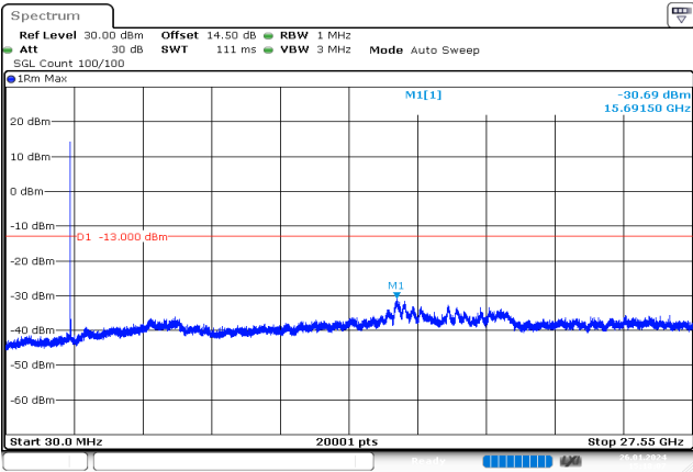
5MHz_Middle_QPSK_25@0 -30.69 dBm
