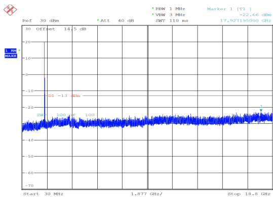
15MHz_Low_QPSK_1@0 -22.66 dBm
