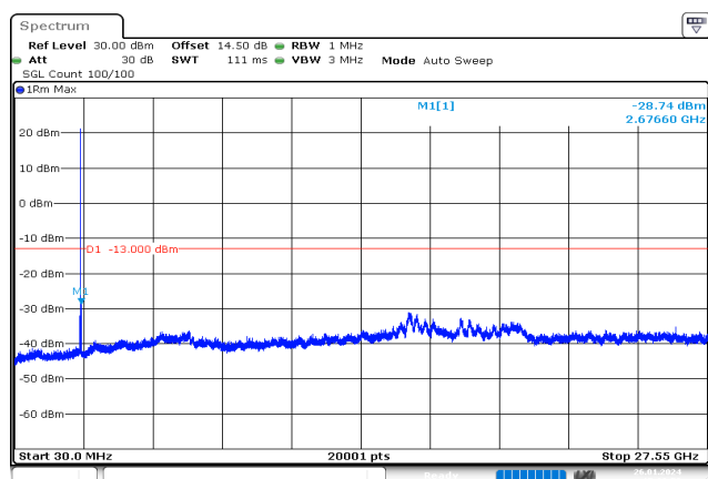
10MHz_High_QPSK_1@49 -28.74 dBm
