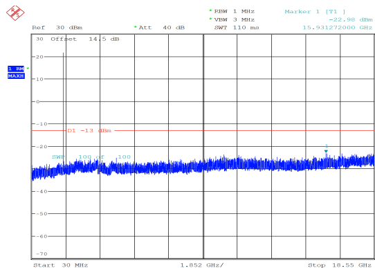
15MHz_Middle_QPSK_1@0 -22.98 dBm
