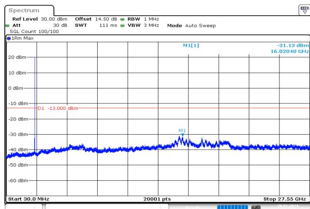
15MHz_Middle_QPSK_1@74 -31.13 dBm
