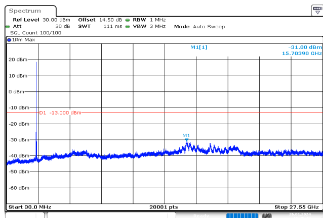
20MHz_Middle_QPSK_1@0 -31.00 dBm
