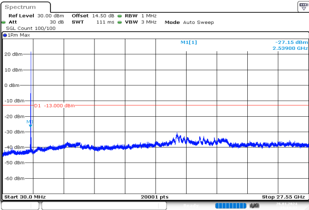
5MHz_Low_QPSK_1@24 -27.15 dBm
