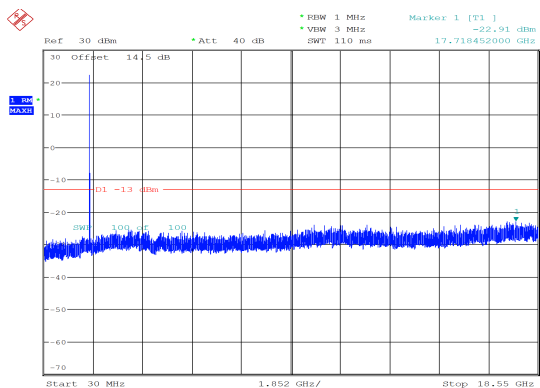
15MHz_High_QPSK_1@0 -22.91 dBm
