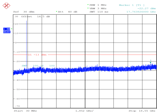
10MHz_Middle_QPSK_1@0 -22.27 dBm
