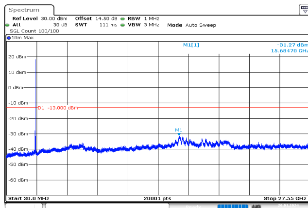
10MHz_High_QPSK_1@0 -31.27 dBm
