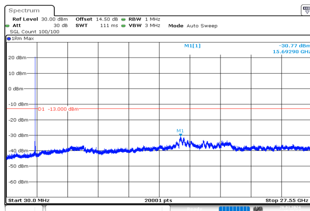
10MHz_Middle_QPSK_1@49 -30.77 dBm
