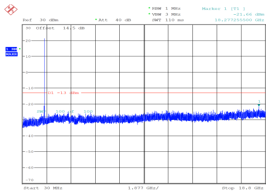
15MHz_Low_QPSK_1@74 -21.66 dBm
