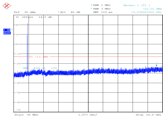
3MHz_Middle_QPSK_1@0 -22.55 dBm
