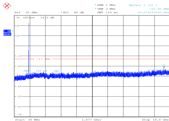
1.4MHz_Middle_QPSK_1@0 -22.00 dBm
