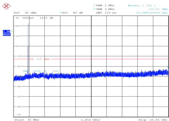
20MHz_High_QPSK_1@99 -22.21 dBm
