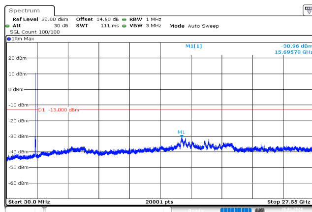
15MHz_Middle_QPSK_75@0 -30.96 dBm
