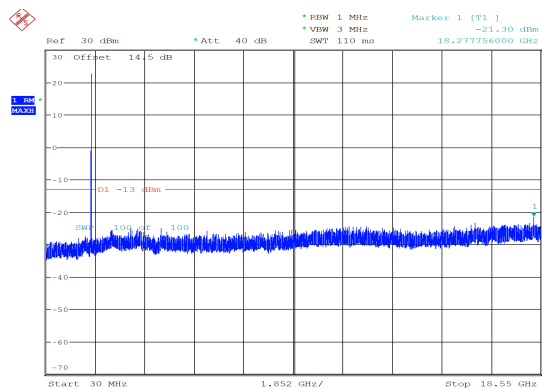
15MHz_Low_QPSK_1@74 -21.30 dBm
