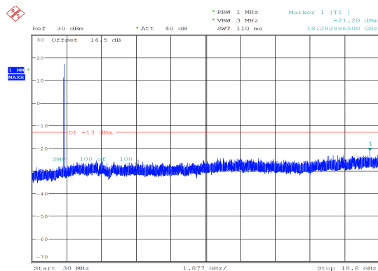
5MHz_Middle_QPSK_25@0 -21.20 dBm
