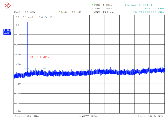
15MHz_Middle_QPSK_1@0 -22.63 dBm
