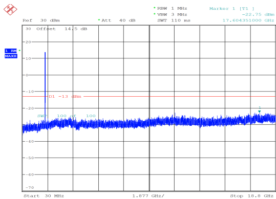
15MHz_Low_QPSK_75@0 -22.75 dBm
