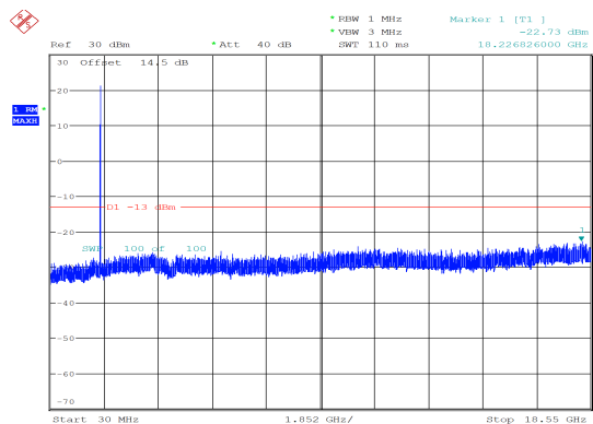
5MHz_High_QPSK_1@0 -22.73 dBm
