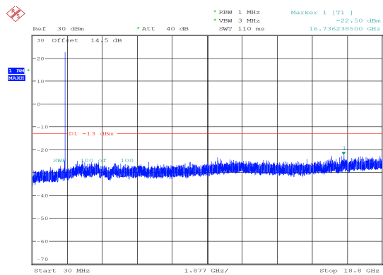
5MHz_High_QPSK_1@24 -22.50 dBm
