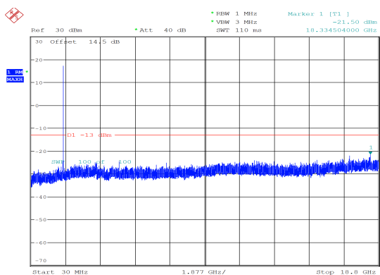
5MHz_High_QPSK_25@0 -21.50 dBm
