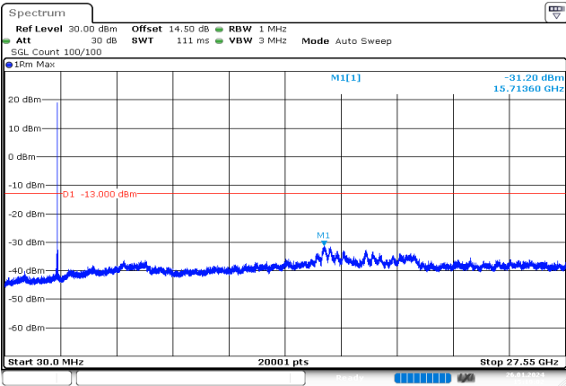
5MHz_Middle_QPSK_1@0 -31.20 dBm
