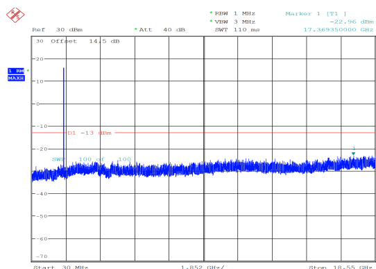
10MHz_High_QPSK_50@0 -22.96 dBm
