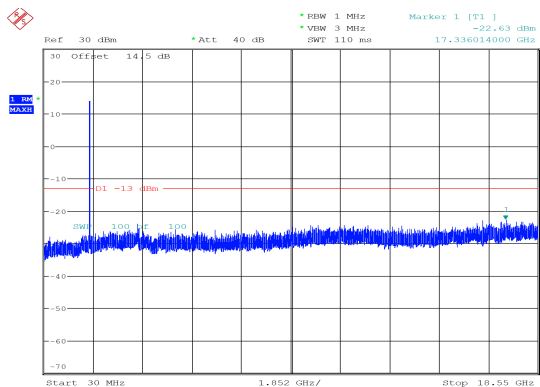
15MHz_High_QPSK_75@0 -22.63 dBm
