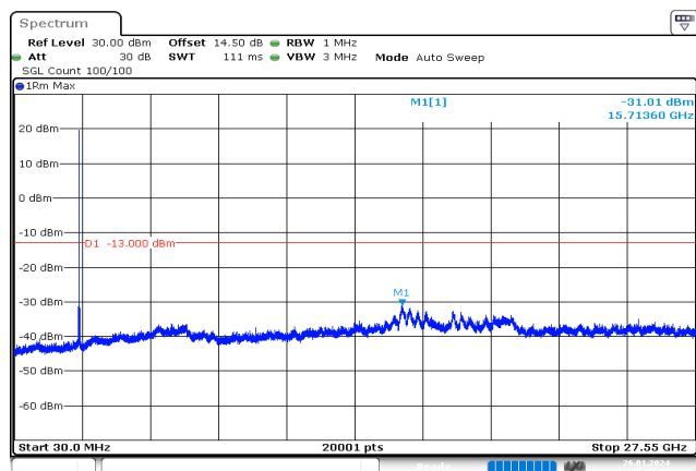
15MHz_High_QPSK_1@0 -31.01 dBm
