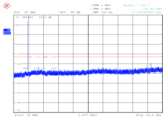
1.4MHz_High_QPSK_1@0 -22.43 dBm
