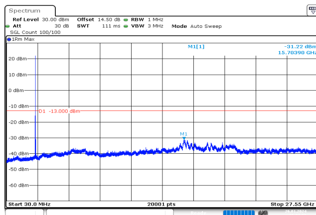
15MHz_Low_QPSK_1@74 -31.22 dBm
