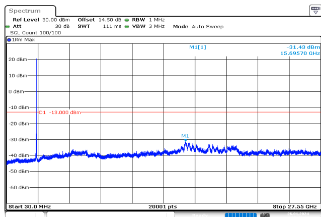
20MHz_High_QPSK_1@99 -31.43 dBm
