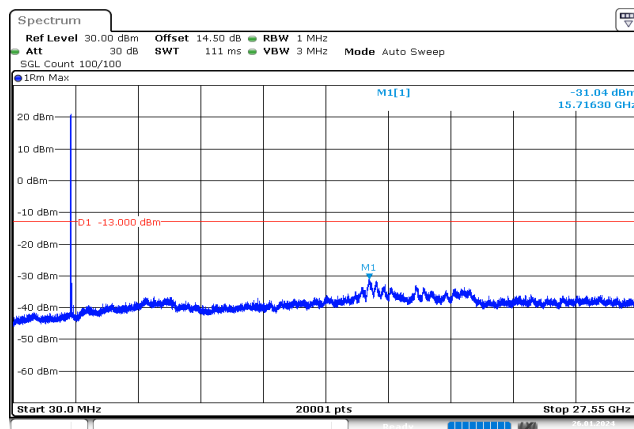
20MHz_Low_QPSK_1@0 -31.04 dBm
