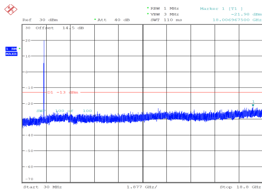
5MHz_Low_QPSK_1@24 -21.98 dBm
