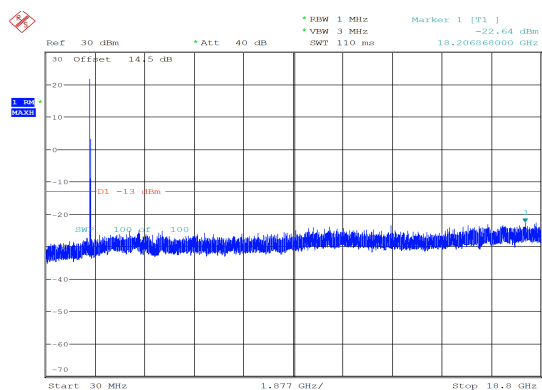
10MHz_Low_QPSK_1@0 -22.64 dBm
