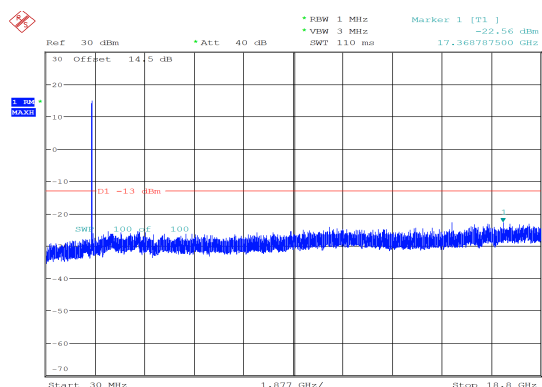
10MHz_High_QPSK_50@0 -22.56 dBm
