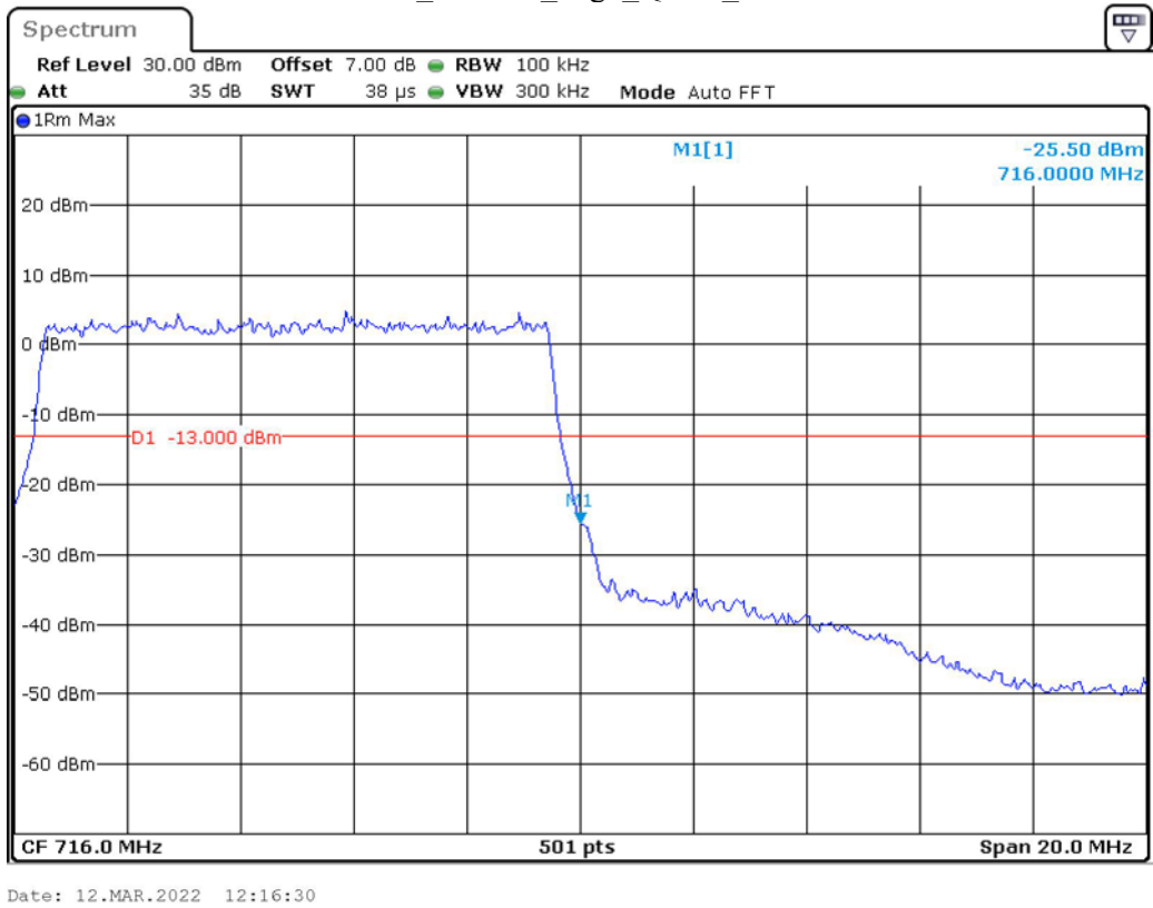
Band 12_10 MHz_High_QPSK_RB50#0
