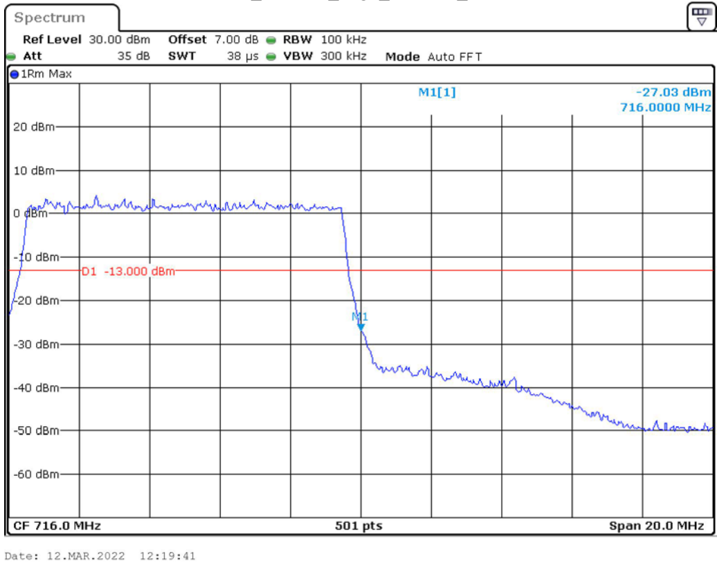
Band 17_10 MHz_High_16QAM_RB50#0
