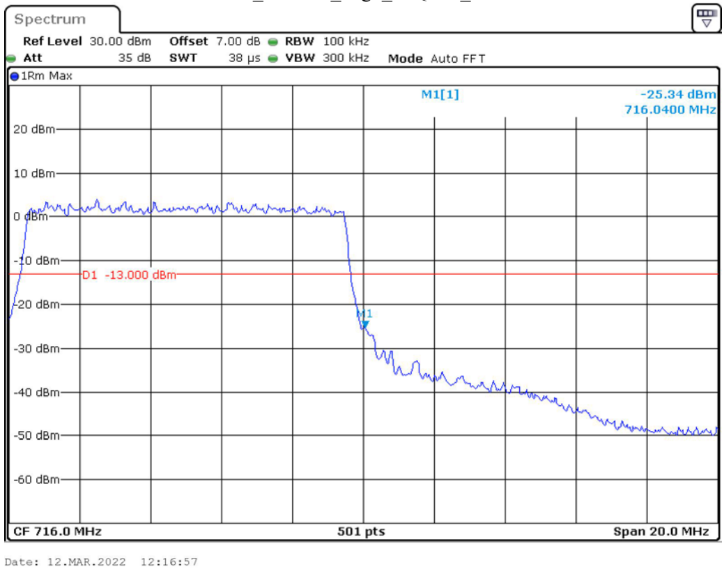
Band 12_10 MHz_High_16QAM_RB50#0
