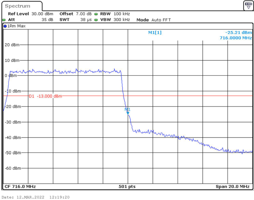
Band 17_10 MHz_High_QPSK_RB50#0
