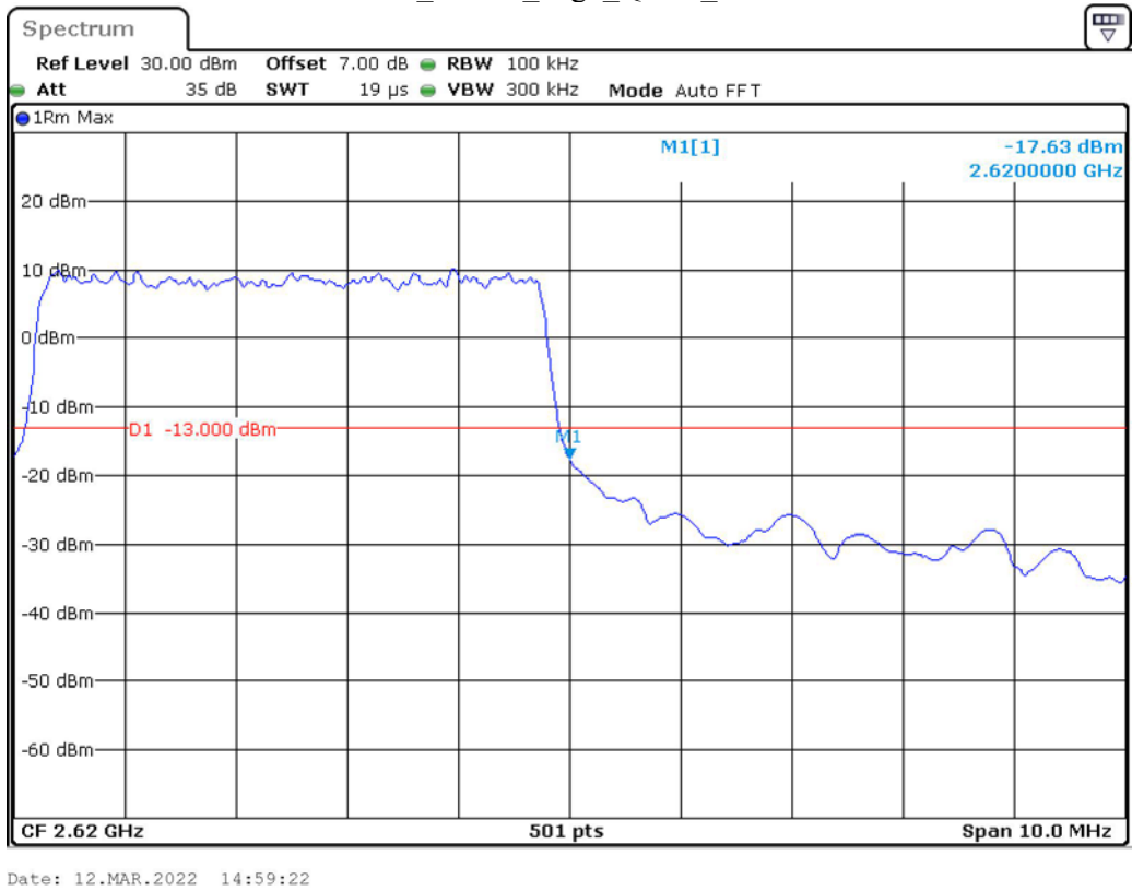
Band 38_5 MHz_High_QPSK_RB25#0
