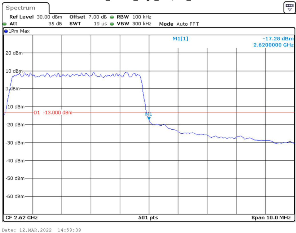
Band 38_5 MHz_High_16QAM_RB25#0
