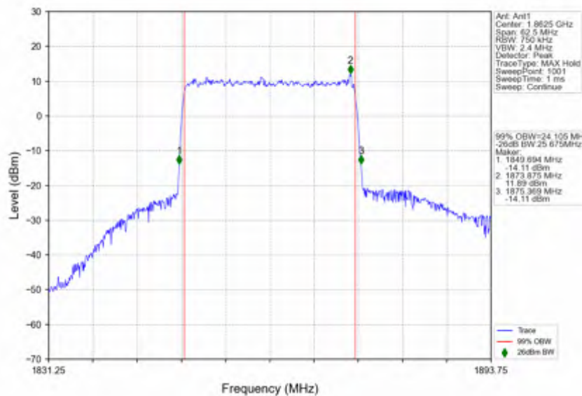
n25_15kHz_SISO_NTNV_25MHz_CP-OFDM_QPSK_1862.5MHz_Outer_Full
