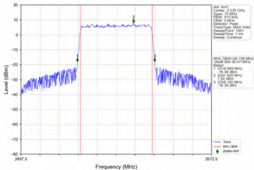
n7 30kHz SISO NTV 30MHz CP-OFDM 256 QAM 2535MHz Outer Full
