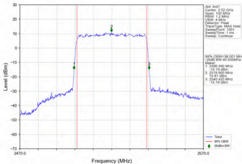
n7_30kHz_SISO_NTNV_40MHz_CP-OFDM 64 QAM 2520MHz_Outer_Full
