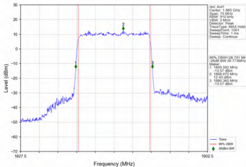
n25_15kHz_SISO_NTNV_30MHz_DFT-s-OFDM 64 QAM_1865MHz_Outer_Full
