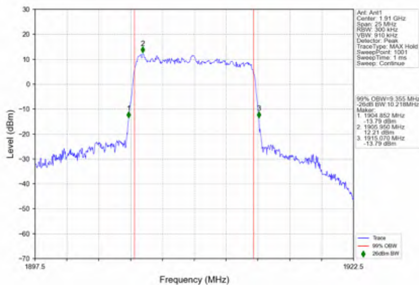
n25 15kHz SISO NTNV 10MHz CP-OFDM 64 QAM 1910MHz Outer Full
