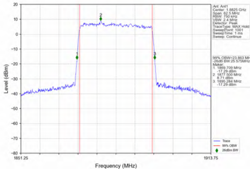
n25_15kHz_SISO_NTNV_25MHz_CP-OFDM_256_QAM_1882.5MHz_Outer_Full
