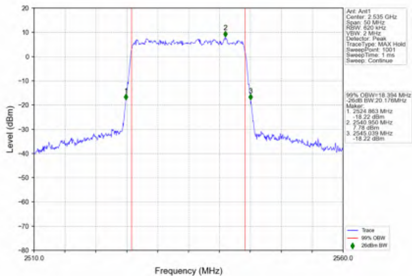
n7 30kHz SISO NTV 20MHz CP-OFDM 256 QAM 2535MHz Outer Full
