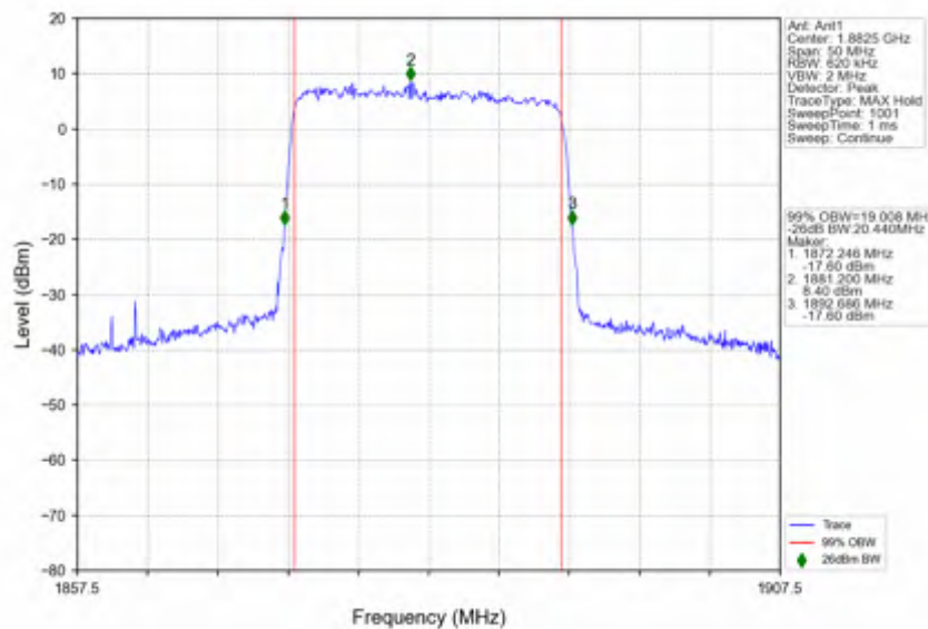
n25 15kHz SISO NTNV 20MHz CP-OFDM 256 QAM 1882.5MHz Outer Full
