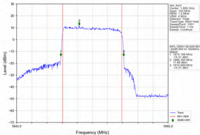
n25_15kHz_SISO_NTNV_40MHz_CP-OFDM 64 QAM_1895MHz_Outer_Full
