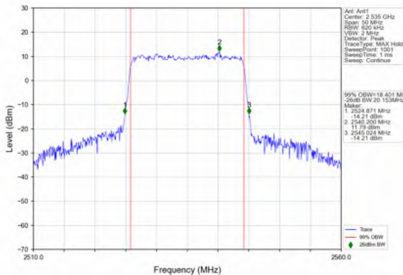
n7_30kHz_SISO_NTNV_20MHz_CP-OFDM_16_QAM_2535MHz_Outer_Full
