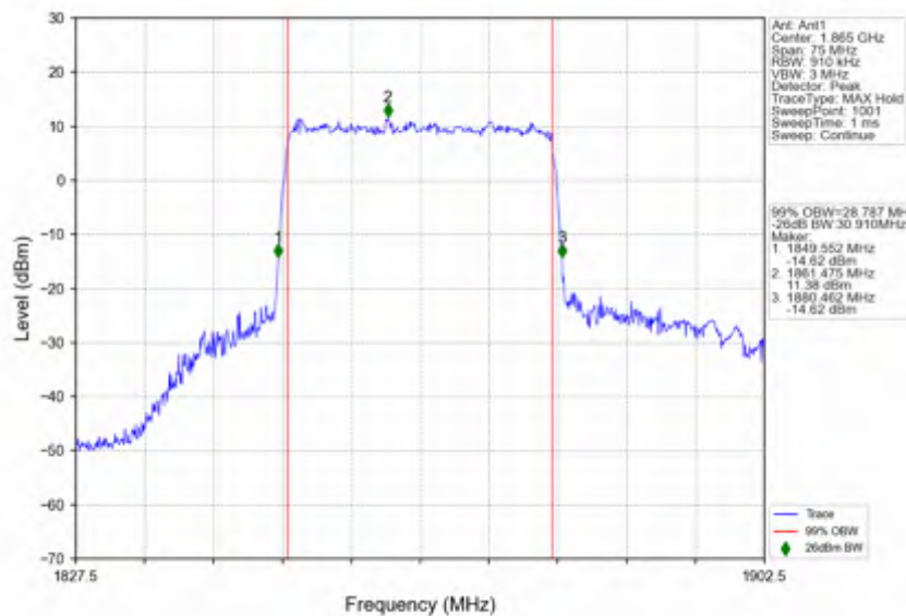
n25_15kHz_SISO_NTV_30MHz_CP-OFDM_QPSK_1865MHz_Outer_Full
