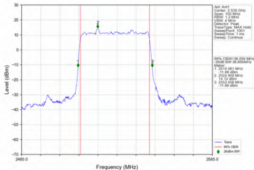
n7_30kHz_SISO_NTNV_40MHz_DFT-s-OFDM PI/2 BPSK_2535MHz_Outer_Full
