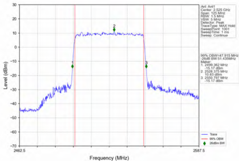
n7 30kHz SISO NTN 50MHz CP-OFDM 64 QAM 2525MHz Outer Full
