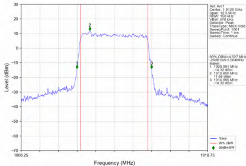
n25_15kHz_SISO_NTNV_5MHz_CP-OFDM_64_QAM_1912.5MHz_Outer_Full
