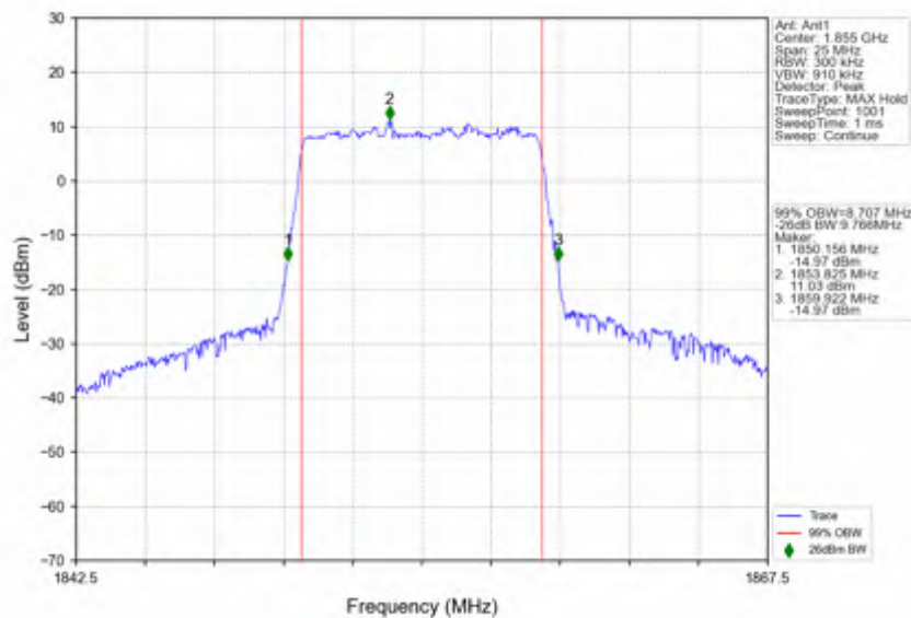
n25_30kHz_SISO_NTNV_10MHz_CP-OFDM 64 QAM_1855MHz_Outer_Full
