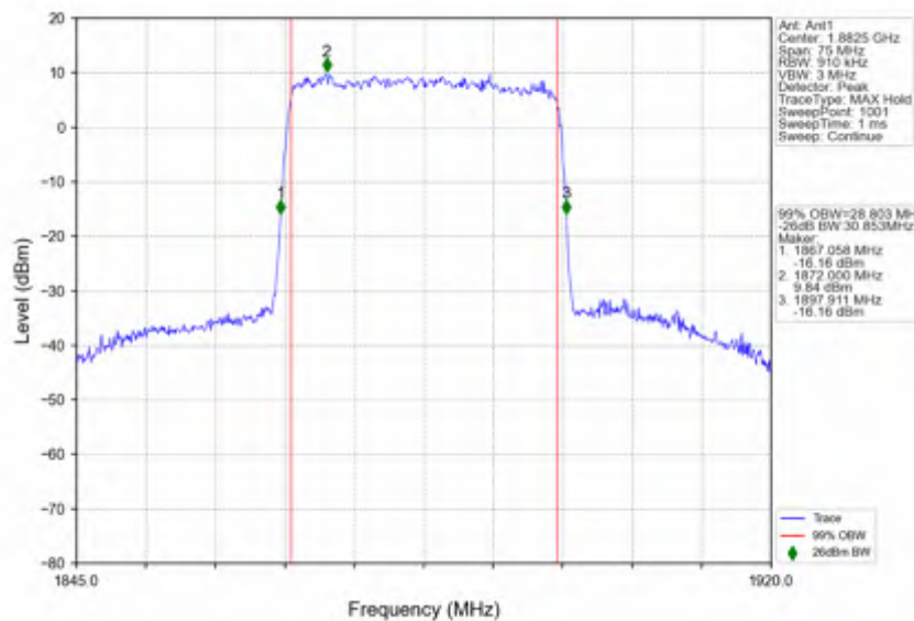
n25_15kHz_SISO_NTNV_30MHz_DFT-s-OFDM_256_QAM_1882.5MHz_Outer_Full
