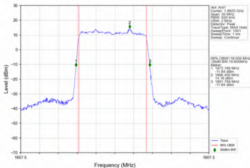
n25_15kHz_SISO_NTNV_20MHz_DFT-s-OFDM_PI/2_BPSK_1882.5MHz_Outer_Full
