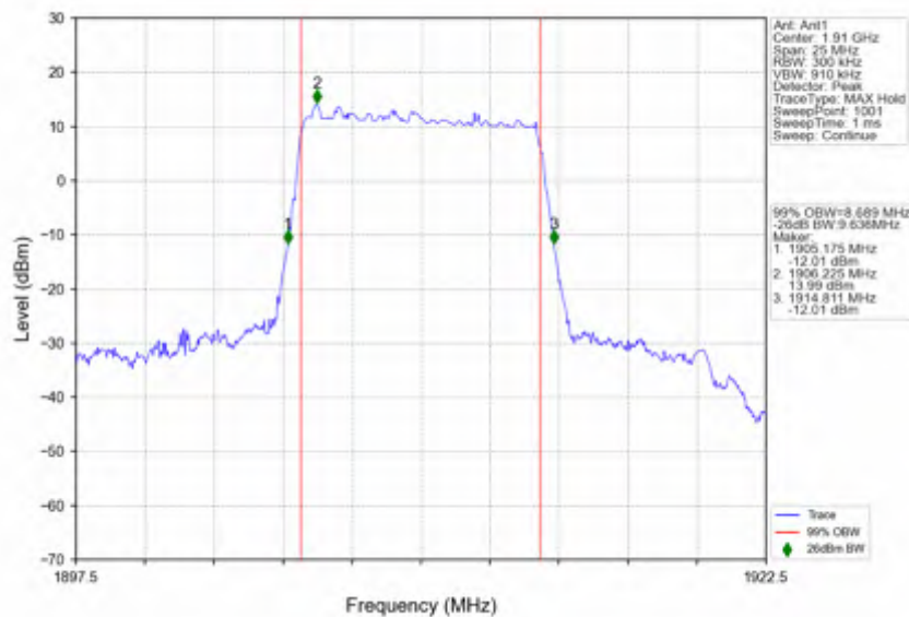
n25_30kHz_SISO_NTNV_10MHz_DFT-s-OFDM_QPSK_1910MHz_Outer_Full
