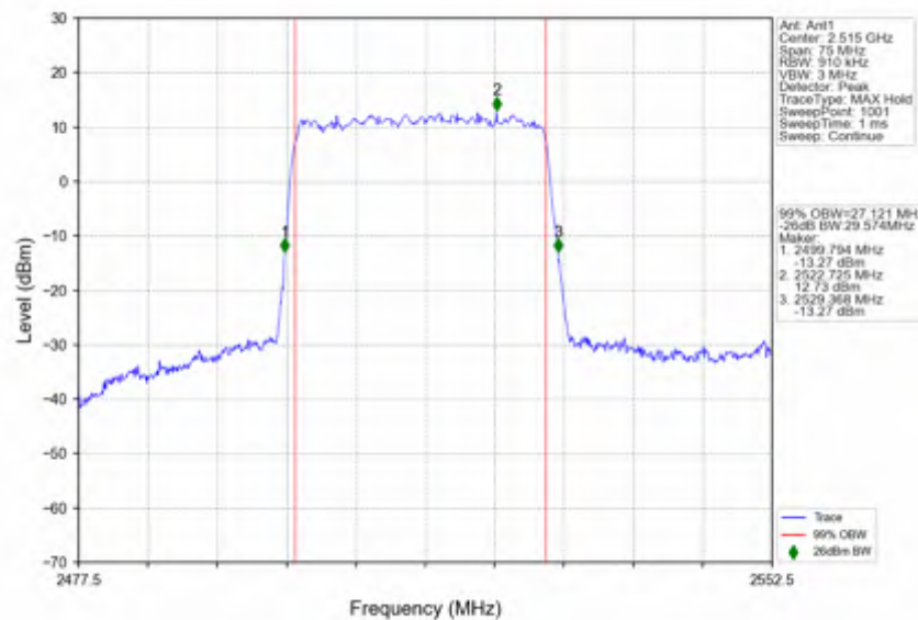
n7_30kHz_SISO_NTNV_30MHz_DFT-s-OFDM QPSK_2515MHz_Outer_Full
