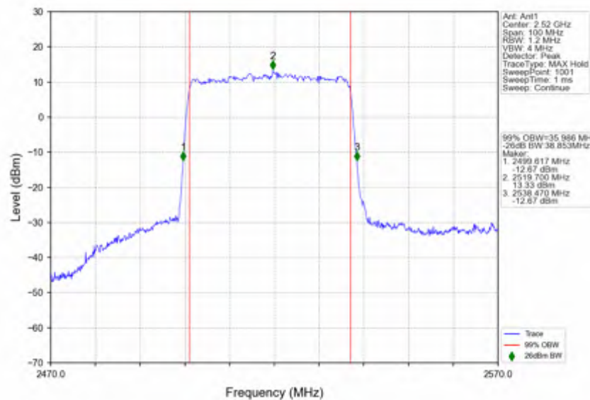
n7_30kHz_SISO_NTNV_40MHz_DFT-s-OFDM QPSK_2520MHz_Outer_Full
