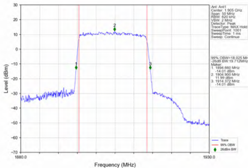
n25_15kHz_SISO_NTNV_20MHz_DFT-s-OFDM 64 QAM_1905MHz_Outer_Full
