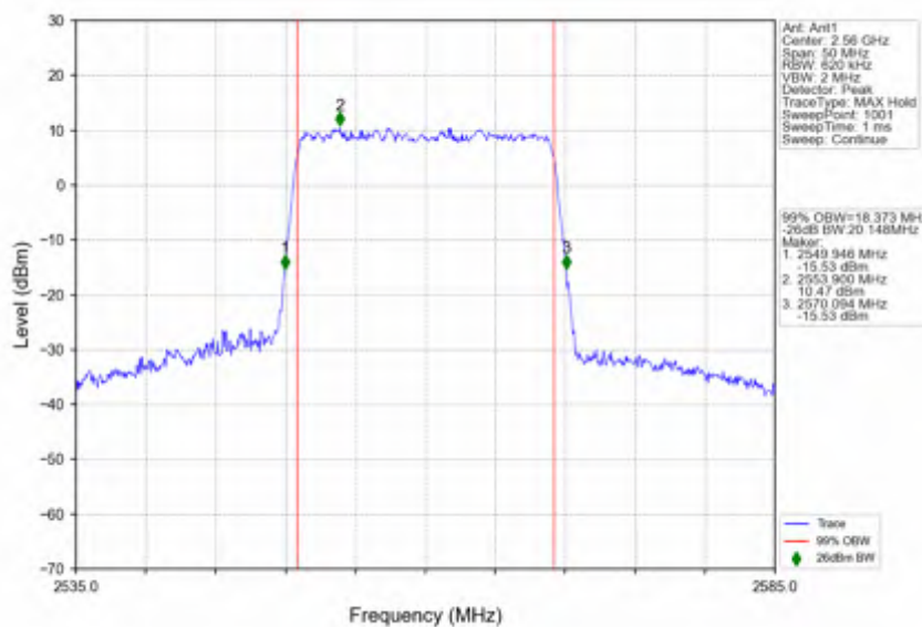
n7 30kHz SISO NTN 20MHz CP-OFDM 64 QAM 2560MHz Outer Full
