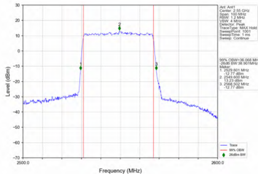
n7_30kHz_SISO_NTNV_40MHz_DFT-s-OFDM_QPSK_2550MHz_Outer_Full
