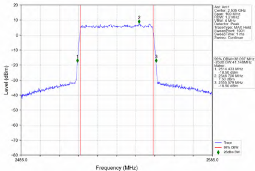
n7 30kHz SISO NTV 40MHz CP-OFDM 256 QAM 2535MHz Outer Full
