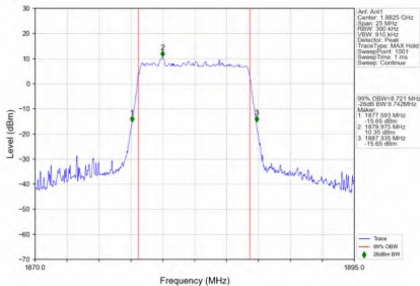
n25_30kHz_SISO_NTNV_10MHz_DFT-s-OFDM_256_QAM_1882.5MHz_Outer_Full
