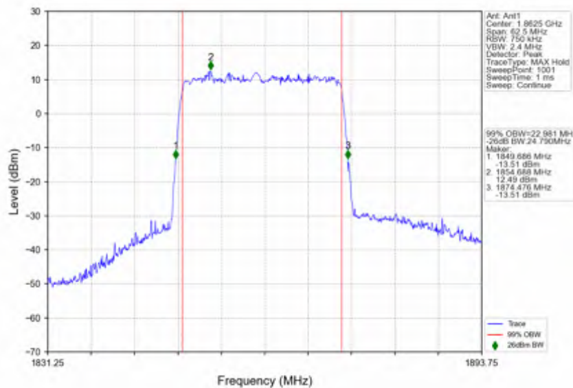
n25_15kHz_SISO_NTV_25MHz_DFT-s-OFDM 64 QAM_1862.5MHz_Outer_Full
