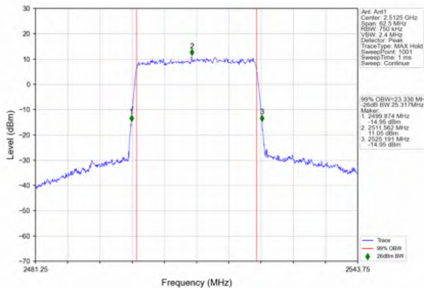
n7_30kHz_SISO_NTNV_25MHz_CP-OFDM QPSK_2512.5MHz_Outer_Full
