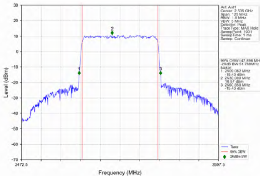
n7_30kHz_SISO_NTNV_50MHz_CP-OFDM_16_QAM_2535MHz_Outer_Full
