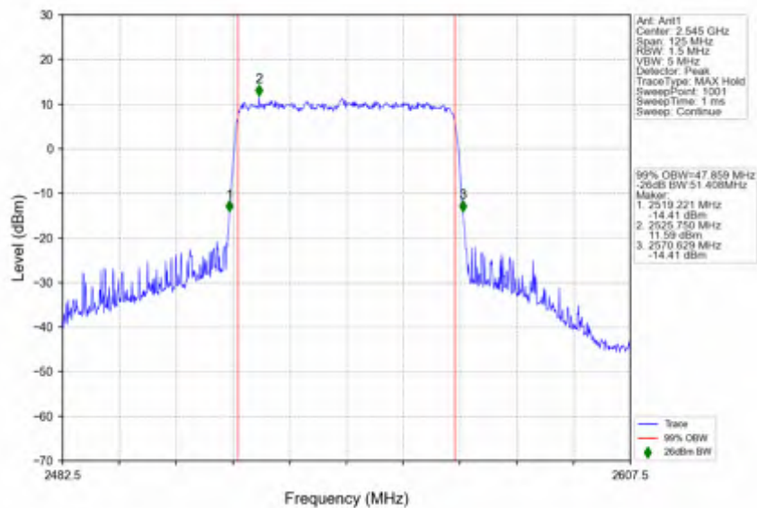
n7_30kHz_SISO_NTNV_50MHz_CP-OFDM_QPSK_2545MHz_Outer_Full
