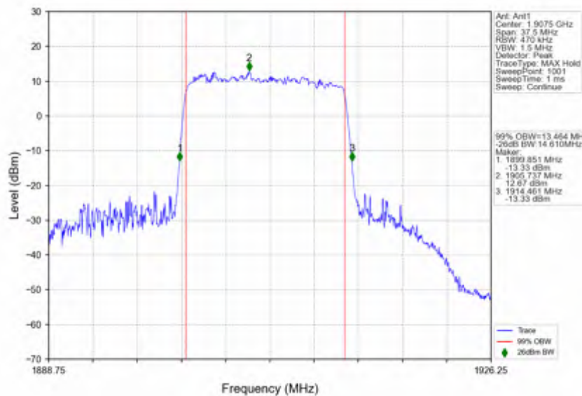
n25_15kHz_SISO_NTV_15MHz_DFT-s-OFDM 64 QAM_1907.5MHz_Outer_Full
