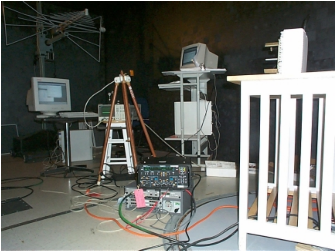
Figure 1 Radiated Emission (18-220 GHz) test setup
