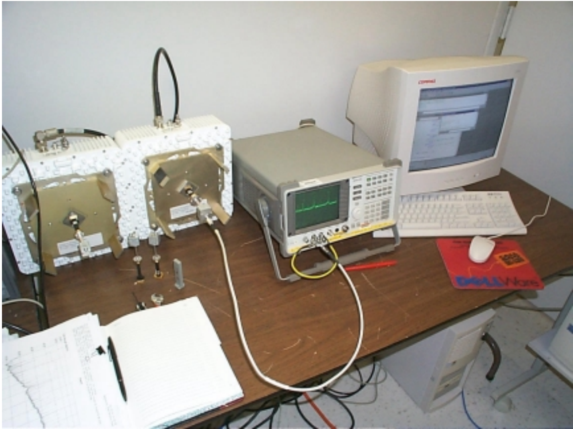
Figure 3: Conducted Spurious Emission Test setup
