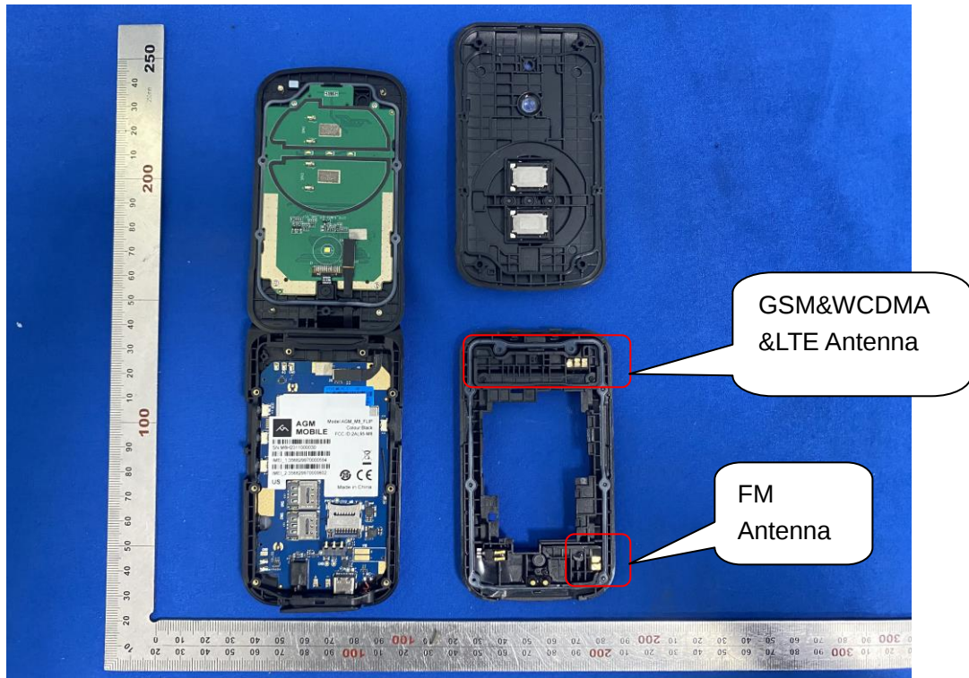
INTERNAL VIEW OF EUT (FIGURE 1)
