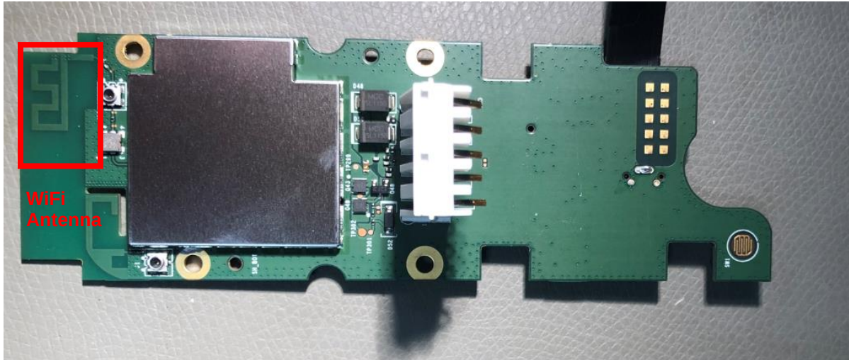
Figure 2. PCPA bottom side with Shield- Confidential
