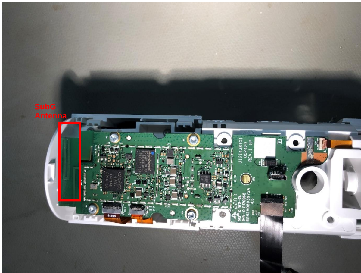
Figure 1. PCPA top side- Confidential
