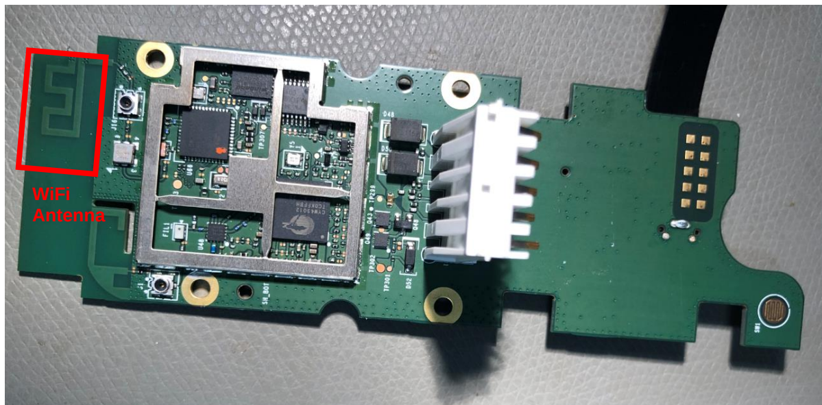
Figure 3. PCBA bottom side without shield- Confidential
