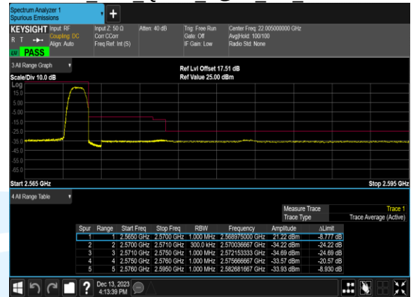
B7 15M QPSK 1@74 CH 21375
