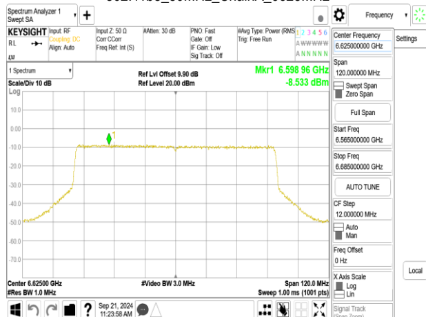
802.11be_80MHz_ChainA_6625MHz_484+242_MRU2
