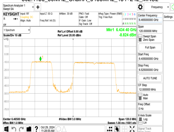
802.11be_80MHz_ChainA_6465MHz_484+242_MRU3
