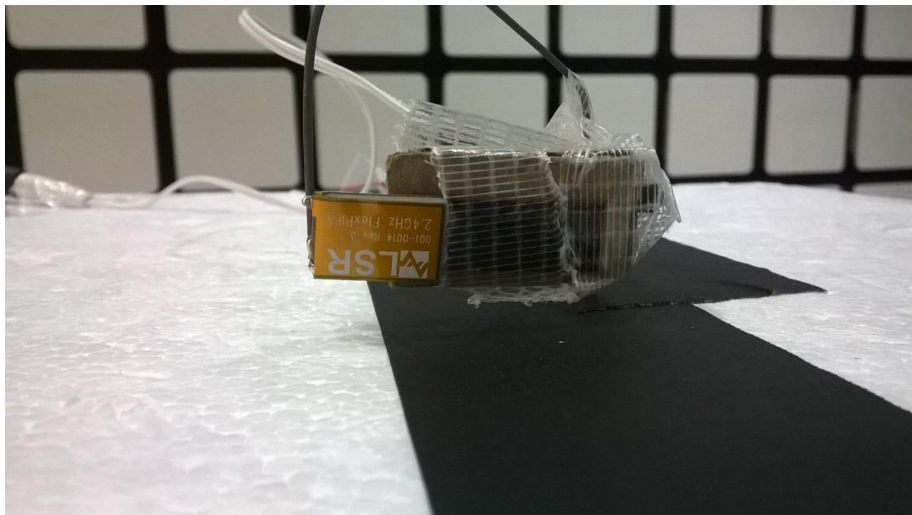
Figure 4 - Radiated Emissions Test Setup, Y axis
