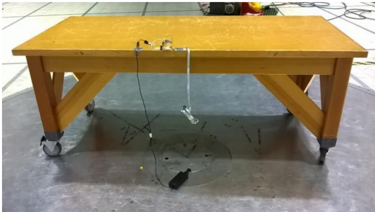
Figure 1 - Radiated Emissions Test Setup, 30MHz - 1GHz
