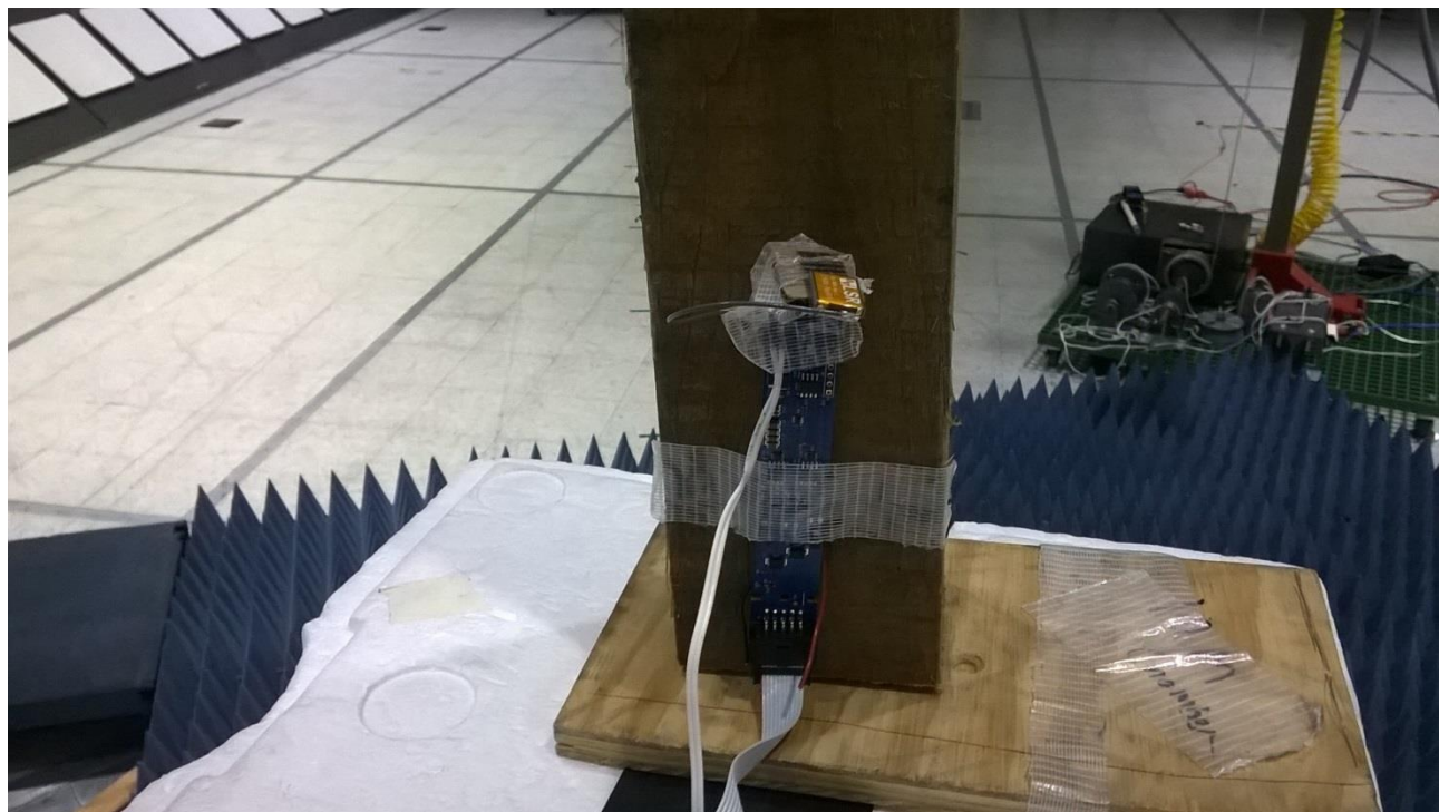
Figure 6 - Radiated Emissions Test Setup, Y axis
