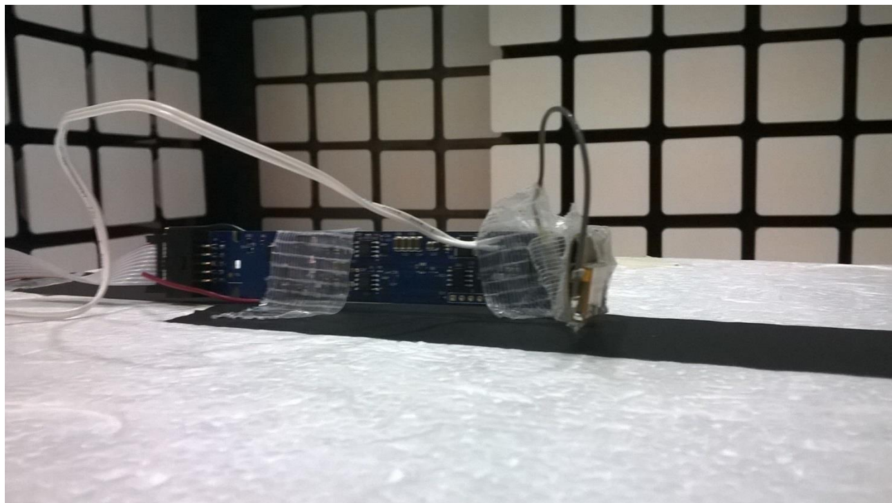
Figure 5 - Radiated Emissions Test Setup, Y axis (alternate view)
