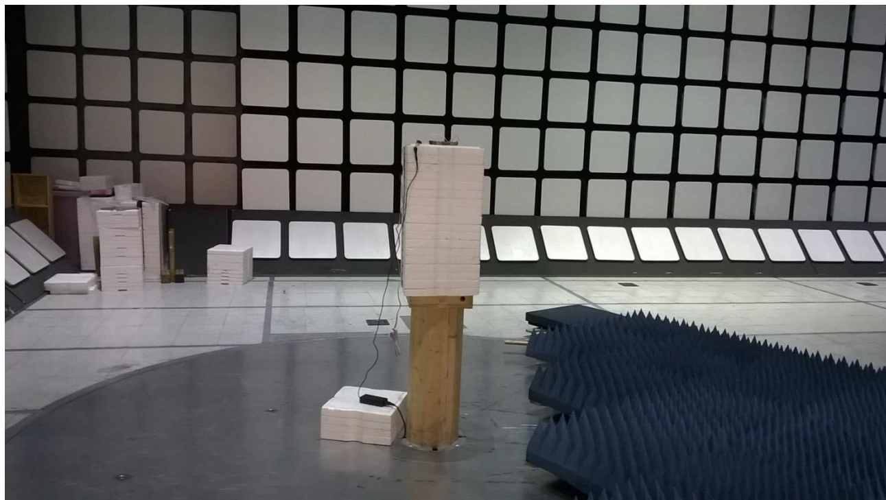
Figure 2 - Radiated Emissions Test Setup, 1 - 25 GHz
