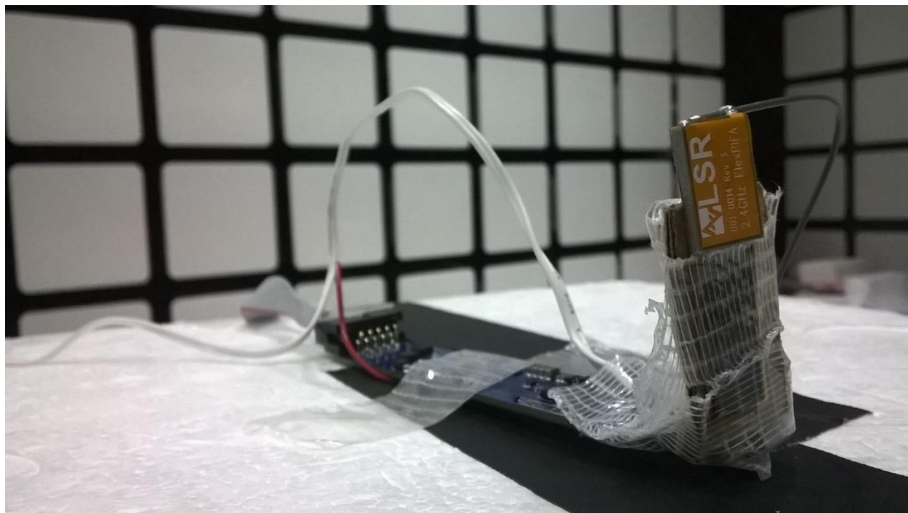
Figure 3 - Radiated Emissions Test Setup, X axis
