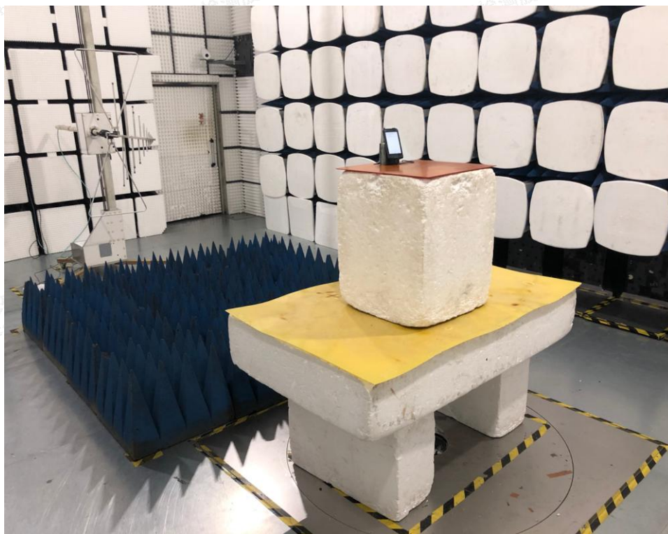
Radiated Emissions Measurement (Below 1GHz)
