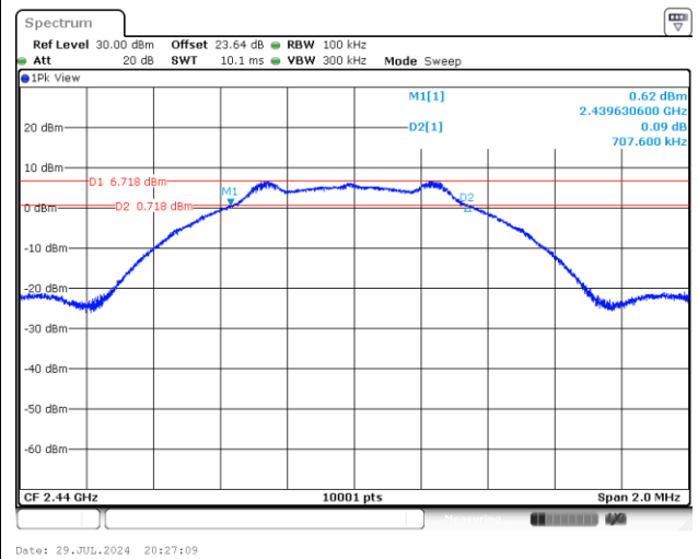
6 dB Bandwidth Plot on Channel 17
