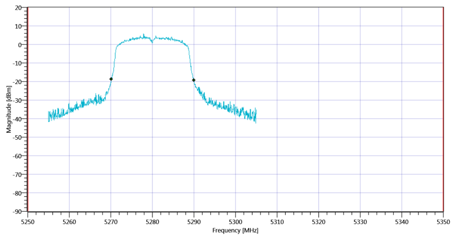
Plot_FCC Part 15.407 & ISSED Bandwidths ~ WLAN5Gx n-HT20 mode U-NII-2A_06112020_094929.png
