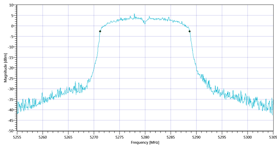
Plot_FCC Part 15.407 & ISSED Bandwidths ~ WLAN5Gx n-HT20 mode U-NII-2A 99PCT_06112020_094917.png
