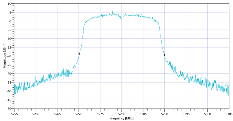
Plot_FCC Part 15.407 & ISSED Bandwidths ~ WLAN5Gx n-HT20 mode U-NII-2A 26dB_06112020_094926.png
