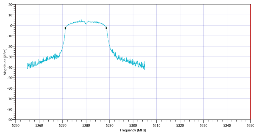
Plot_FCC Part 15.407 & ISSED Bandwidths ~ WLAN5Gx n-HT20 mode U-NII-2A_06112020_094921.png
