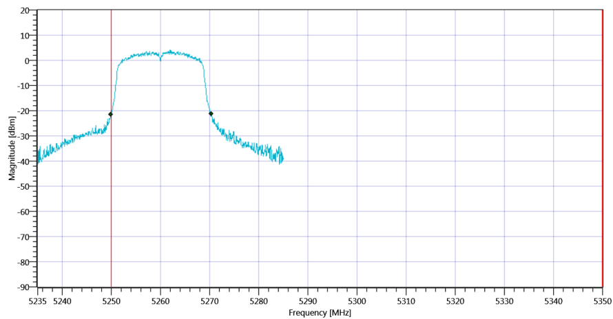
Plot_FCC Part 15.407 & ISSED Bandwidths ~ WLAN5Gx n-HT20 mode U-NII-2A_06112020_094608.png
