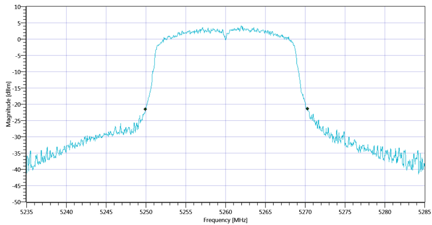
Plot_FCC Part 15.407 & ISSED Bandwidths ~ WLAN5Gx n-HT20 mode U-NII-2A 26dB_06112020_094605.png
