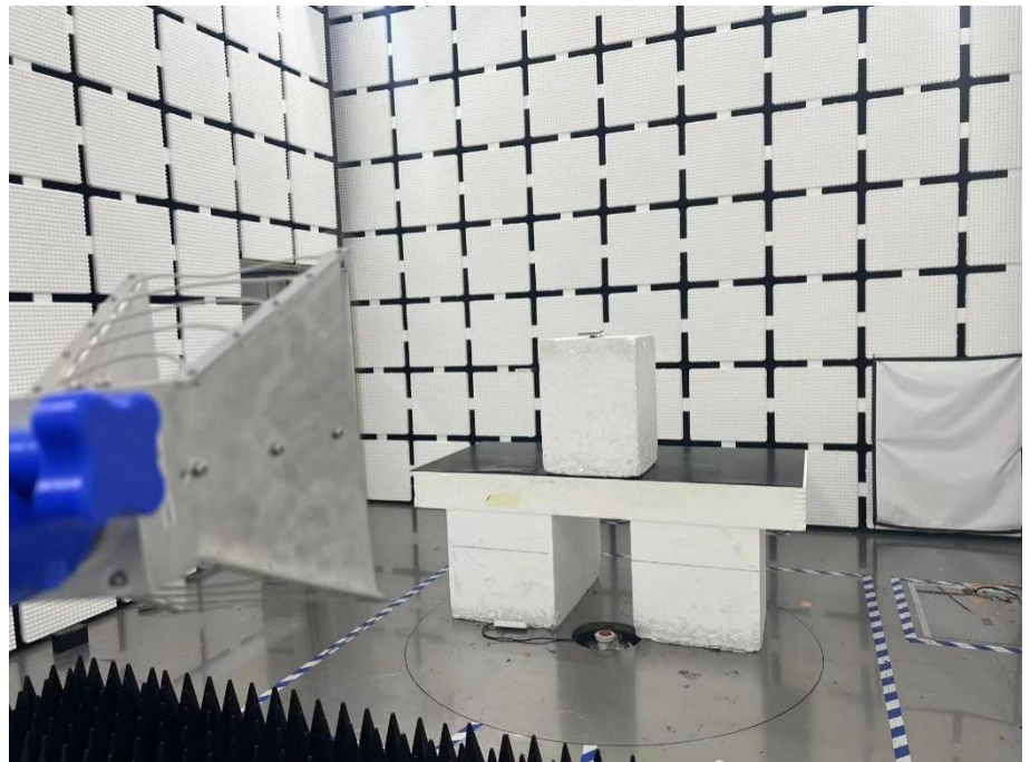
Radiation Emission Test Setup (1GHz to 18GHz)
