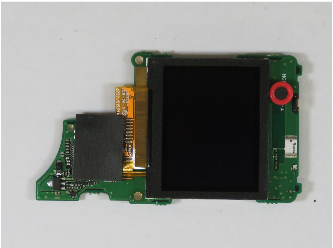
IC-F7010S/T FRONT SIDE A with LCD
