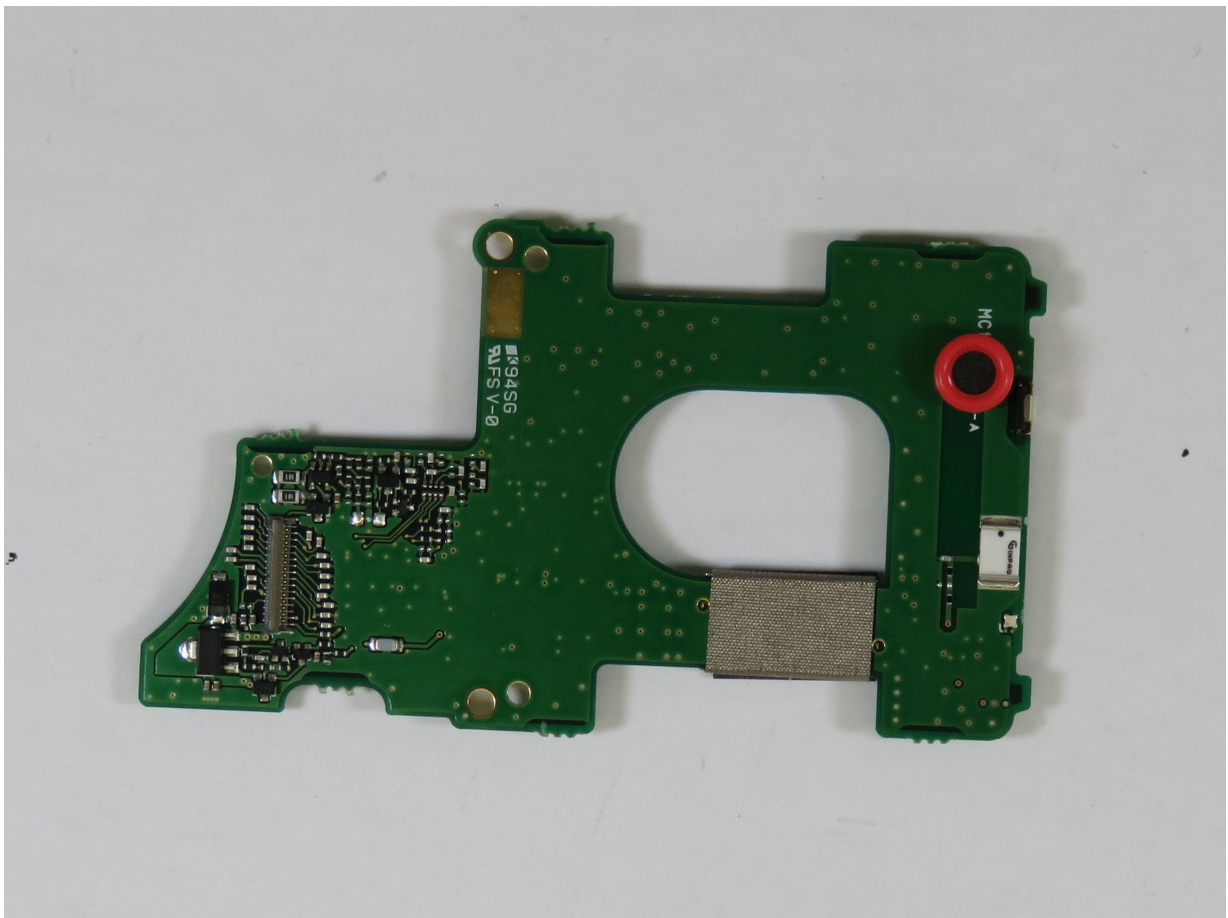
IC-F7010S/T FRONT SIDE A
