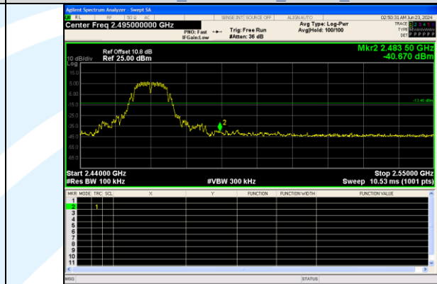
Out Of Band Emission IEEE 802.11b Channel 11 20MHz Antenna 0
