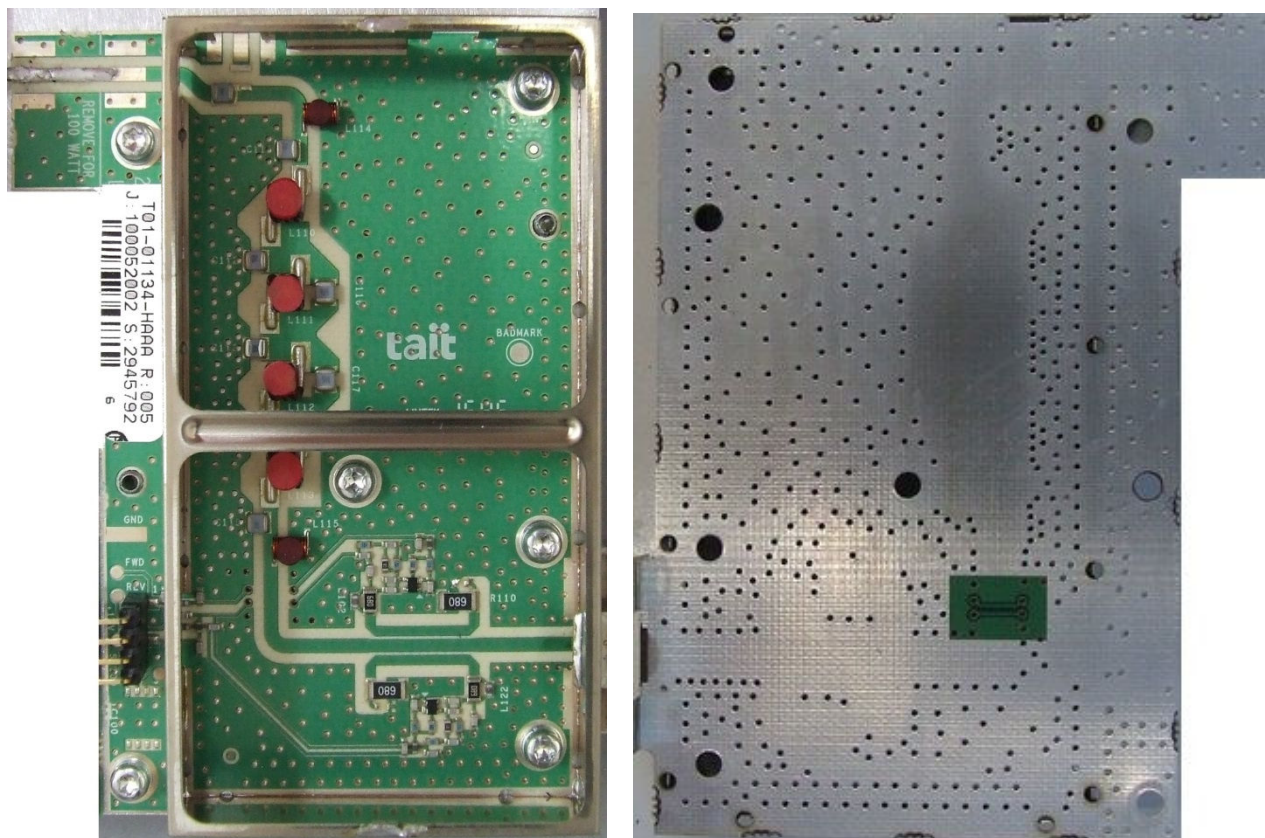
Photograph 19 & 20: Power Amplifier LPF PCB – Top & Bottom
