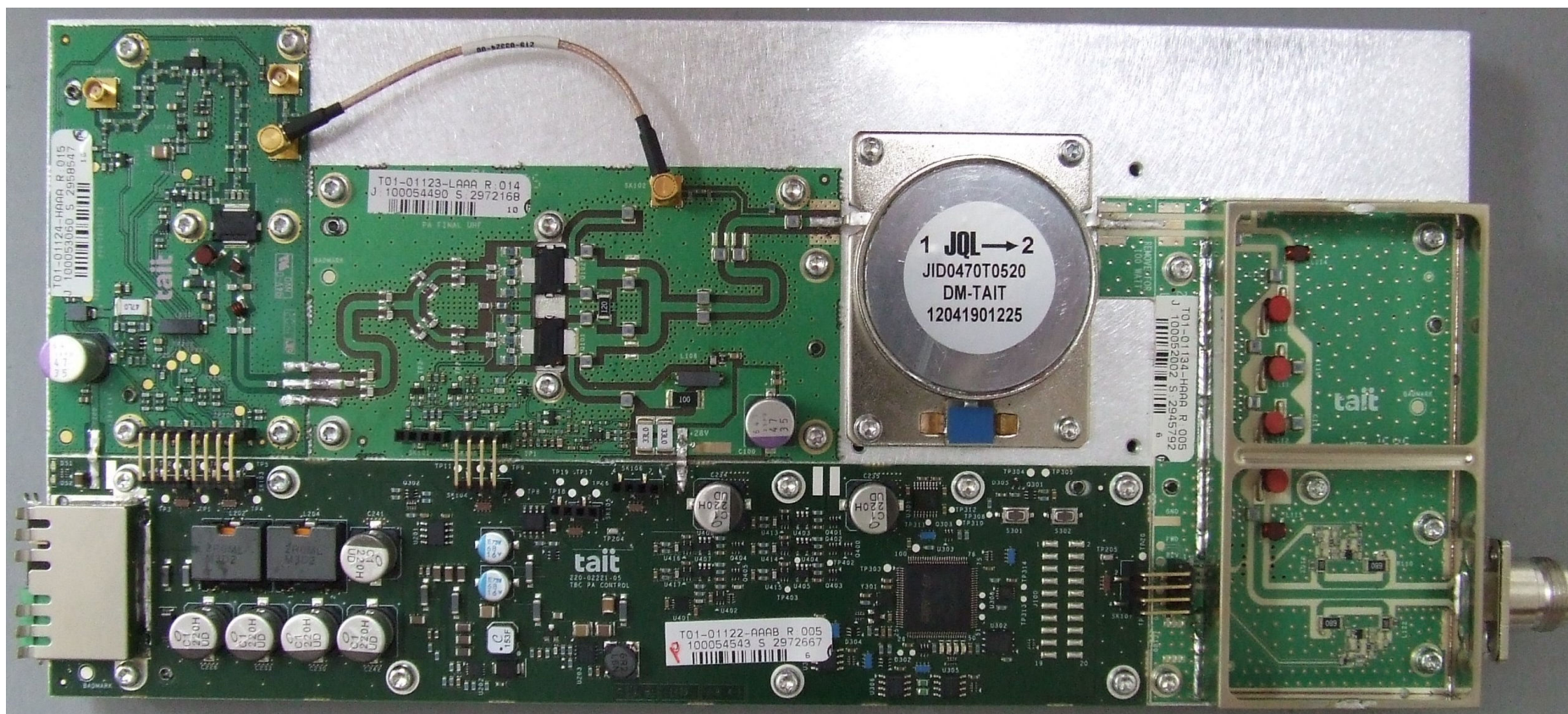
Photograph 16: 50 Watt Power Amplifier – (shields off)
