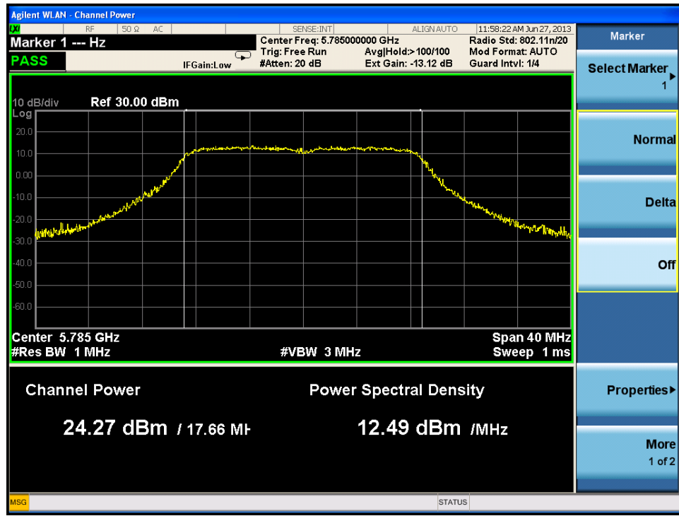
Figure 4.5.1 The Peak Output Power Measured for 802.11n (20MHz-2Tx-2S) Carrier at Channel 157/5785MHz, 18dBm Setting (Both High and Medium Gain Antenna), OFDM/SM, MCS8, Port 1.
