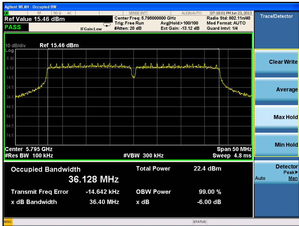
Figure 4.4.4 The Maximum 6dB DTS Bandwidth Measured (36.40MHz) for 802.11n (HT40-2Tx-1S) Carrier at Ch 159/5795MHz, 18dBm, OFDM/CDD, MCS0, Port 2.
