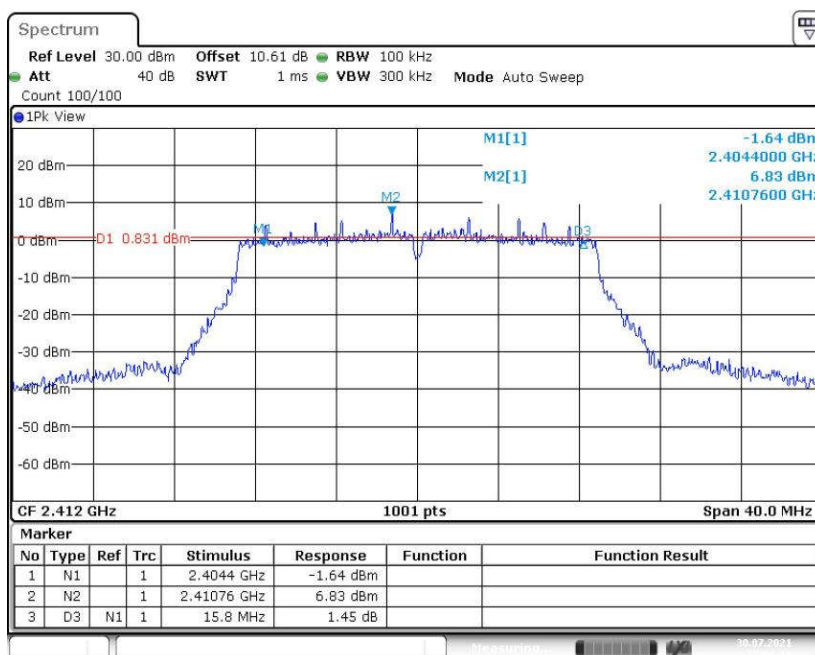
Fig.16 6dB Bandwidth (802.11n-HT20, CH 1)
