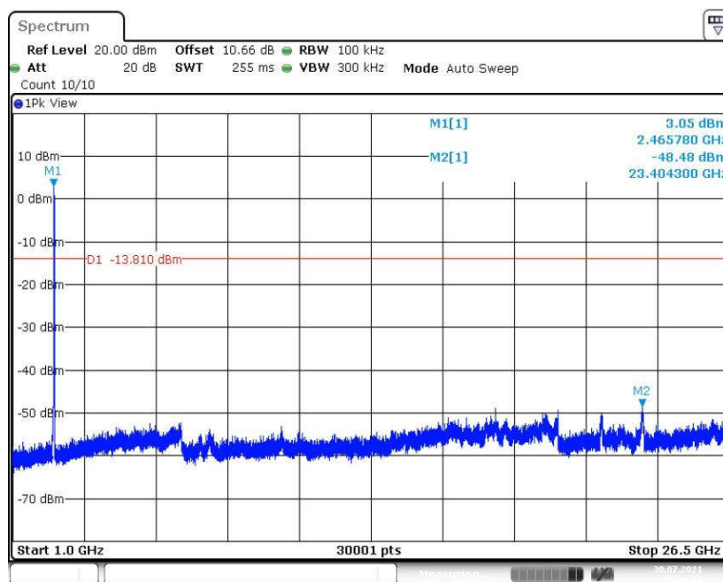
Fig.51 Conducted Spurious Emission (1GHz-26.5GHz, 802.11n-HT20, CH11)
