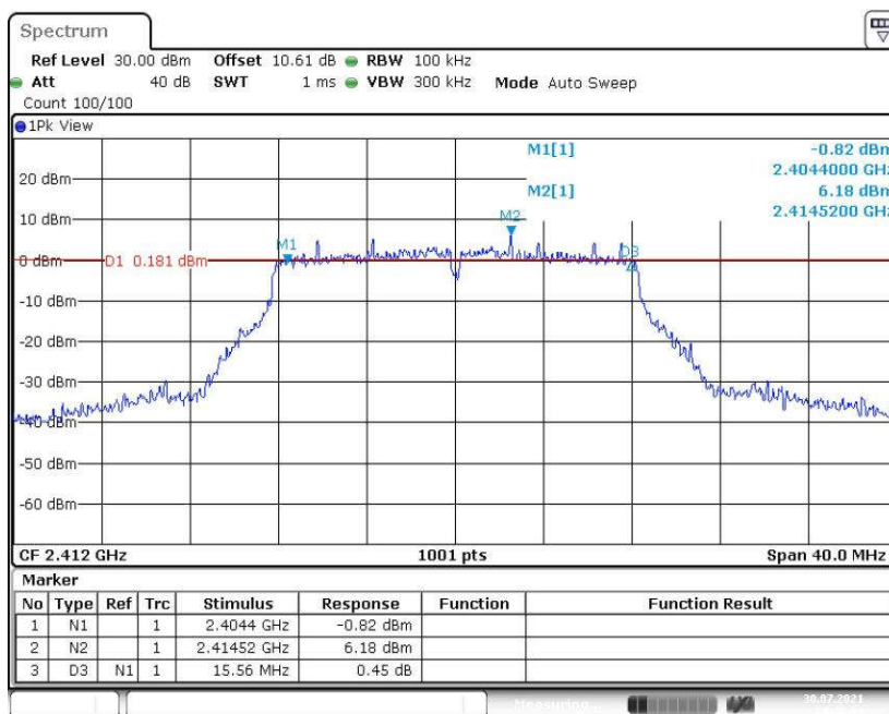
Fig.13 6dB Bandwidth (802.11g, CH 1)
