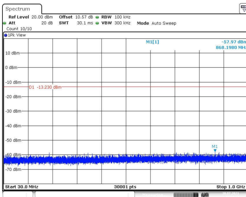
Fig.47 Conducted Spurious Emission (30MHz -1GHz, 802.11n-HT20, CH6)
