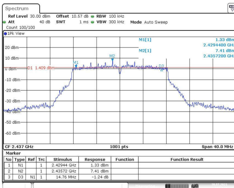
Fig.14 6dB Bandwidth (802.11g, CH 6)
