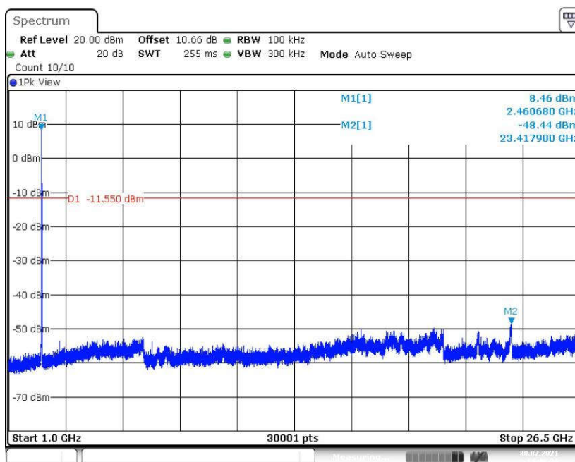
Fig.33 Conducted Spurious Emission (1GHz-26.5GHz, 802.11b, CH11)
