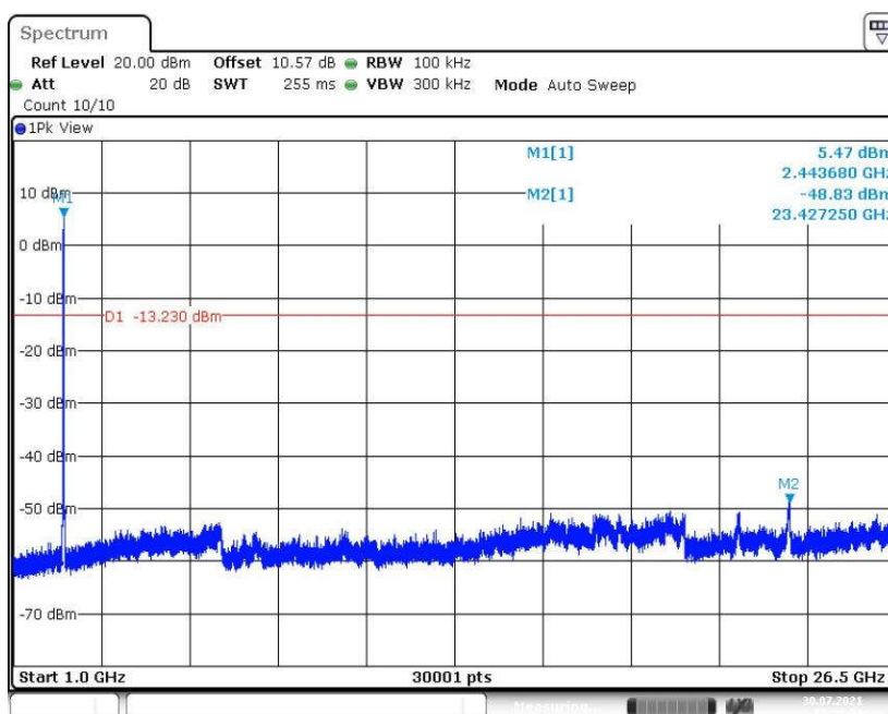
Fig.48 Conducted Spurious Emission (1GHz-26.5GHz, 802.11n-HT20, CH6)
