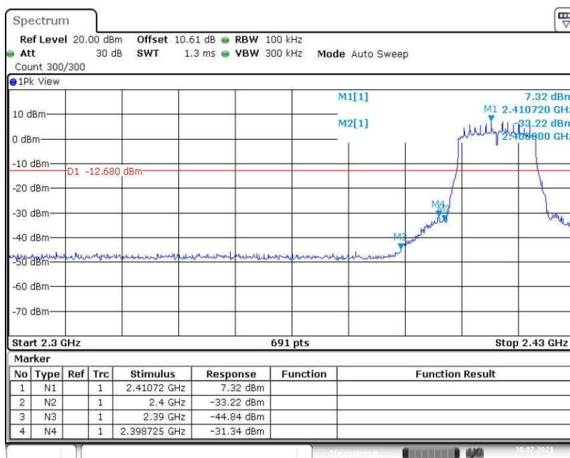
Fig.23 Band Edges (802.11n-HT20, CH 1)
