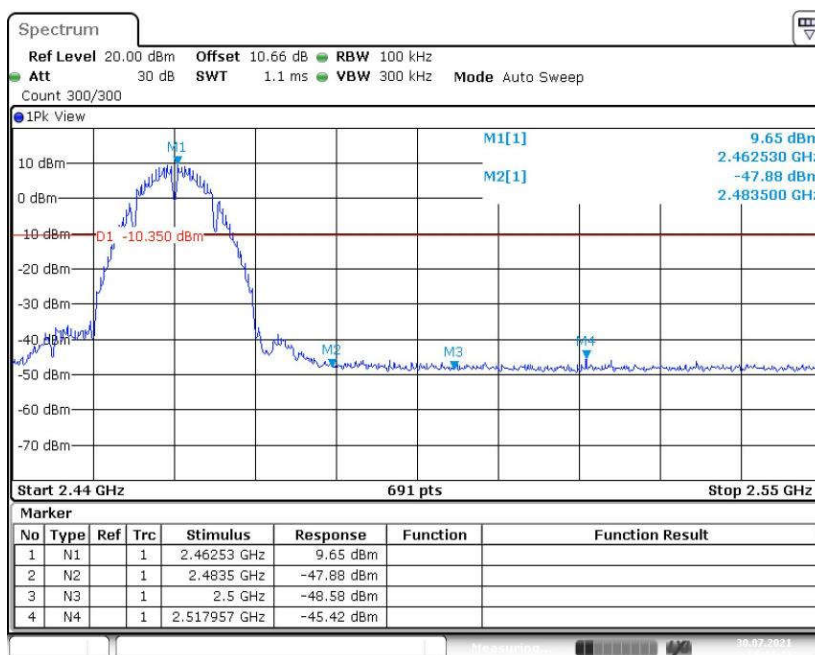
Fig.20 Band Edges (802.11b, CH 11)
