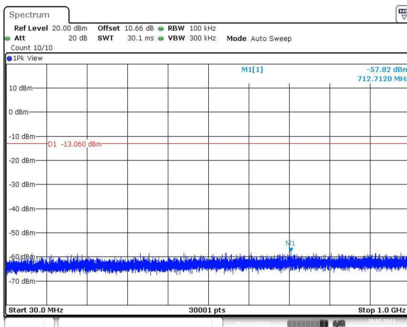
Fig.41 Conducted Spurious Emission (30MHz -1GHz, 802.11g, CH11)
