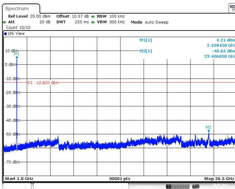
Fig.39 Conducted Spurious Emission (1GHz-26.5GHz, 802.11g, CH6)
