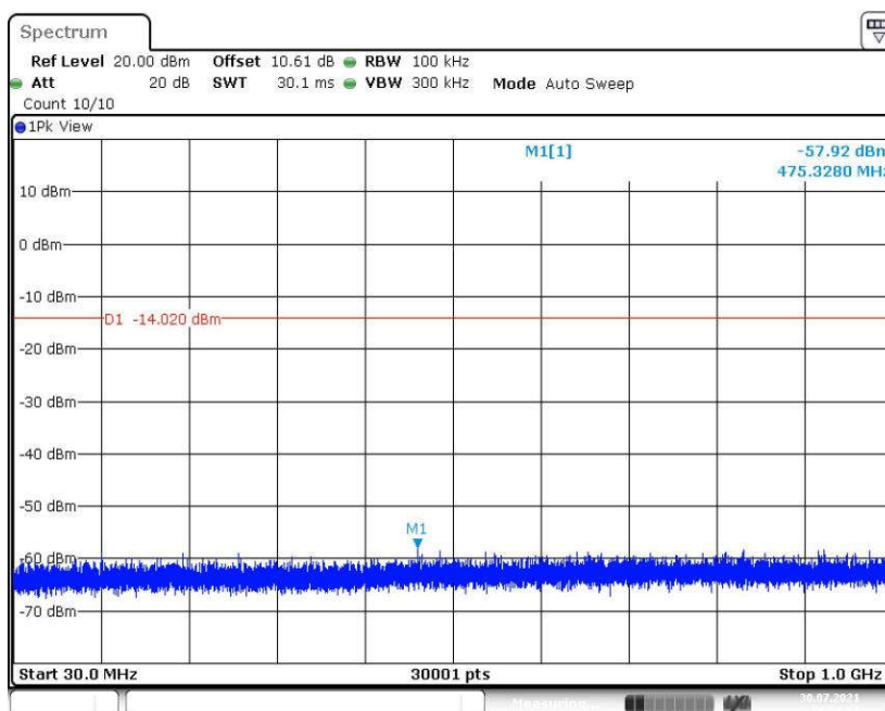
Fig.35 Conducted Spurious Emission (30MHz -1GHz, 802.11g, CH1)
