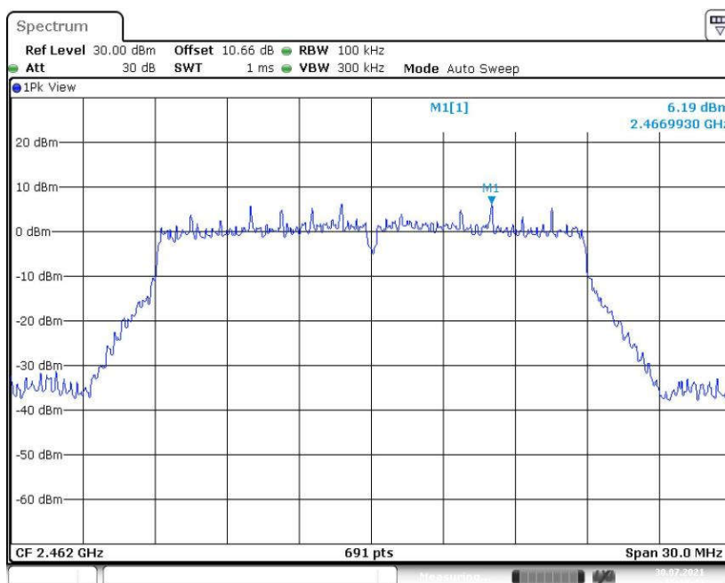
Fig.49 Conducted Spurious Emission (Center Frequency, 802.11n-HT20, CH11)
