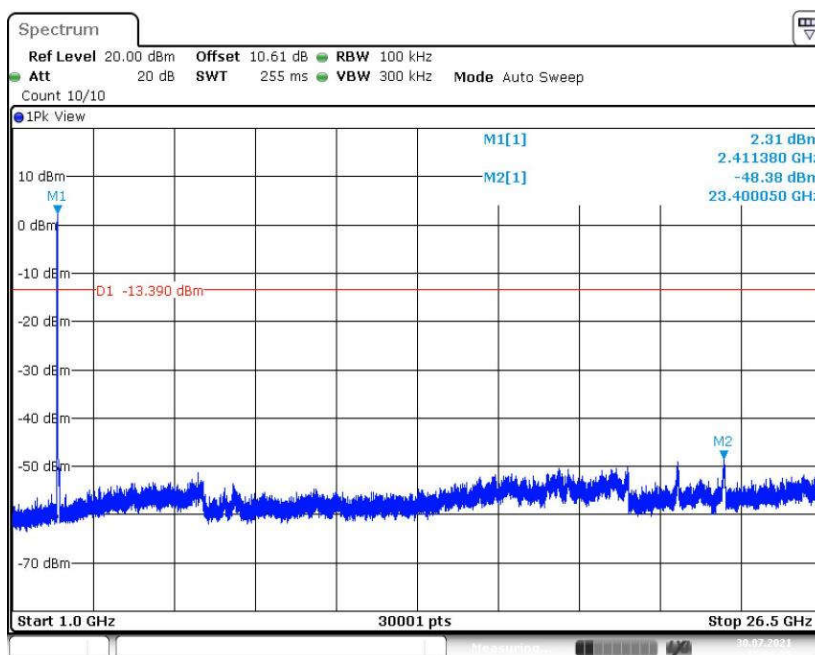
Fig.45 Conducted Spurious Emission (1GHz-26.5GHz, 802.11n-HT20, CH1)
