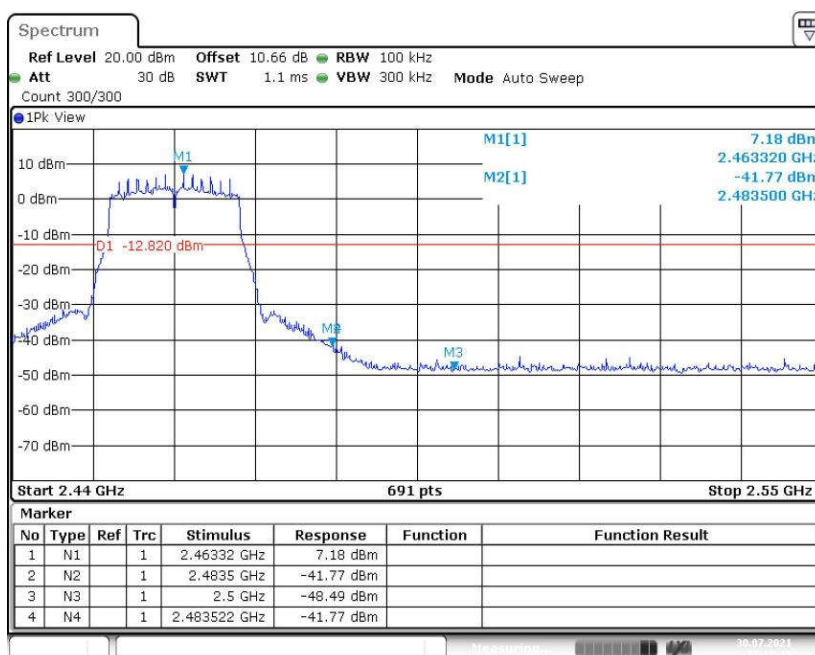
Fig.24 Band Edges (802.11n-HT20, CH 11)
