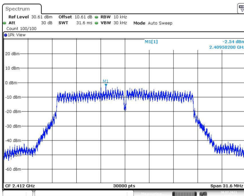
Fig.7 Power Spectral Density (802.11n-HT20, CH 1)
