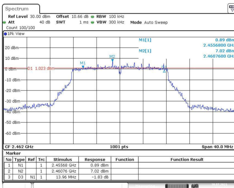
Fig.15 6dB Bandwidth (802.11g, CH 11)
