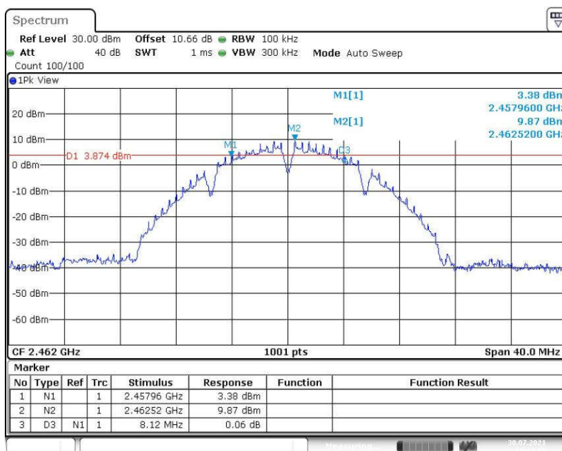
Fig.12 6dB Bandwidth (802.11b, CH 11)
