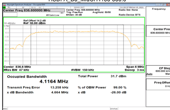
HSDPA_B5_MidCH4183-836.6
