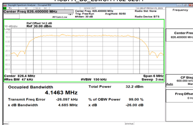
HSDPA_B5_LowCH4132-826.4
