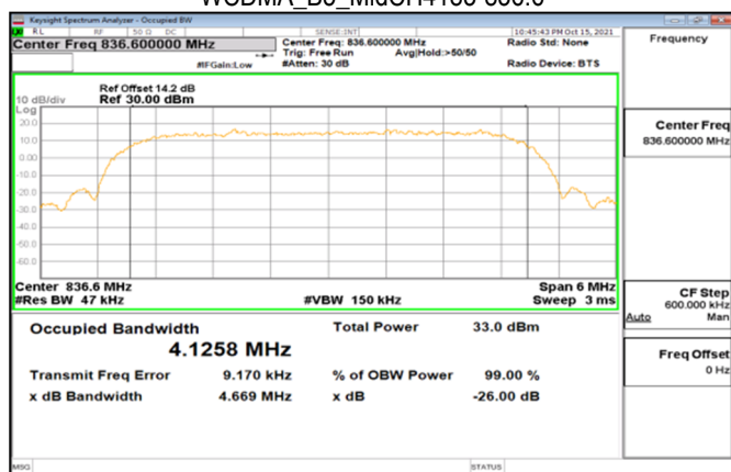
WCDMA_B5_MidCH4183-836.6
