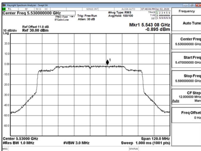
802.11ax_80MHz_RU_484_65_5530MHz-5530
