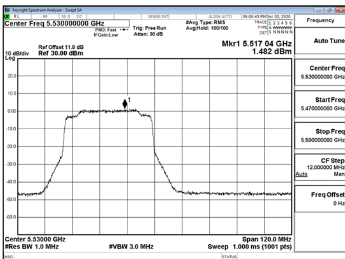
802.11ax_80MHz_RU_484_65_5530MHz-5530
