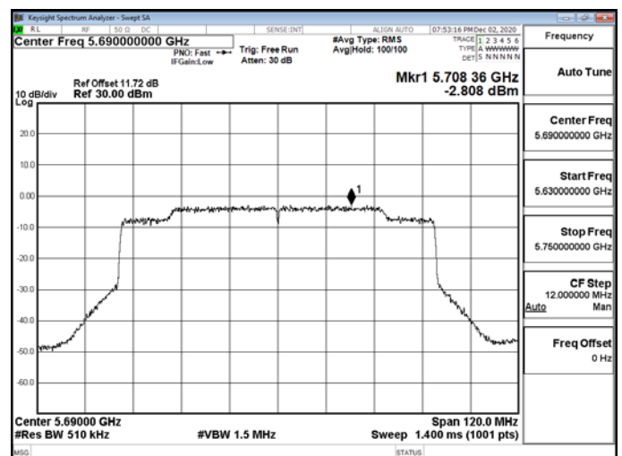
802.11ax_80MHz_5690MHz_UNII 3
