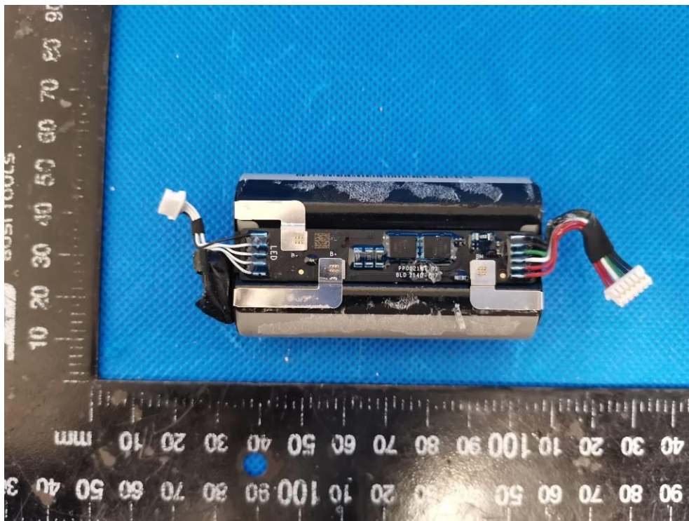
Photo- 06 PCB view-01 of battery
