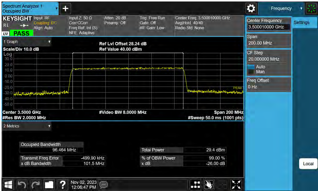
Sub6 n77(78). Occupied Bandwidth Plot (100 M BW Ch.633334 64QAM )
