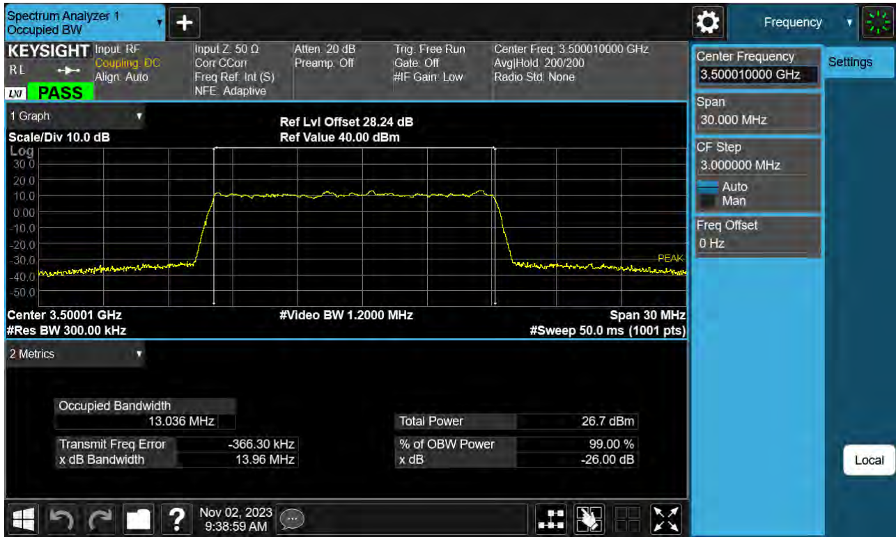
Sub6 n77(78). Occupied Bandwidth Plot (15 M BW Ch.633334 256QAM )
