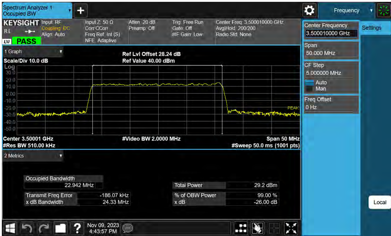
Sub6 n77(78). Occupied Bandwidth Plot (25 M BW Ch.633334 64QAM )
