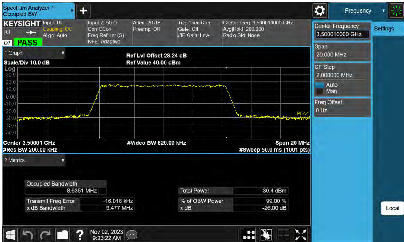
Sub6 n77(78). Occupied Bandwidth Plot (10 M BW Ch.633334 QPSK )
