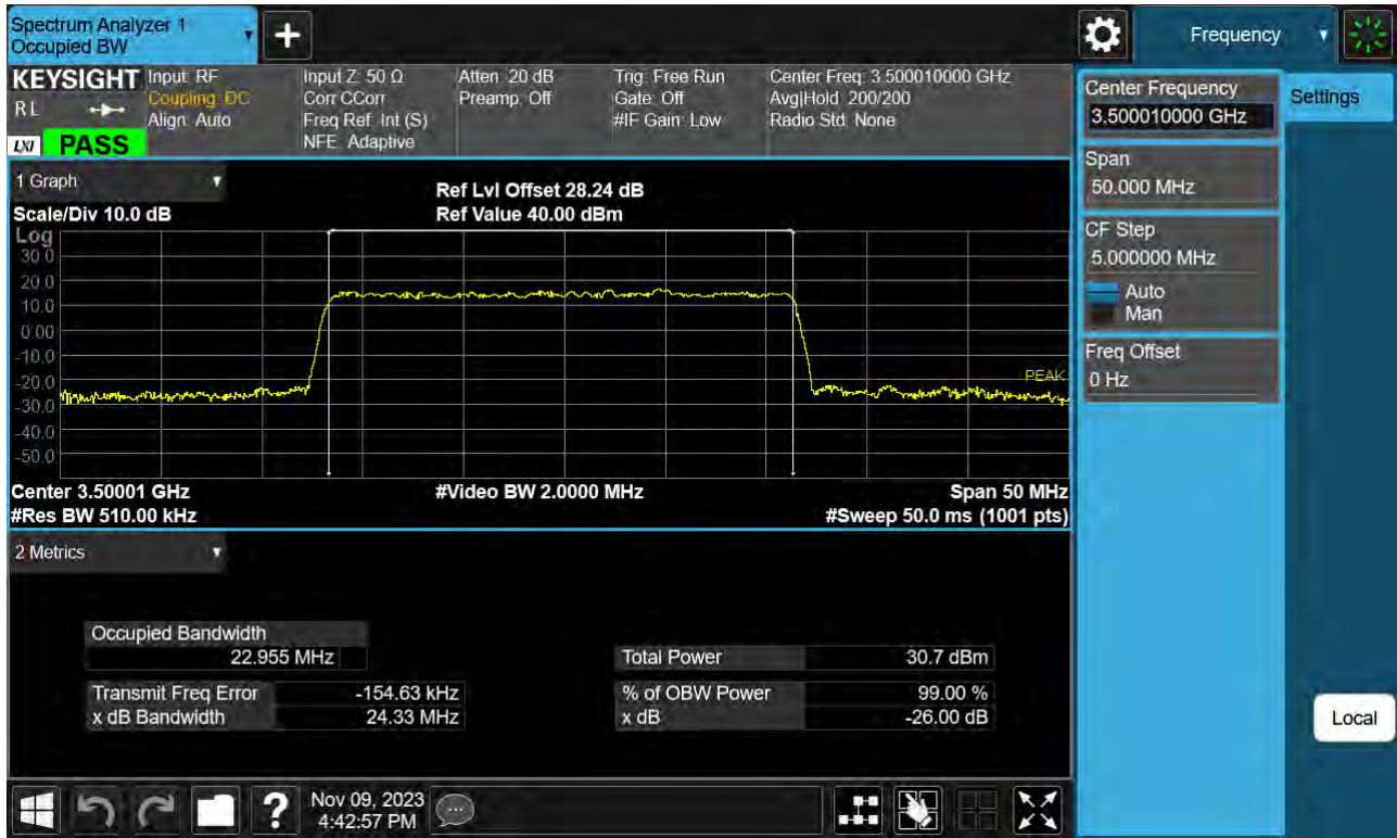
Sub6 n77(78). Occupied Bandwidth Plot (25 M BW Ch.633334 QPSK )
