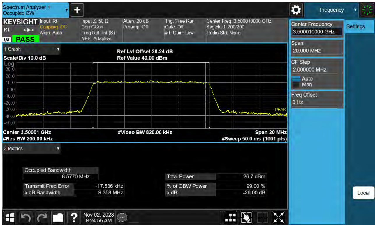
Sub6 n77(78). Occupied Bandwidth Plot (10 M BW Ch.633334 256QAM )
