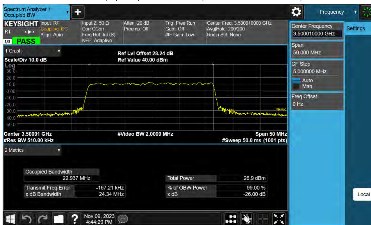
Sub6 n77(78). Occupied Bandwidth Plot (25 M BW Ch.633334 256QAM )
