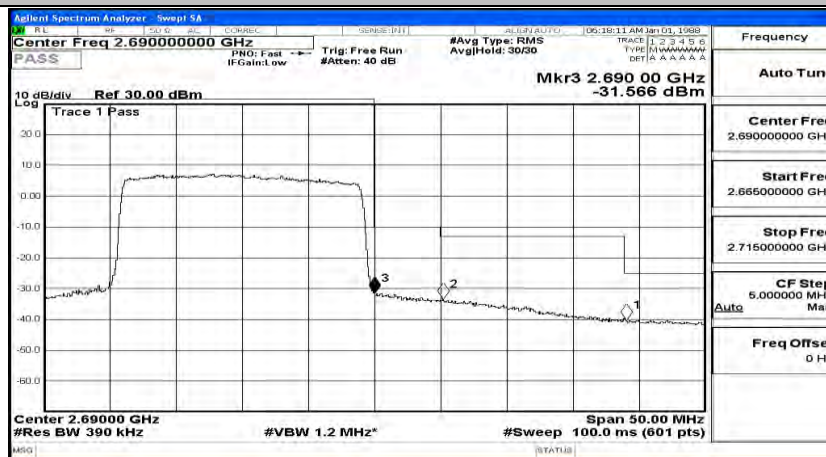
Band Edge Test Graph(s) (Channel Bandwidth:20 MHz)_HCH_16QAM
