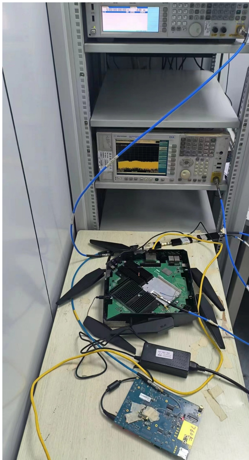
Picture 1 DFS Test Setup
