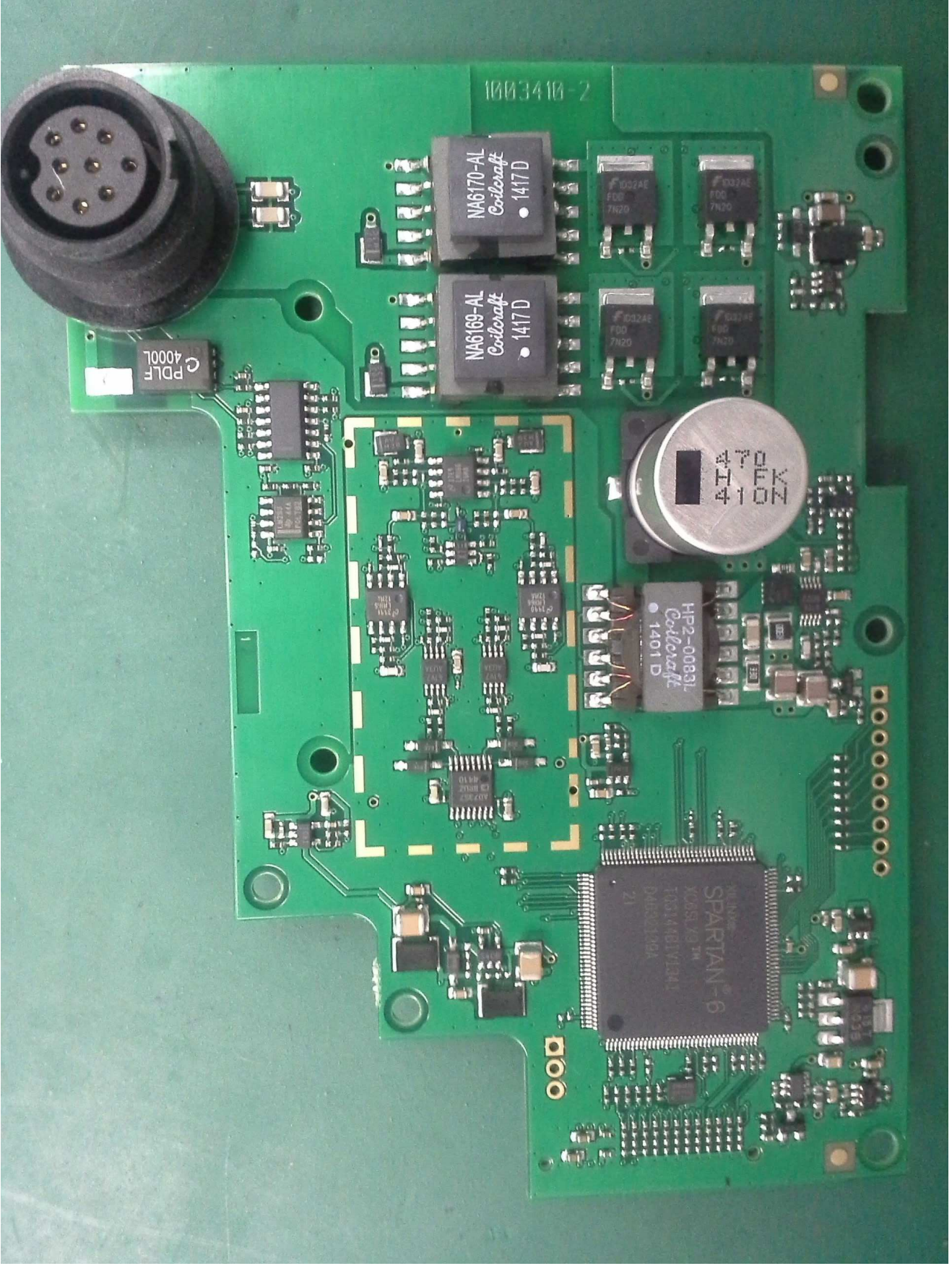
Figure 5 - DOWNVISION_PCBA_TOP
