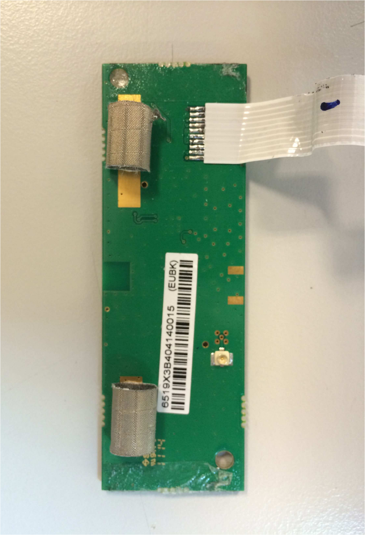
Figure 6 - GPS_PCBA_BOTTOM
