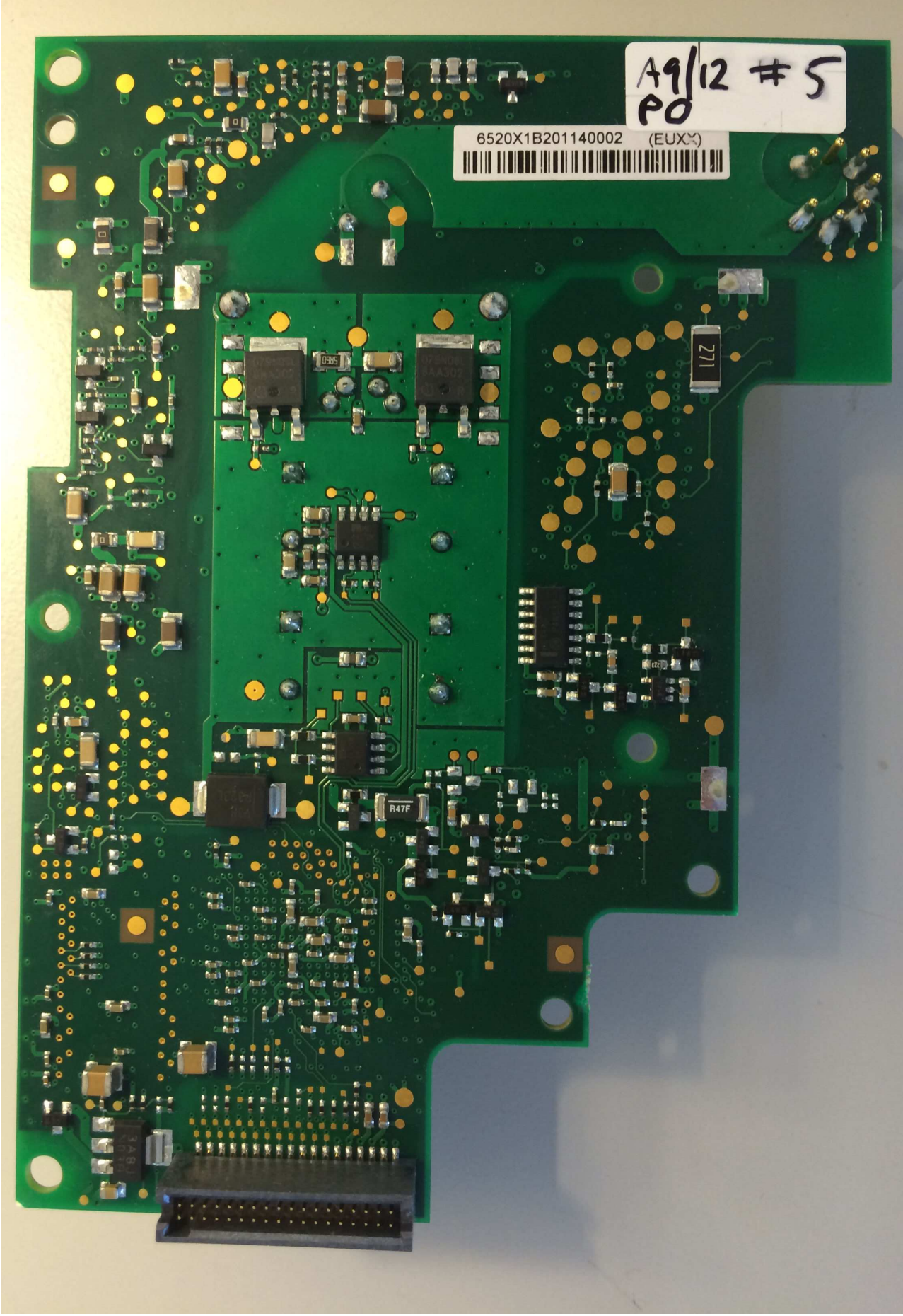
Figure 10 - SONAR_PCBA_BOTTOM
