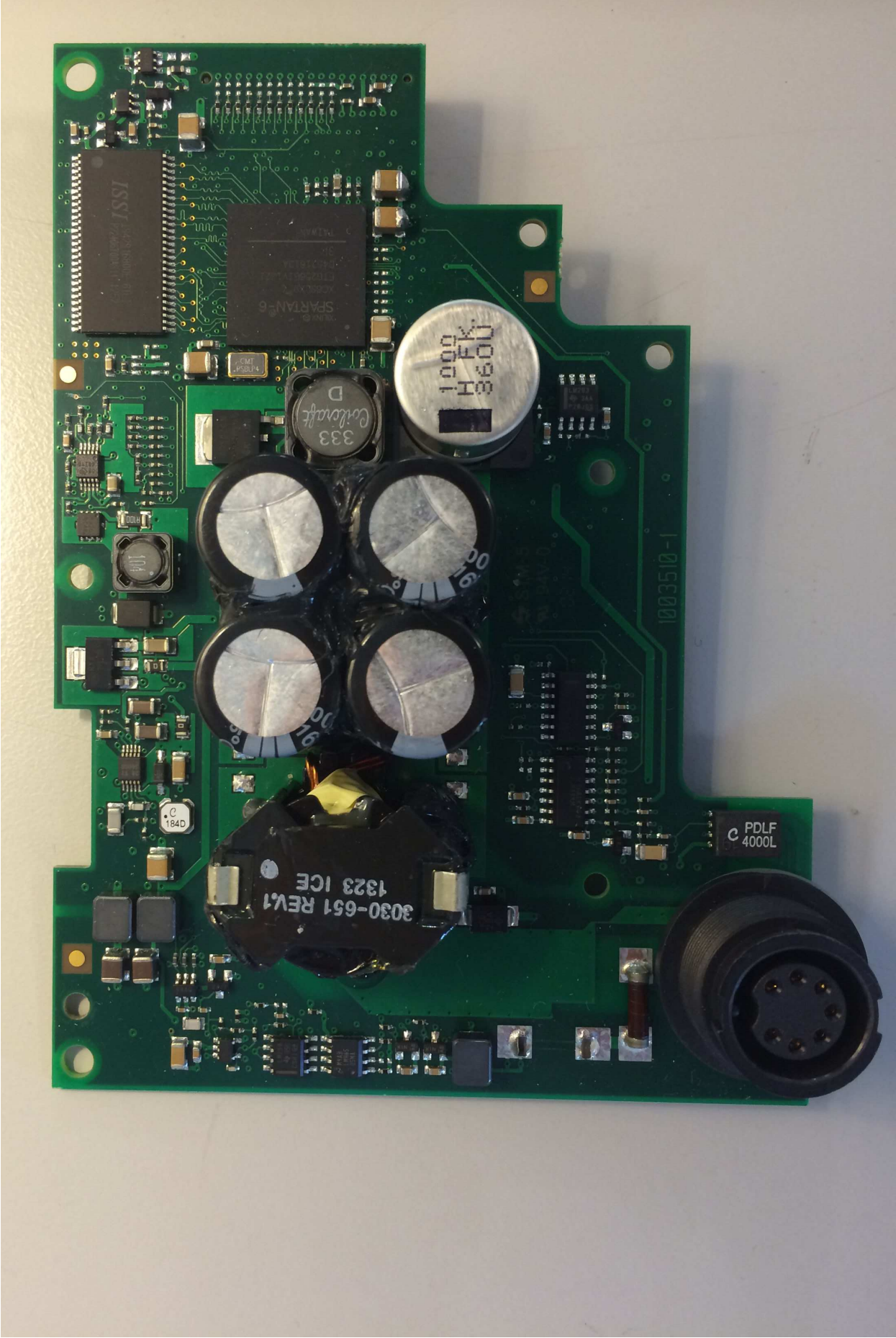
Figure 11 - SONAR_PCBA_TOP
