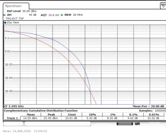
Band38-10MHz-16QAM-38200-50RB#0
