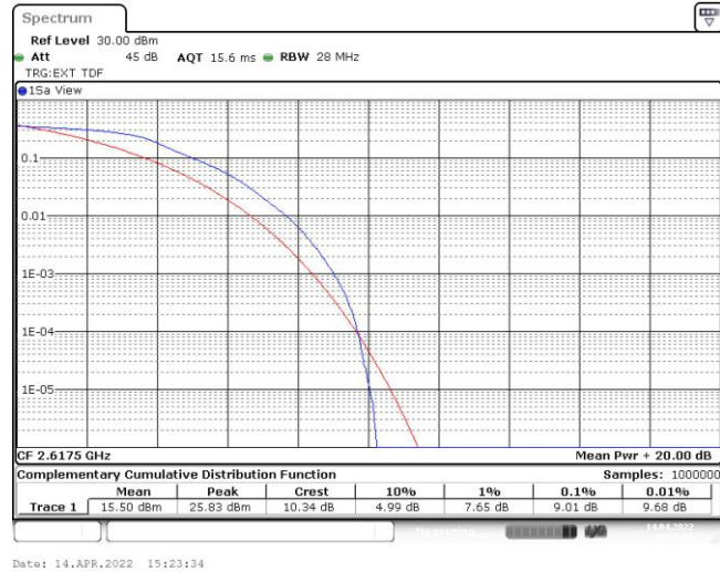
Band38-5MHz-16QAM-37775-25RB#0
