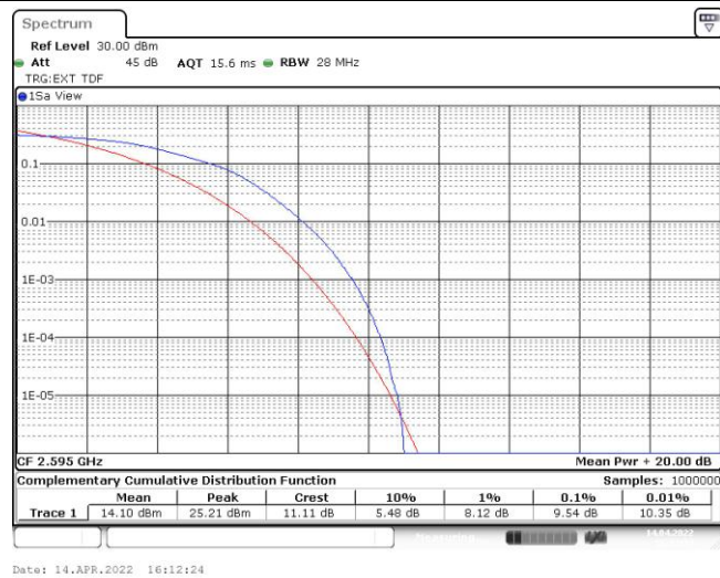
Band38-20MHz-16QAM-38150-100RB#0
