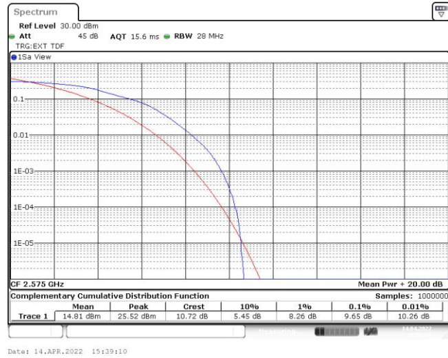
Band38-10MHz-16QAM-38000-50RB#0
