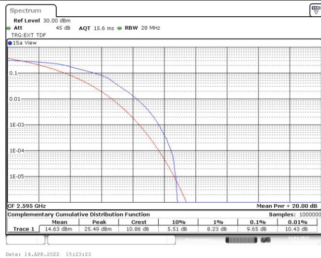
Band38-5MHz-16QAM-38225-25RB#0
