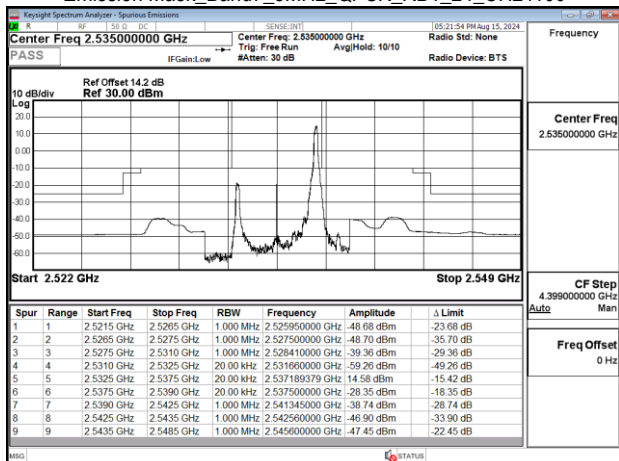
Emission Mask_Band7_5MHz_QPSK_RB1_24_CH21100
