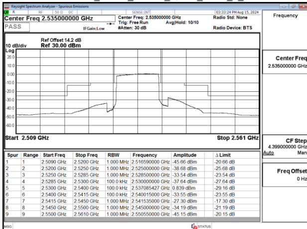
Emission Mask_Band7_10MHz_QPSK_RB50_0_CH21100
