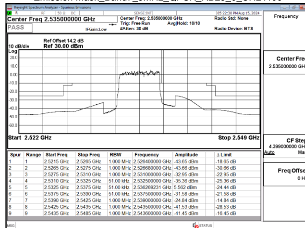
Emission Mask_Band7_5MHz_QPSK_RB25_0_CH21100
