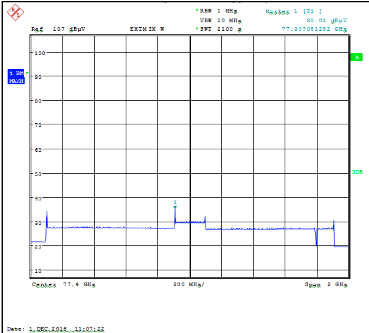
Plot 4-1: Radiated Fundamental (EIRP in 1 MHz)
