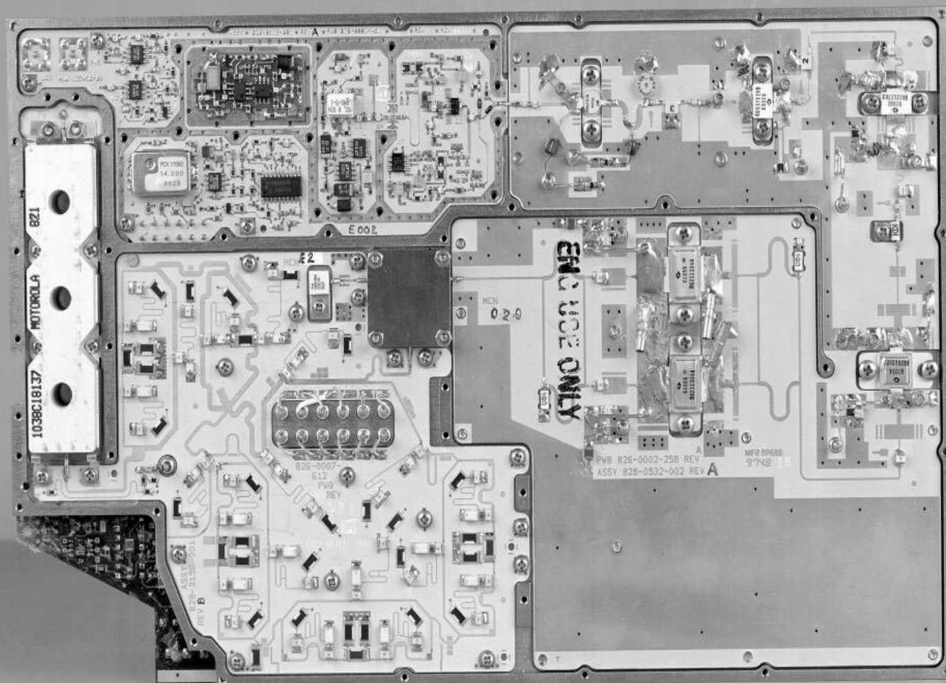
Transmitter Module
