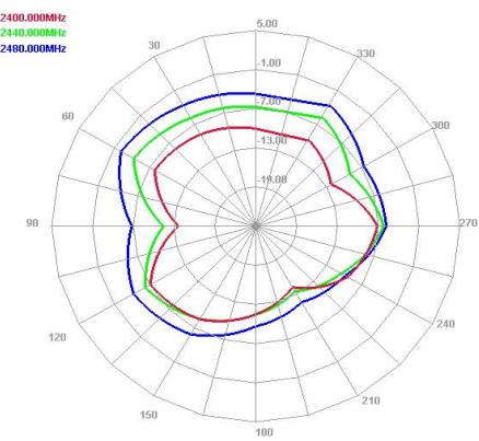
Horizontal
