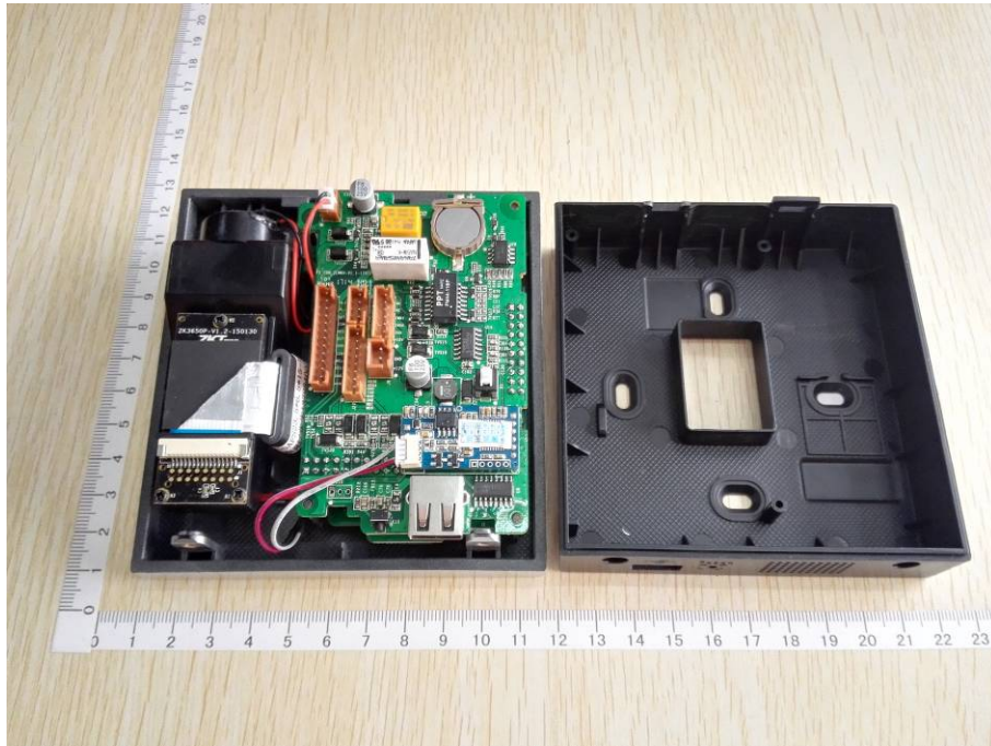
Internal photos for 125KHz Module
