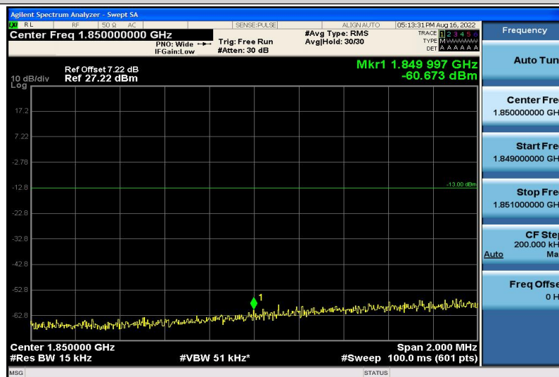
Band2-10MHz-16QAM-18650-1RB#5
