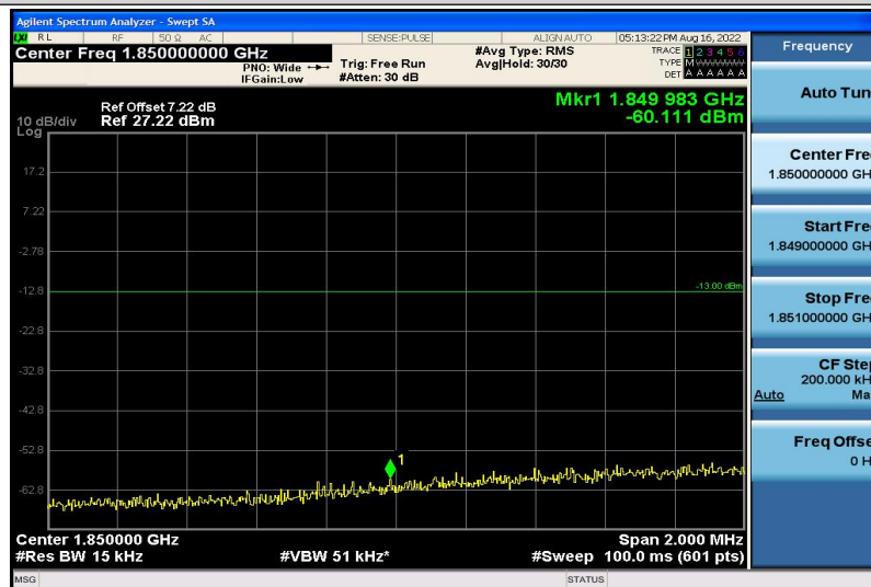
Band2-10MHz-QPSK-18650-1RB#5
