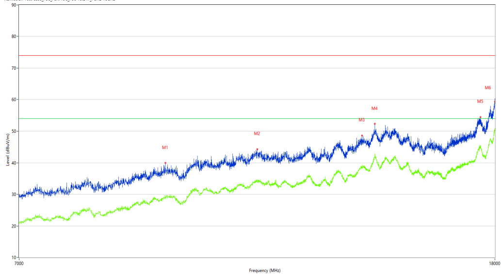
REmission Test case_FCC_Part 15C_FCC 15.247 /GHz-18GHz
