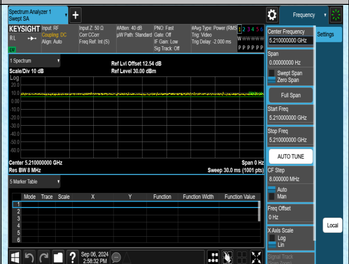
NTNV-11AC80MIMO-Ant4-5210
