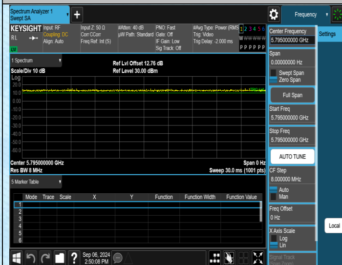
NTNV-11AC40MIMO-Ant3-5795
