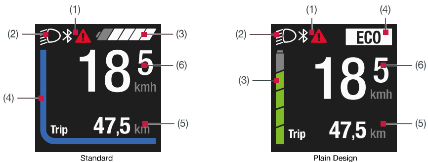
Fig. 2: User interface
