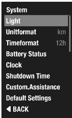
Fig. 9: Settings System
