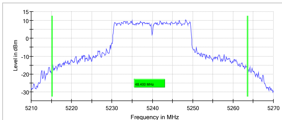
26 dB Bandwidth
