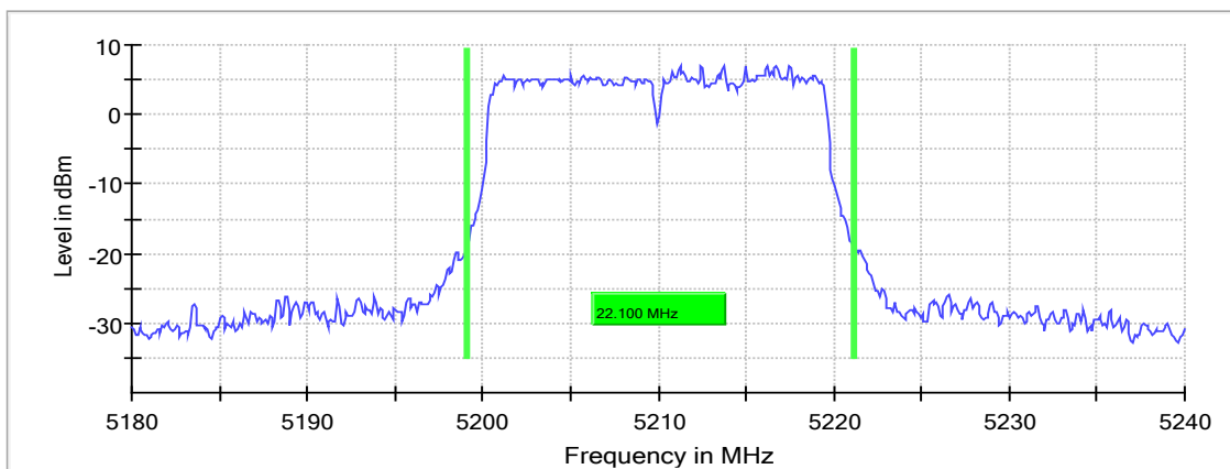
Bandwidth
