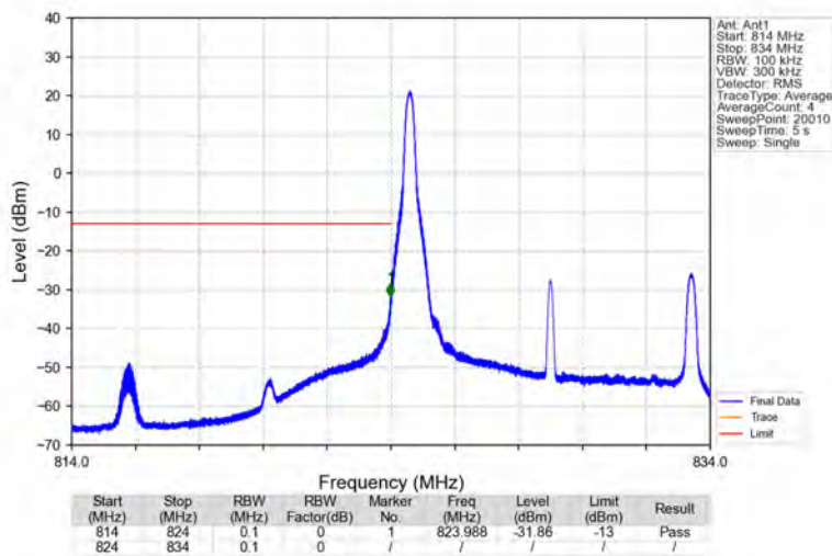
Band5_10MHz_16QAM_LCH_829MHz_RB_1_0_NTNV
