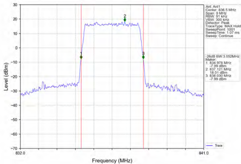
Band5_3MHz_16QAM_MCH_836.5MHz_RB_15_0_NTNV
