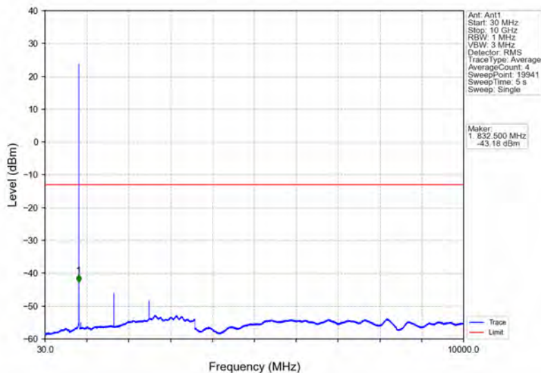
Band5_1.4MHz_QPSK_MCH_836.5MHz_RB_1_0_NTNV
