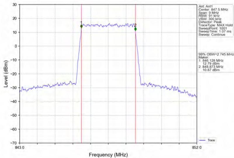
Band5_3MHz_64QAM_HCH_847.5MHz_RB_15_0_NTNV
