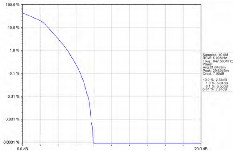
Band5_3MHz_16QAM_HCH_847.5MHz_RB_15_0_NTNV
