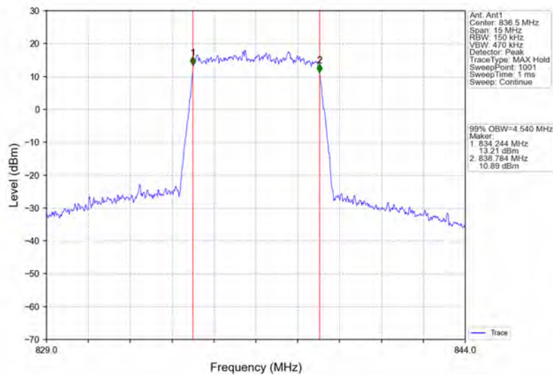
Band5_5MHz_64QAM_MCH_836.5MHz_RB_25_0_NTNV
