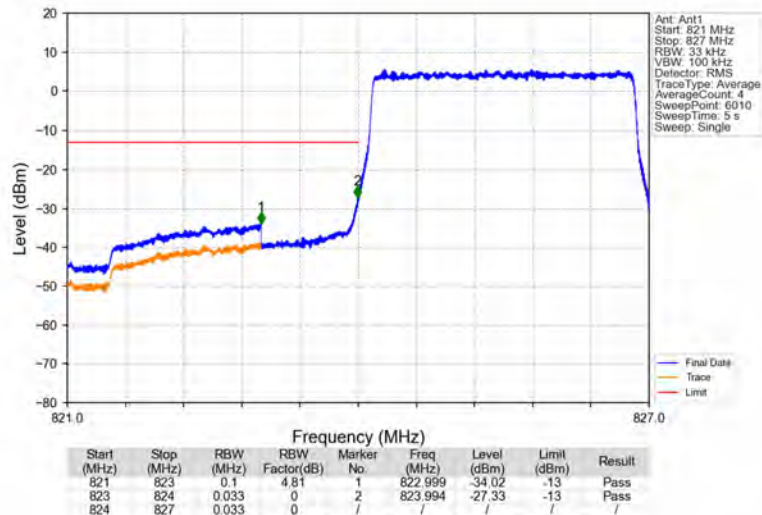
Band5_3MHz_QPSK_LCH_825.5MHz_RB_15_0_NTNV
