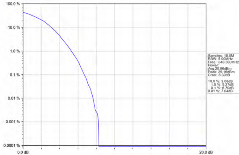
Band5_1.4MHz_64QAM_HCH_848.3MHz_RB_6_0_NTNV
