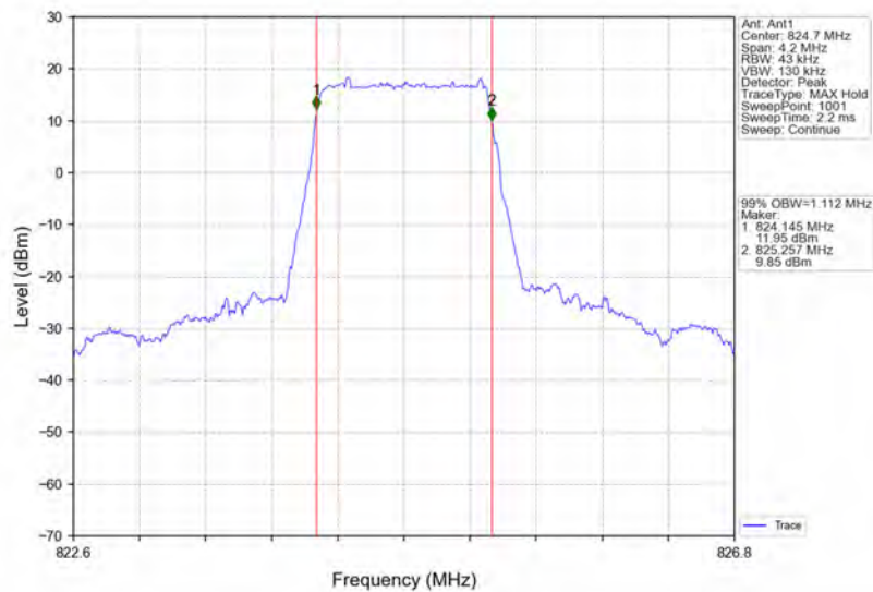
Band5_1.4MHz_16QAM_LCH_824.7MHz_RB_6_0_NTNV
