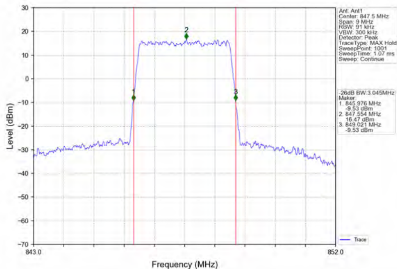
Band5_3MHz_64QAM_HCH_847.5MHz_RB_15_0_NTNV
