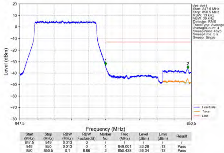
Band5_1.4MHz_QPSK_HCH_848.3MHz_RB_6_0_NTNV
