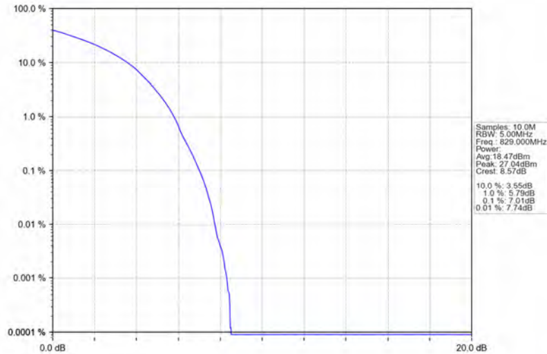
Band5_10MHz_64QAM_LCH_829MHz_RB_50_0_NTNV
