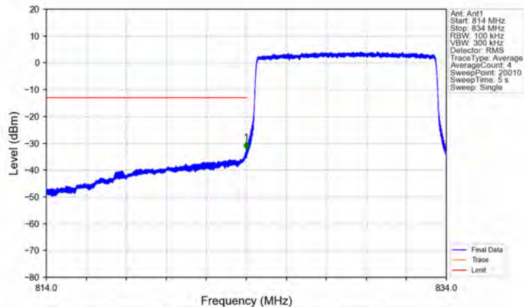
Band5_10MHz_16QAM_LCH_829MHz_RB_50_0_NTNV
