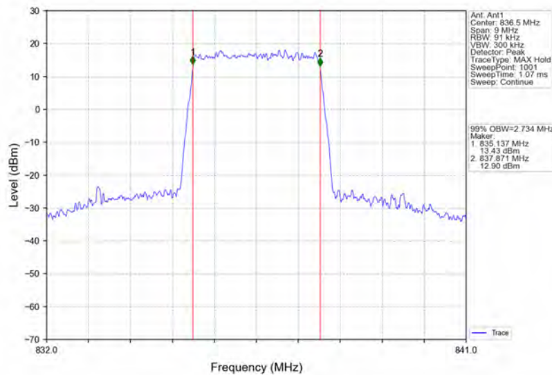
Band5_3MHz_16QAM_MCH_836.5MHz_RB_15_0_NTNV
