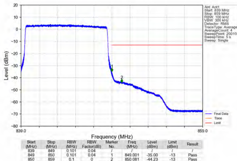
Band5_10MHz_16QAM_HCH_844MHz_RB_50_0_NTNV
