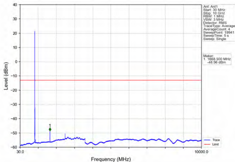
Band5_5MHz_64QAM_MCH_836.5MHz_RB_1_0_NTNV
