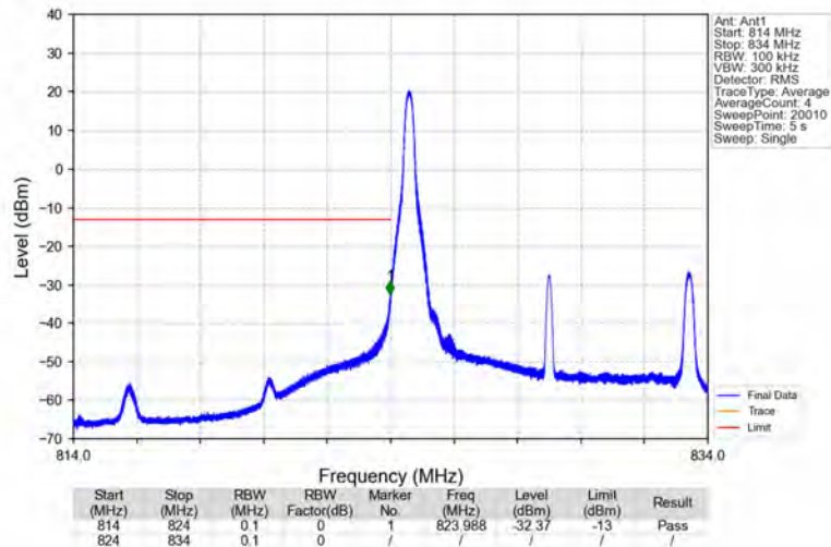
Band5_10MHz_64QAM_LCH_829MHz_RB_1_0_NTNV
