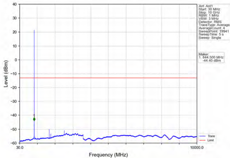
Band5_1.4MHz_64QAM_HCH_848.3MHz_RB_1_5_NTNV
