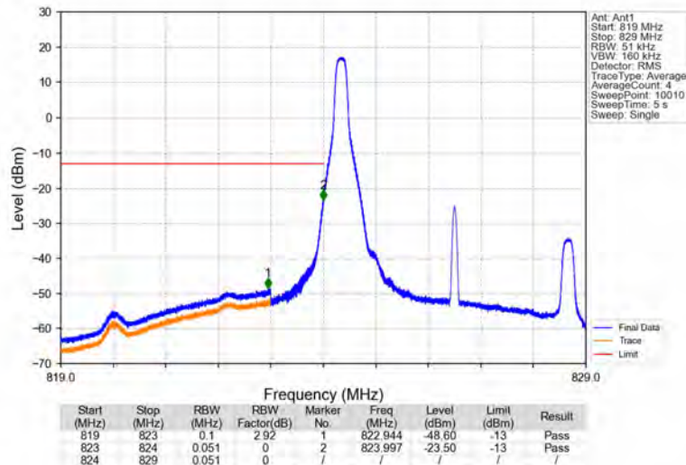
Band5_5MHz_64QAM_LCH_826.5MHz_RB_1_0_NTNV
