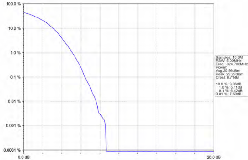
Band5_1.4MHz_64QAM_LCH_824.7MHz_RB_6_0_NTNV
