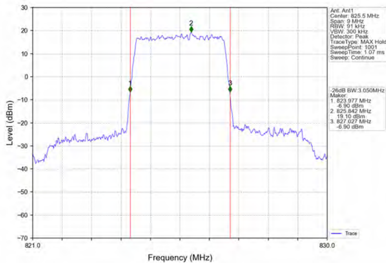
Band5_3MHz_QPSK_LCH_825.5MHz_RB_15_0_NTNV
