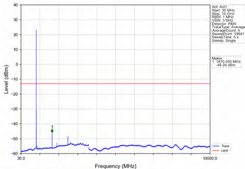
Band5_3MHz_QPSK_MCH_836.5MHz_RB_1_0_NTNV
