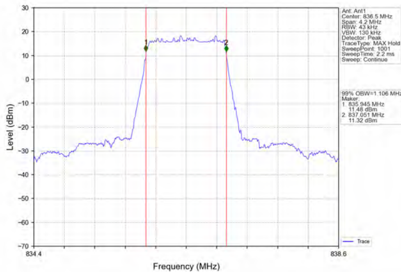
Band5_1.4MHz_64QAM_MCH_836.5MHz_RB_6_0_NTNV
