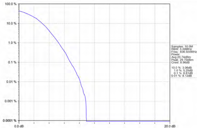
Band5_1.4MHz_64QAM_MCH_836.5MHz_RB_6_0_NTNV
