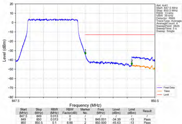
Band5_1.4MHz_16QAM_HCH_848.3MHz_RB_6_0_NTNV
