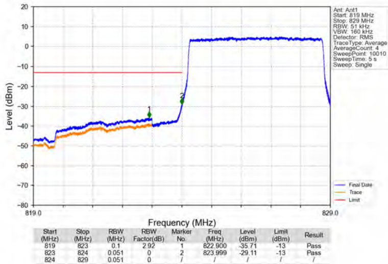
Band5_5MHz_QPSK_LCH_826.5MHz_RB_25_0_NTNV
