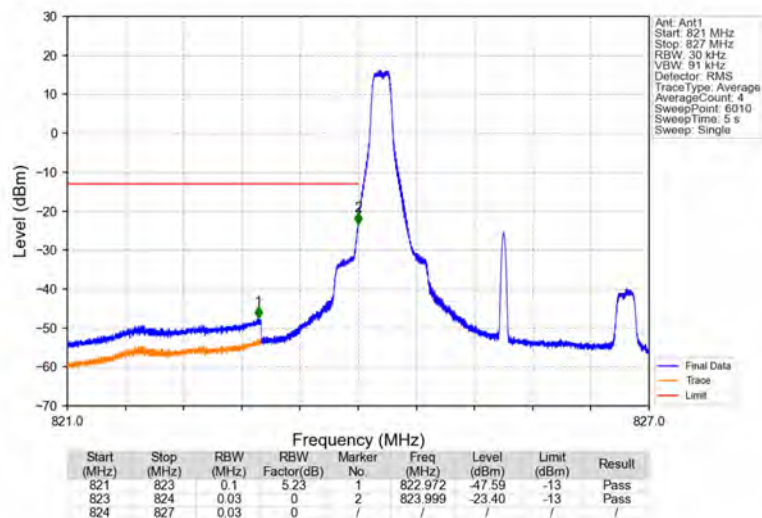
Band5_3MHz_16QAM_LCH_825.5MHz_RB_1_0_NTNV
