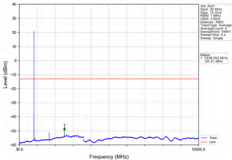
Band5_3MHz_64QAM_HCH_847.5MHz_RB_1_14_NTNV
