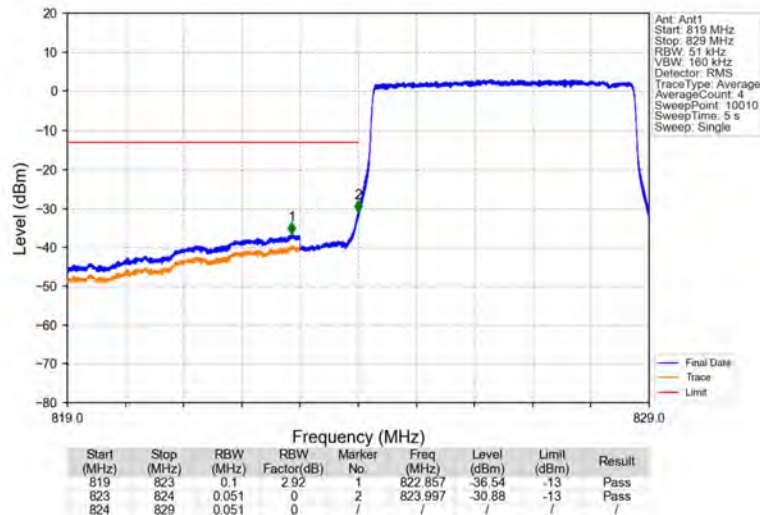
Band5_5MHz_64QAM_LCH_826.5MHz_RB_25_0_NTNV
