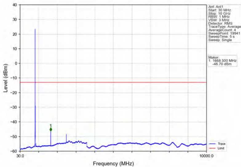
Band5_5MHz_QPSK_MCH_836.5MHz_RB_1_0_NTNV
