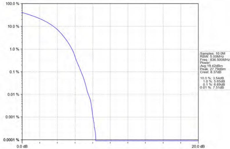
Band5_10MHz_16QAM_MCH_836.5MHz_RB_50_0_NTNV
