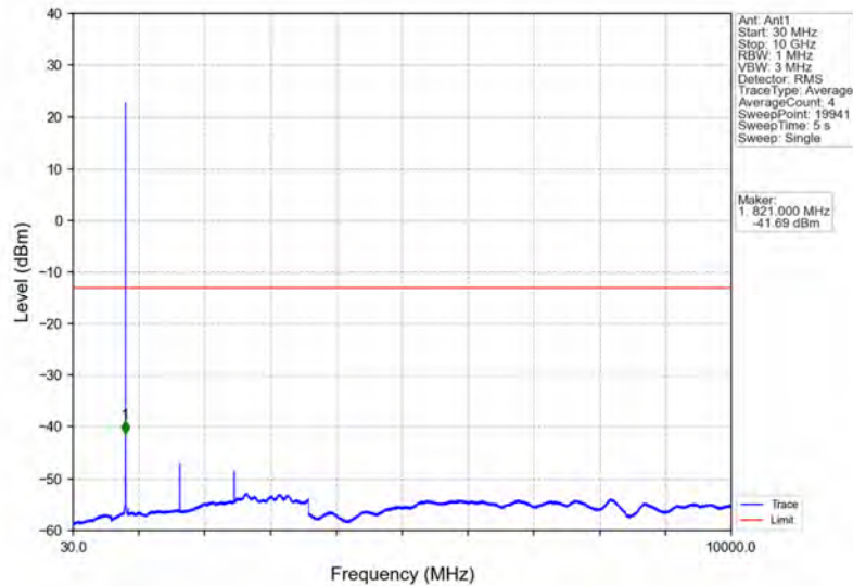
Band5_1.4MHz_16QAM_LCH_824.7MHz_RB_6_0_NTNV
