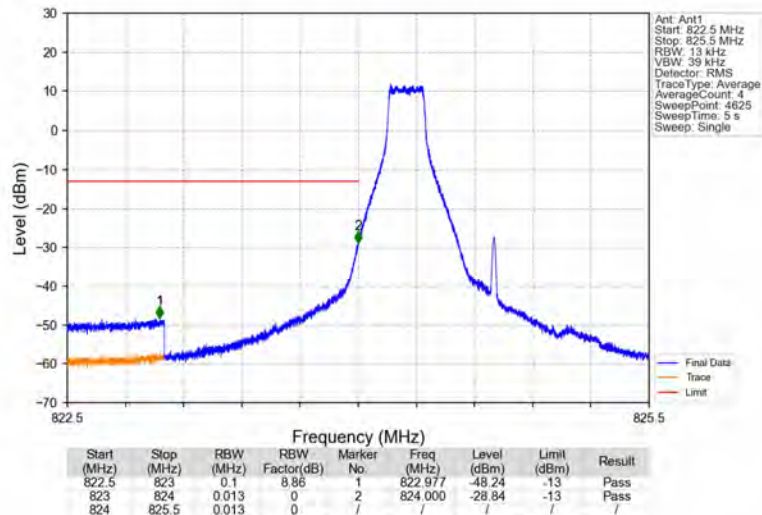
Band5_1.4MHz_64QAM_LCH_824.7MHz_RB_1_0_NTNV
