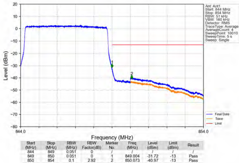
Band5_5MHz_64QAM_HCH_846.5MHz_RB_25_0_NTNV
