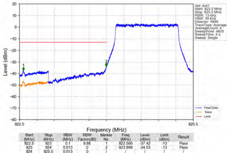
Band5_1.4MHz_64QAM_LCH_824.7MHz_RB_6_0_NTNV
