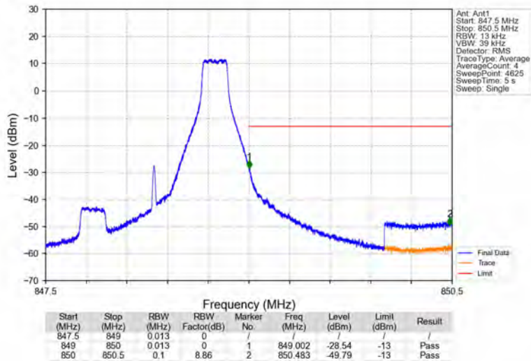
Band5_1.4MHz_16QAM_HCH_848.3MHz_RB_1_5_NTNV
