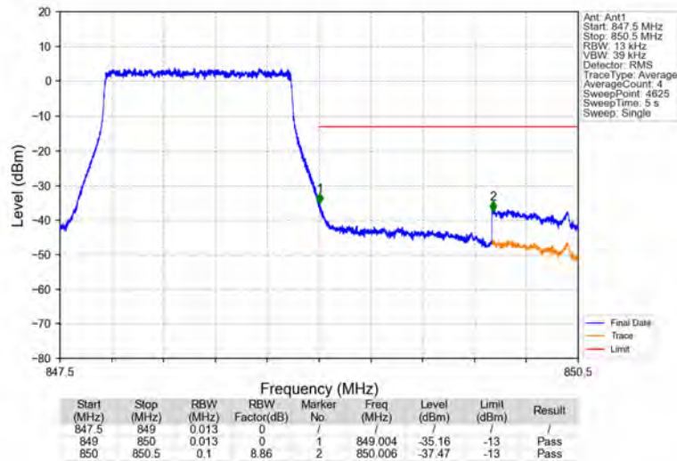
Band5_1.4MHz_64QAM_HCH_848.3MHz_RB_6_0_NTNV
