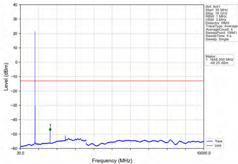
Band5_5MHz_64QAM_LCH_826.5MHz_RB_1_0_NTNV
