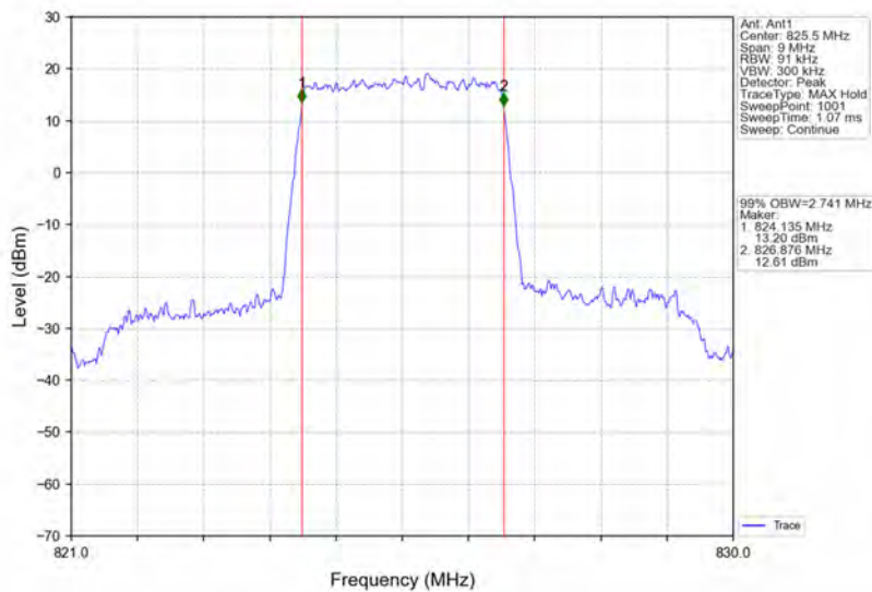
Band5_3MHz_QPSK_LCH_825.5MHz_RB_15_0_NTNV
