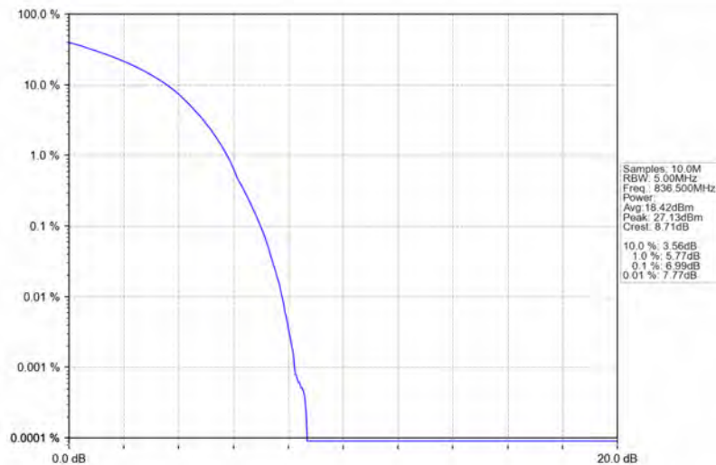
Band5_10MHz_64QAM_MCH_836.5MHz_RB_50_0_NTNV
