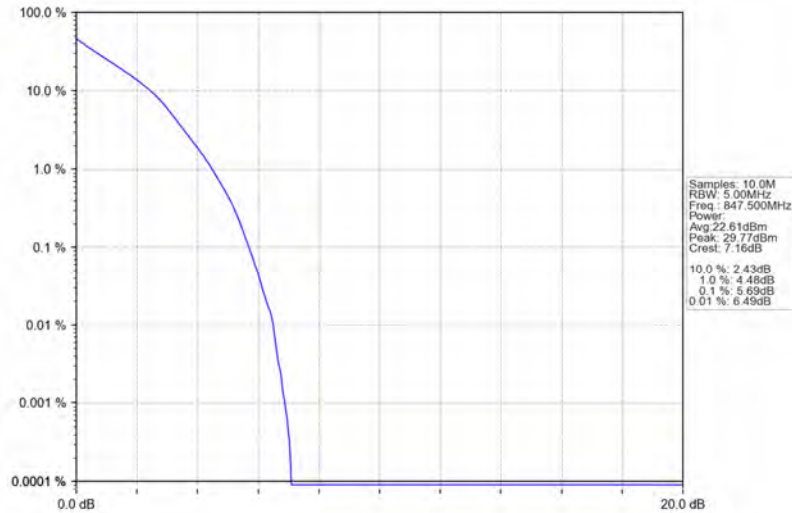
Band5_3MHz_QPSK_HCH_847.5MHz_RB_15_0_NTNV
