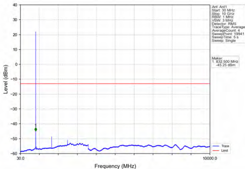
Band5_1.4MHz_64QAM_MCH_836.5MHz_RB_1_0_NTNV
