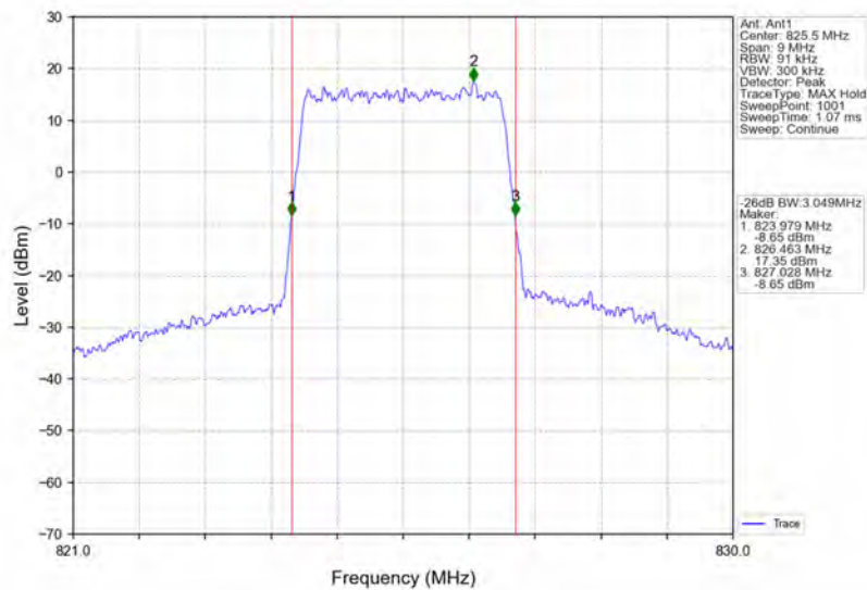
Band5_3MHz_64QAM_LCH_825.5MHz_RB_15_0_NTNV
