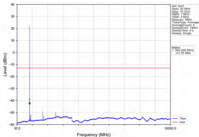
Band5_1.4MHz_16QAM_HCH_848.3MHz_RB_1_0_NTNV
