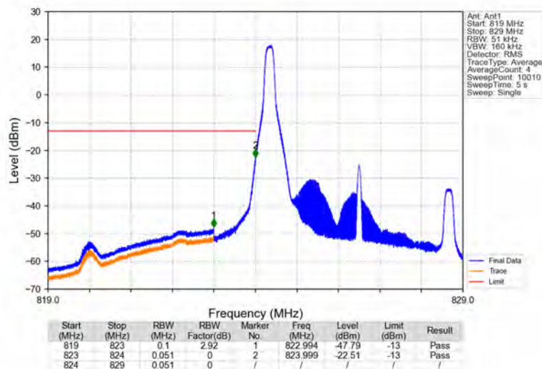
Band5_5MHz_16QAM_LCH_826.5MHz_RB_1_0_NTNV
