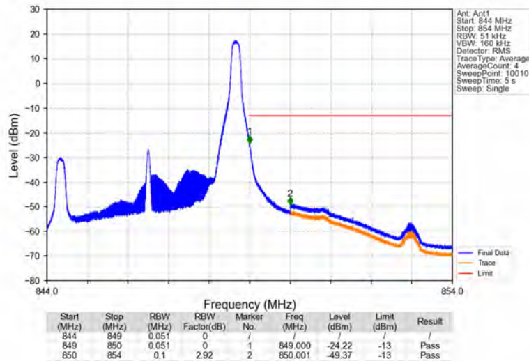
Band5_5MHz_16QAM_HCH_846.5MHz_RB_1_24_NTNV
