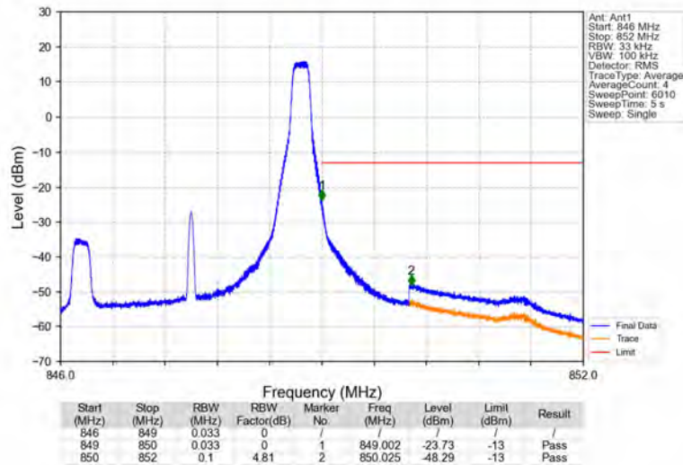
Band5_3MHz_16QAM_HCH_847.5MHz_RB_1_14_NTNV
