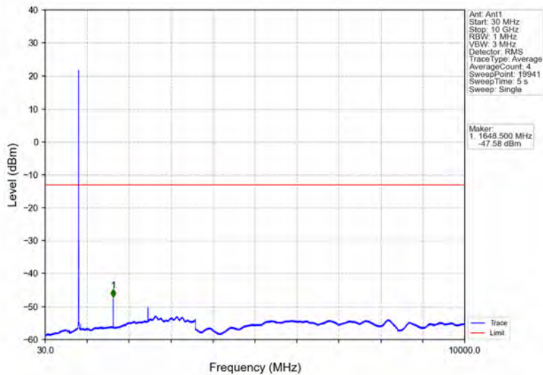
Band5_3MHz_16QAM_LCH_825.5MHz_RB_15_0_NTNV
