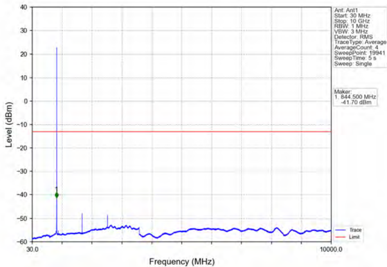
Band5_1.4MHz_QPSK_HCH_848.3MHz_RB_1_5_NTNV
