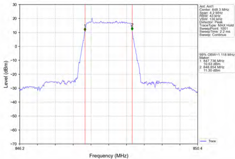
Band5_1.4MHz_16QAM_HCH_848.3MHz_RB_6_0_NTNV
