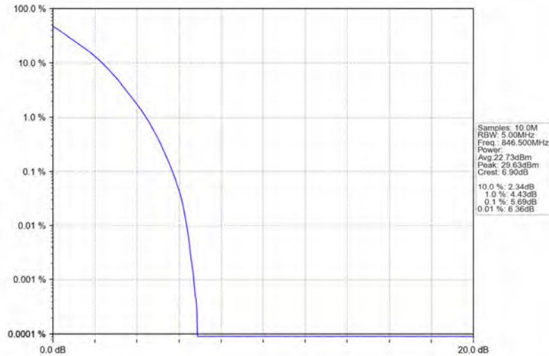
Band5_5MHz_QPSK_HCH_846.5MHz_RB_25_0_NTNV
