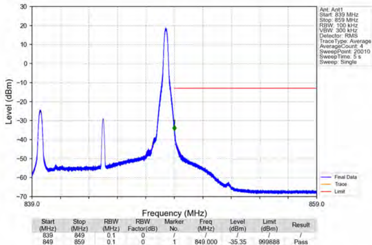
Band5_10MHz_64QAM_HCH_844MHz_RB_1_49_NTNV
