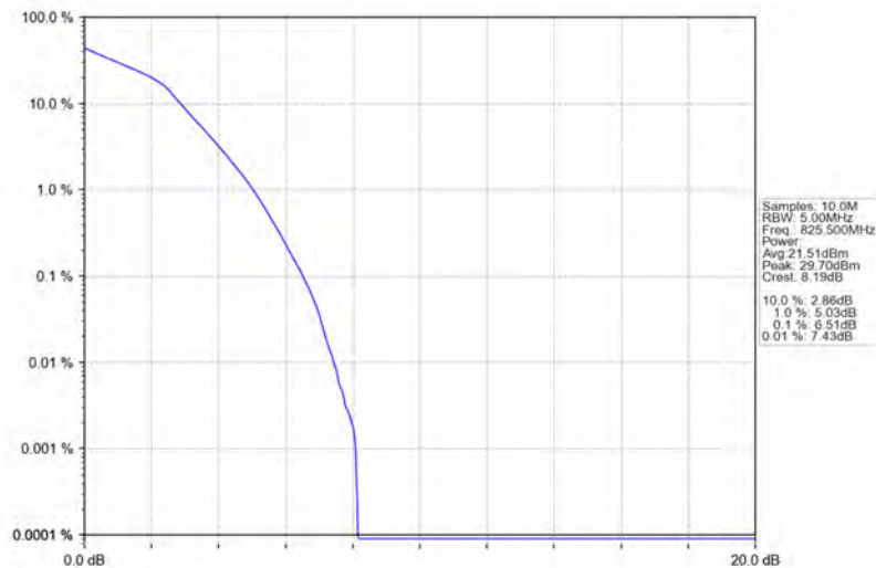
Band5_3MHz_16QAM_LCH_825.5MHz_RB_15_0_NTNV
