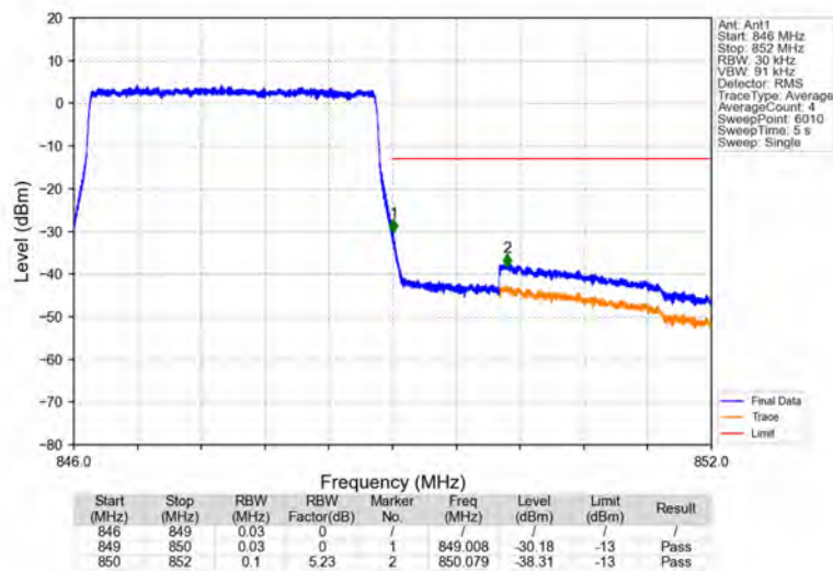
Band5_3MHz_16QAM_HCH_847.5MHz_RB_15_0_NTNV
