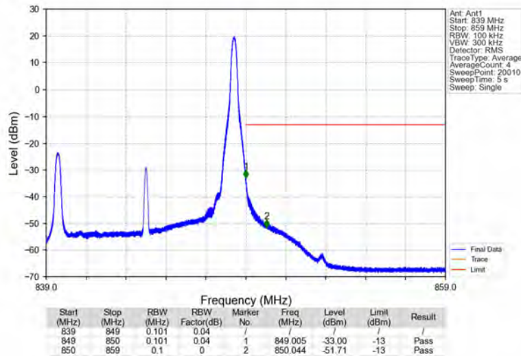
Band5_10MHz_16QAM_HCH_844MHz_RB_1_49_NTNV
