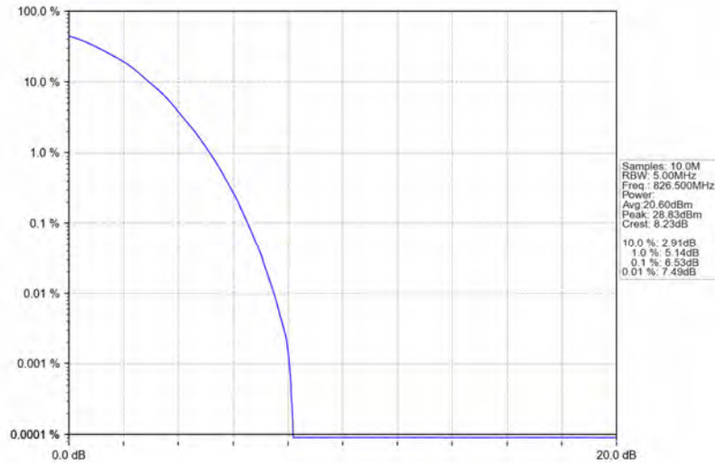
Band5_5MHz_64QAM_LCH_826.5MHz_RB_25_0_NTNV
