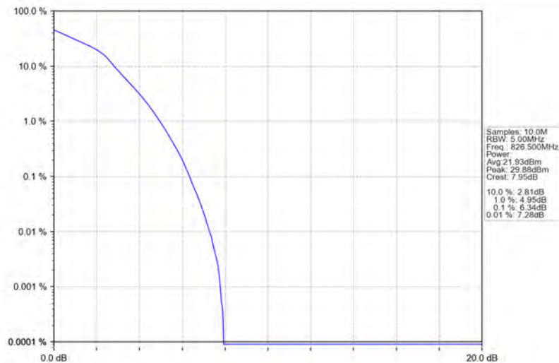
Band5_5MHz_16QAM_LCH_826.5MHz_RB_25_0_NTNV
