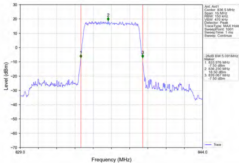
Band5_5MHz_QPSK_MCH_836.5MHz_RB_25_0_NTNV
