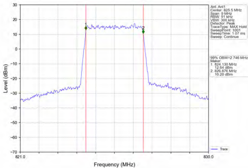
Band5_3MHz_64QAM_LCH_825.5MHz_RB_15_0_NTNV
