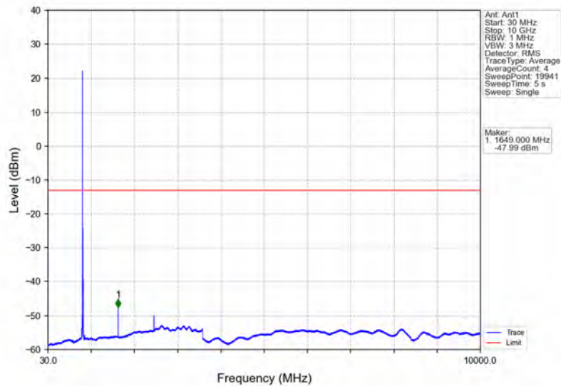
Band5_10MHz_16QAM_LCH_829MHz_RB_50_0_NTNV
