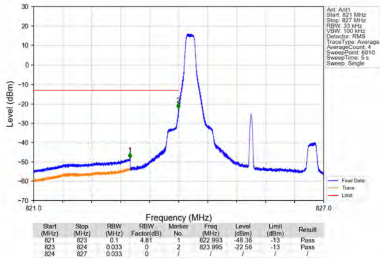
Band5_3MHz_64QAM_LCH_825.5MHz_RB_1_0_NTNV
