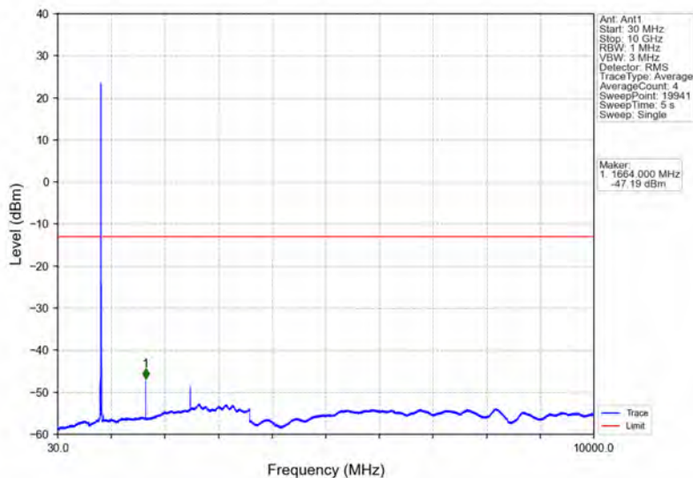
Band5_10MHz_QPSK_MCH_836.5MHz_RB_1_0_NTNV
