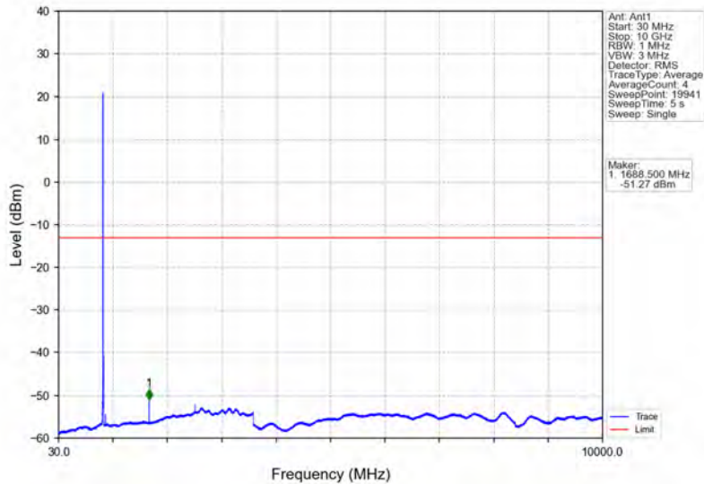
Band5_5MHz_64QAM_HCH_846.5MHz_RB_1_24_NTNV
