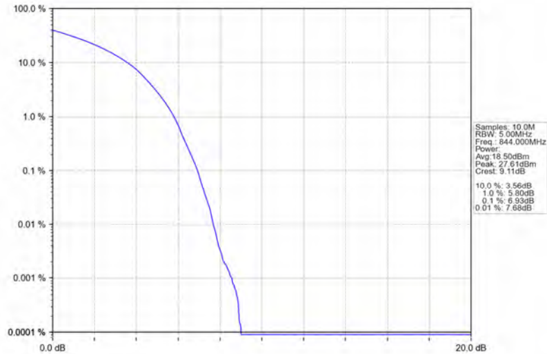
Band5_10MHz_64QAM_HCH_844MHz_RB_50_0_NTNV
