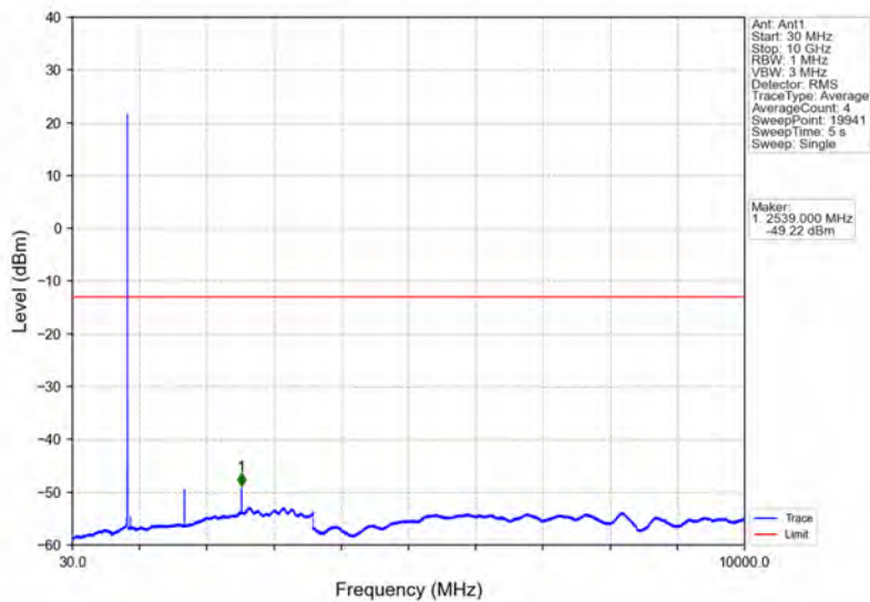
Band5_3MHz_16QAM_HCH_847.5MHz_RB_1_0_NTNV
