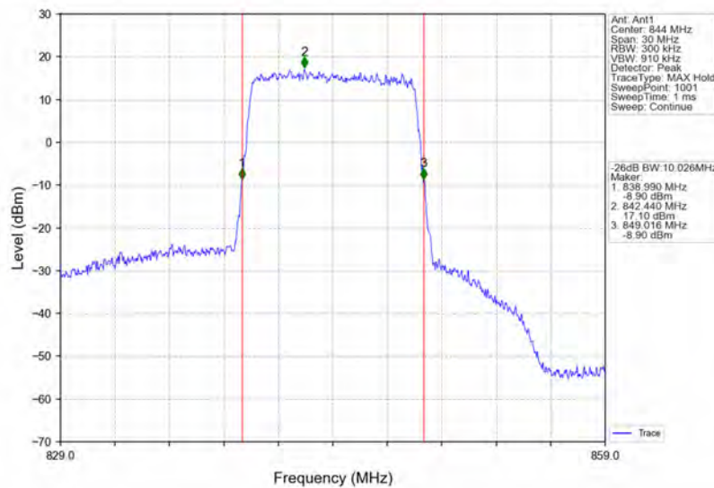
Band5_10MHz_64QAM_HCH_844MHz_RB_50_0_NTNV
