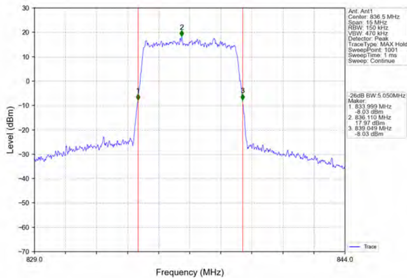
Band5_5MHz_64QAM_MCH_836.5MHz_RB_25_0_NTNV
