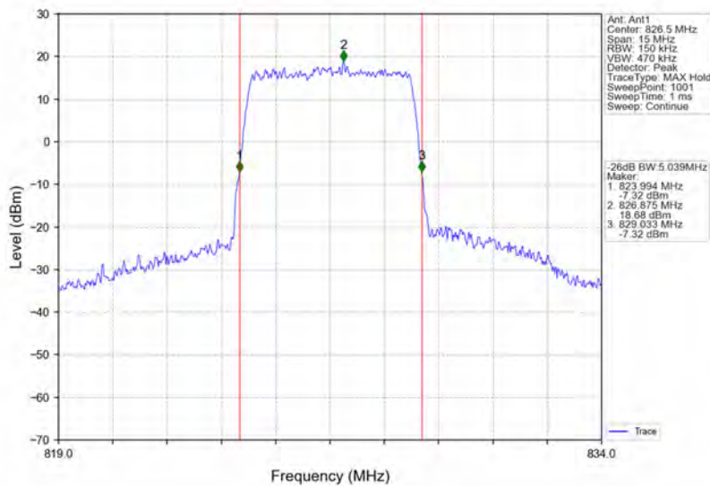
Band5_5MHz_16QAM_LCH_826.5MHz_RB_25_0_NTNV
