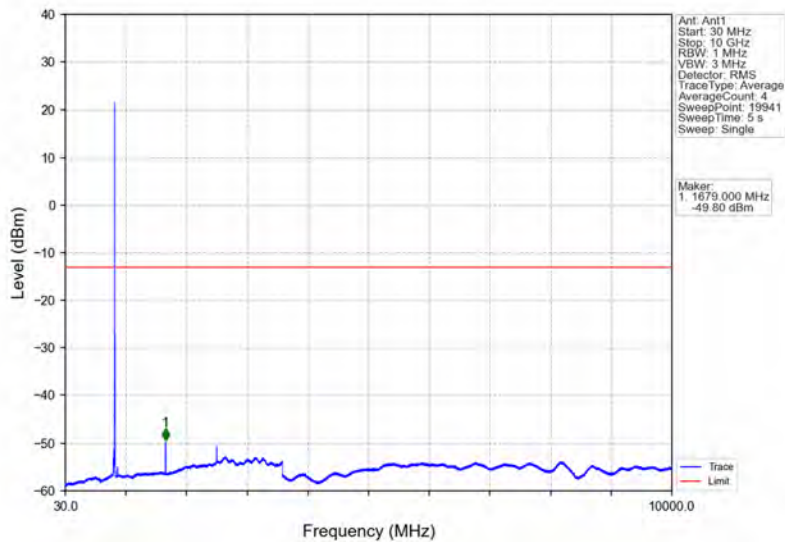
Band5_10MHz_64QAM_HCH_844MHz_RB_1_49_NTNV
