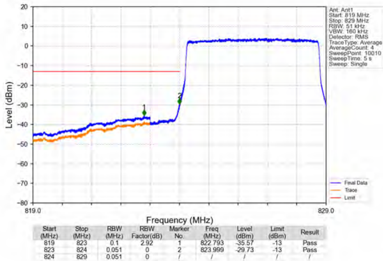
Band5_5MHz_16QAM_LCH_826.5MHz_RB_25_0_NTNV
