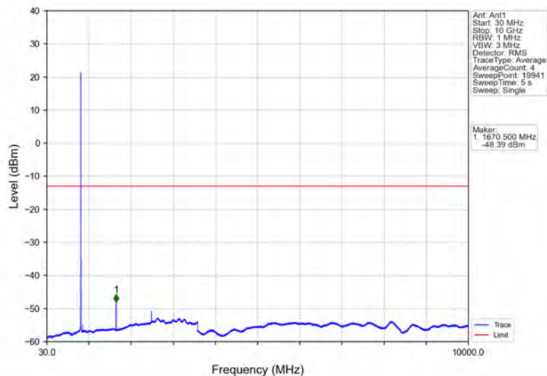
Band5_3MHz_64QAM_MCH_836.5MHz_RB_1_0_NTNV
