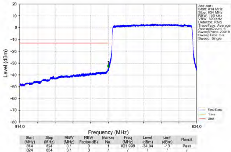
Band5_10MHz_64QAM_LCH_829MHz_RB_50_0_NTNV
