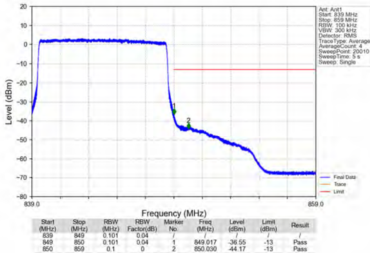
Band5_10MHz_64QAM_HCH_844MHz_RB_50_0_NTNV
