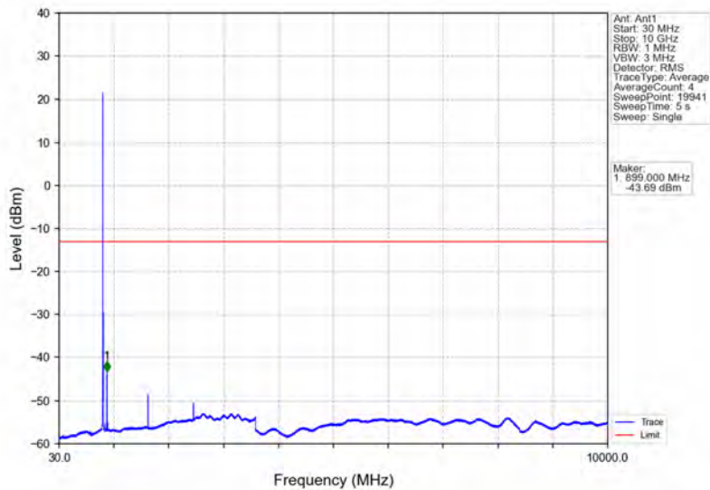
Band5_5MHz_16QAM_LCH_826.5MHz_RB_25_0_NTNV
