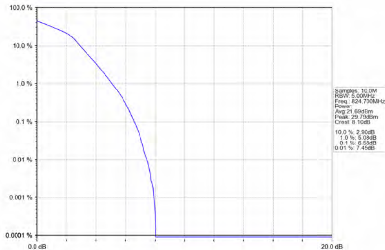
Band5_1.4MHz_16QAM_LCH_824.7MHz_RB_6_0_NTNV
