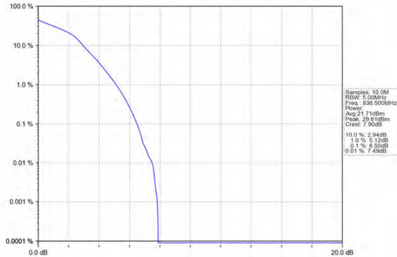
Band5_1.4MHz_16QAM_MCH_836.5MHz_RB_6_0_NTNV
