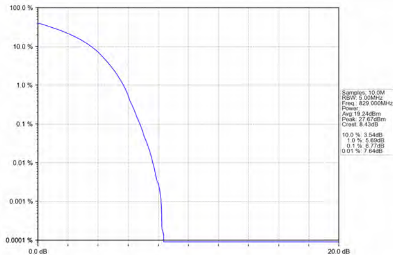
Band5_10MHz_16QAM_LCH_829MHz_RB_50_0_NTNV
