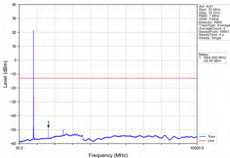
Band5_10MHz_64QAM_MCH_836.5MHz_RB_1_0_NTNV
