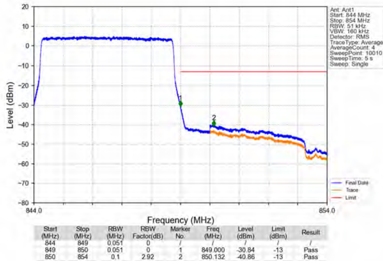
Band5_5MHz_QPSK_HCH_846.5MHz_RB_25_0_NTNV
