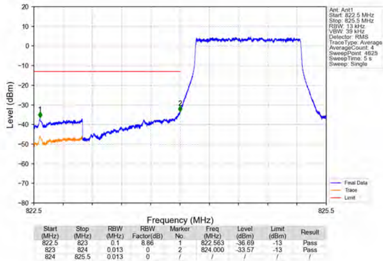
Band5_1.4MHz_16QAM_LCH_824.7MHz_RB_6_0_NTNV
