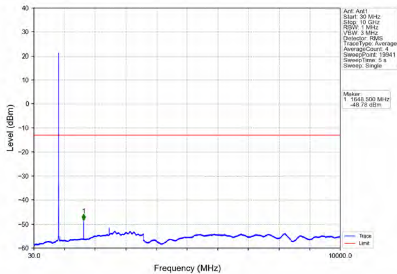
Band5_3MHz_64QAM_LCH_825.5MHz_RB_1_0_NTNV
