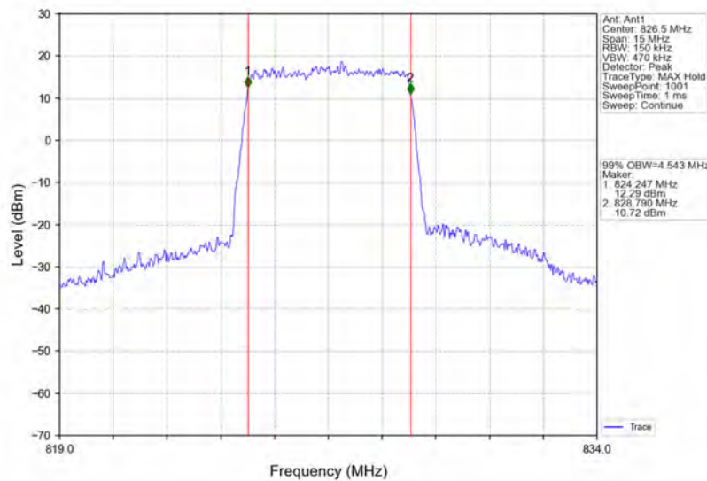
Band5_5MHz_16QAM_LCH_826.5MHz_RB_25_0_NTNV
