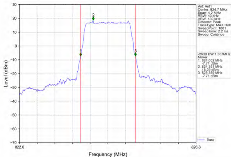
Band5_1.4MHz_16QAM_LCH_824.7MHz_RB_6_0_NTNV
