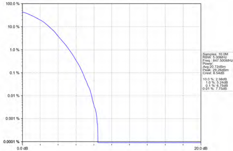
Band5_3MHz_64QAM_HCH_847.5MHz_RB_15_0_NTNV
