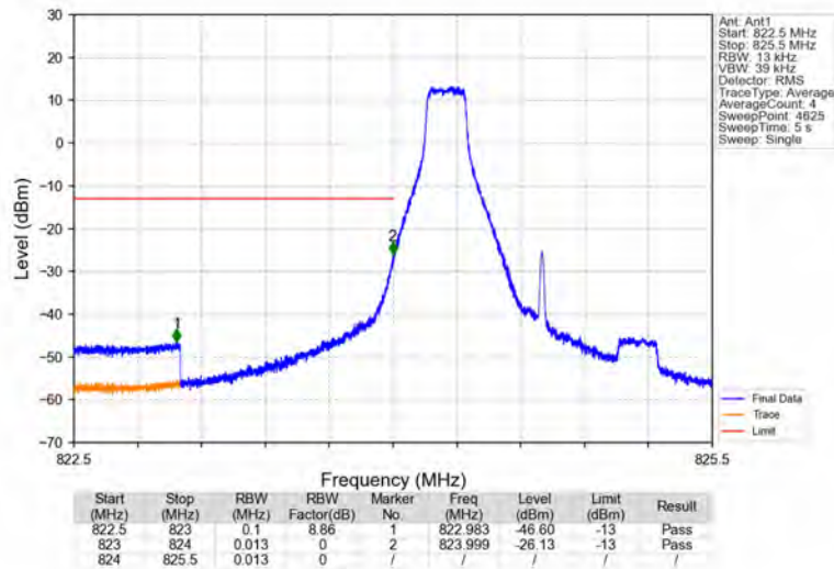
Band5_1.4MHz_16QAM_LCH_824.7MHz_RB_1_0_NTNV
