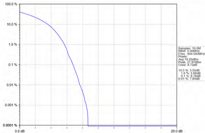
Band5_10MHz_16QAM_HCH_844MHz_RB_50_0_NTNV
