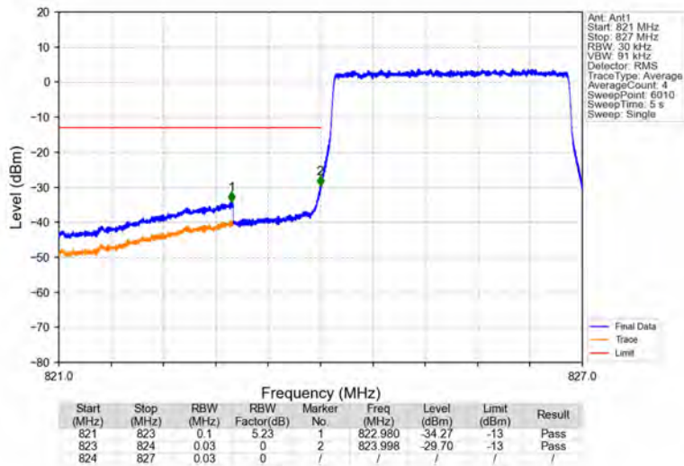
Band5_3MHz_16QAM_LCH_825.5MHz_RB_15_0_NTNV
