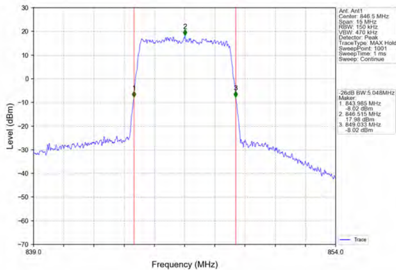
Band5_5MHz_16QAM_HCH_846.5MHz_RB_25_0_NTNV
