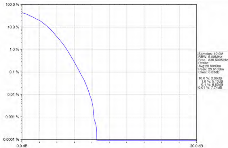
Band5_3MHz_64QAM_MCH_836.5MHz_RB_15_0_NTNV
