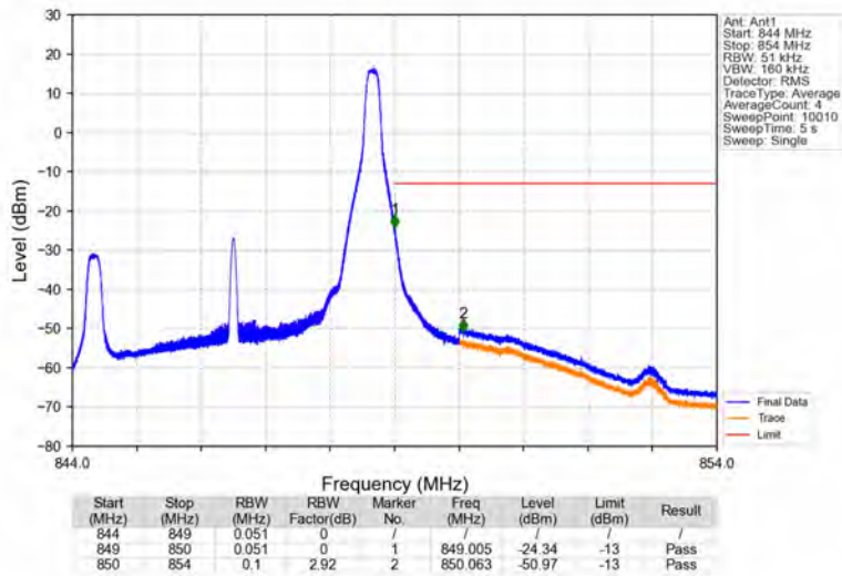
Band5_5MHz_64QAM_HCH_846.5MHz_RB_1_24_NTNV
