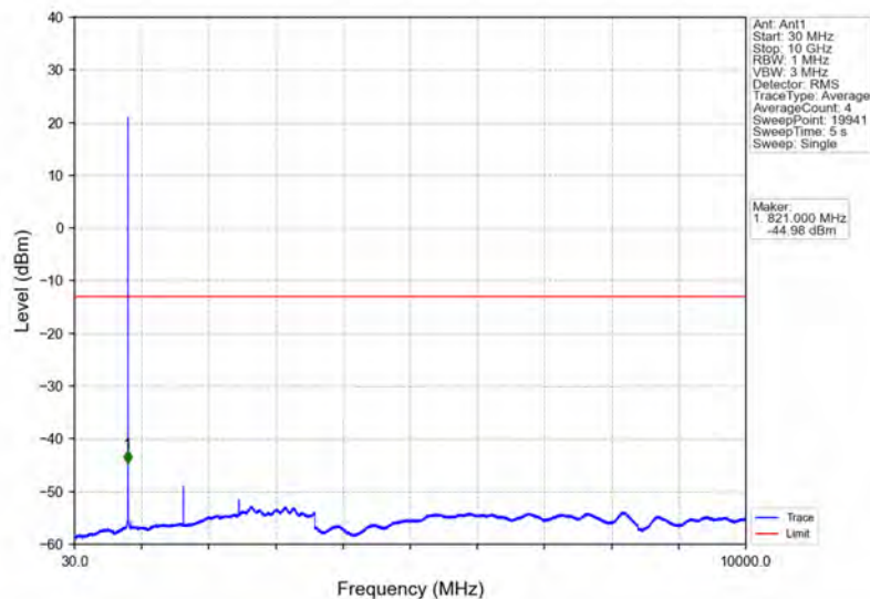
Band5_1.4MHz_64QAM_LCH_824.7MHz_RB_1_0_NTNV
