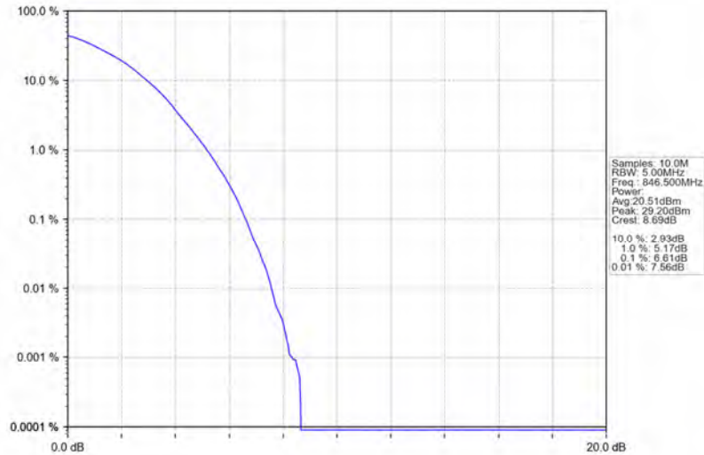
Band5_5MHz_64QAM_HCH_846.5MHz_RB_25_0_NTNV
