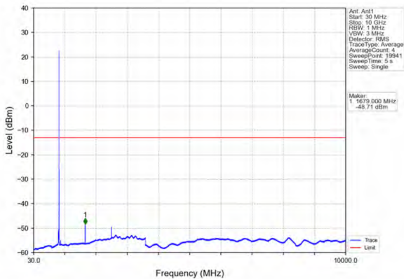
Band5_10MHz_16QAM_HCH_844MHz_RB_1_0_NTNV
