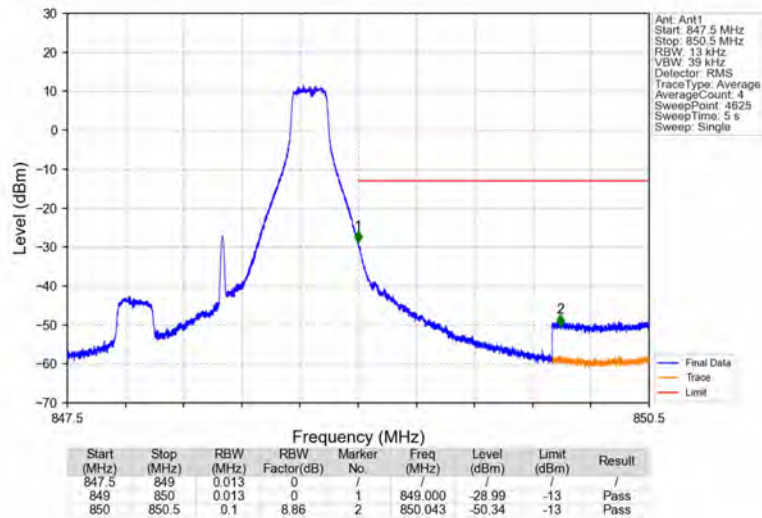
Band5_1.4MHz_64QAM_HCH_848.3MHz_RB_1_5_NTNV
