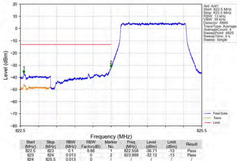
Band5_1.4MHz_QPSK_LCH_824.7MHz_RB_6_0_NTNV
