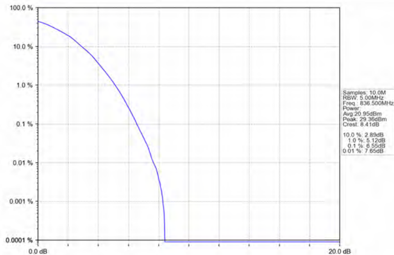
Band5_5MHz_64QAM_MCH_836.5MHz_RB_25_0_NTNV
