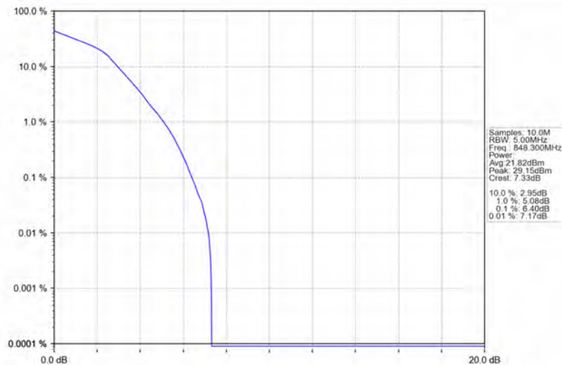
Band5_1.4MHz_16QAM_HCH_848.3MHz_RB_6_0_NTNV
