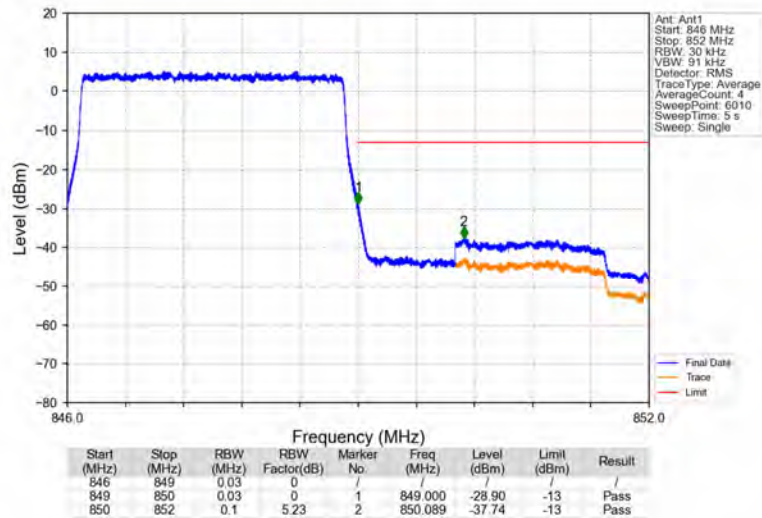
Band5_3MHz_QPSK_HCH_847.5MHz_RB_15_0_NTNV
