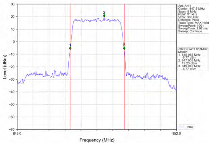
Band5_3MHz_QPSK_HCH_847.5MHz_RB_15_0_NTNV
