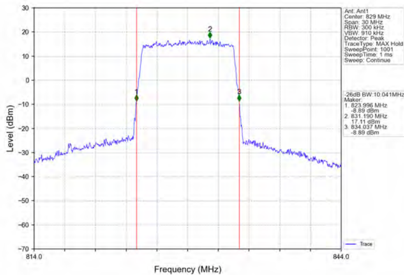
Band5_10MHz_64QAM_LCH_829MHz_RB_50_0_NTNV
