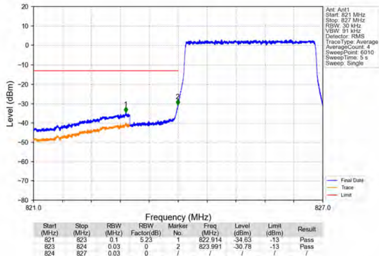
Band5_3MHz_64QAM_LCH_825.5MHz_RB_15_0_NTNV
