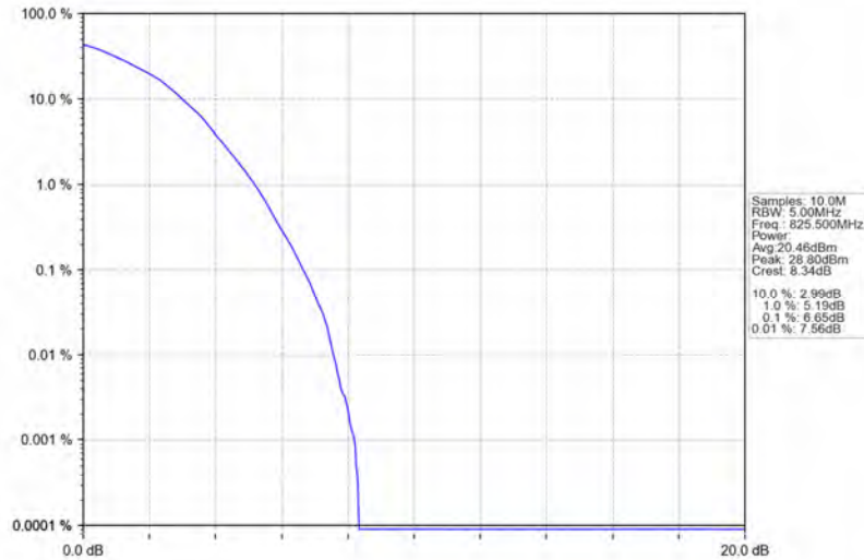
Band5_3MHz_64QAM_LCH_825.5MHz_RB_15_0_NTNV
