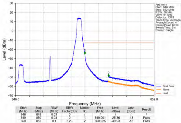
Band5_3MHz_64QAM_HCH_847.5MHz_RB_1_14_NTNV
