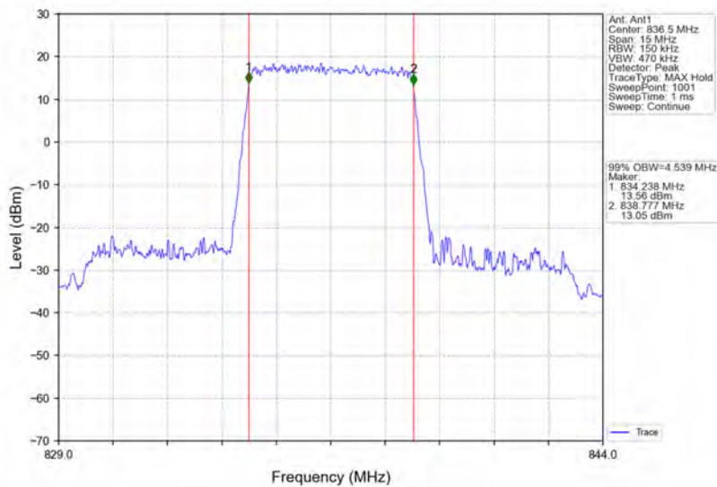
Band5_5MHz_QPSK_MCH_836.5MHz_RB_25_0_NTNV
