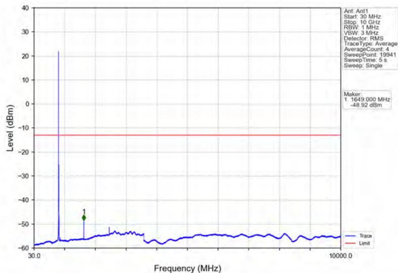
Band5_10MHz_64QAM_LCH_829MHz_RB_1_0_NTNV
