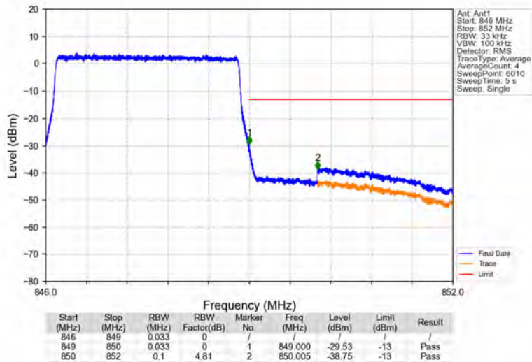
Band5_3MHz_64QAM_HCH_847.5MHz_RB_15_0_NTNV
