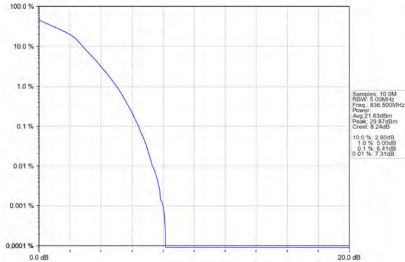
Band5_5MHz_16QAM_MCH_836.5MHz_RB_25_0_NTNV
