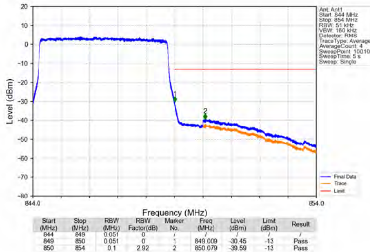
Band5_5MHz_16QAM_HCH_846.5MHz_RB_25_0_NTNV
