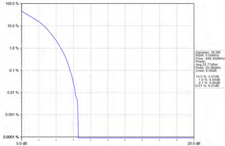
Band5_1.4MHz_QPSK_HCH_848.3MHz_RB_6_0_NTNV
