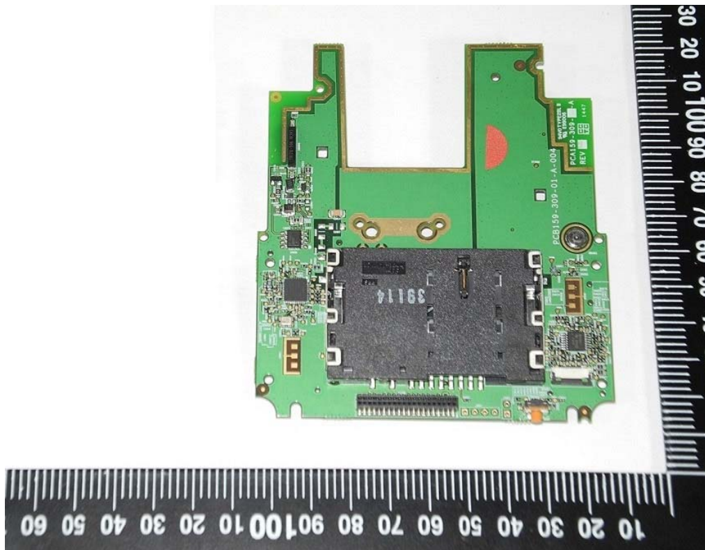
RF IC: PN512
